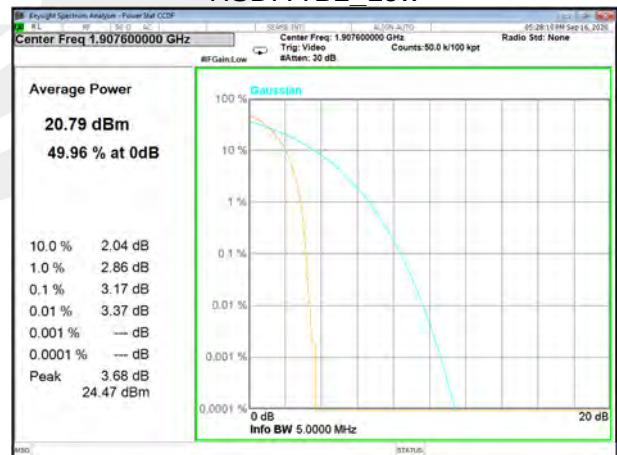
HSDPA B2_High
