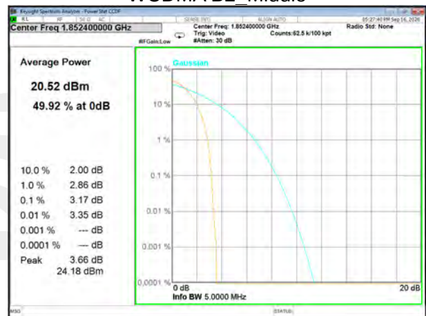
HSDPA B2_Low
