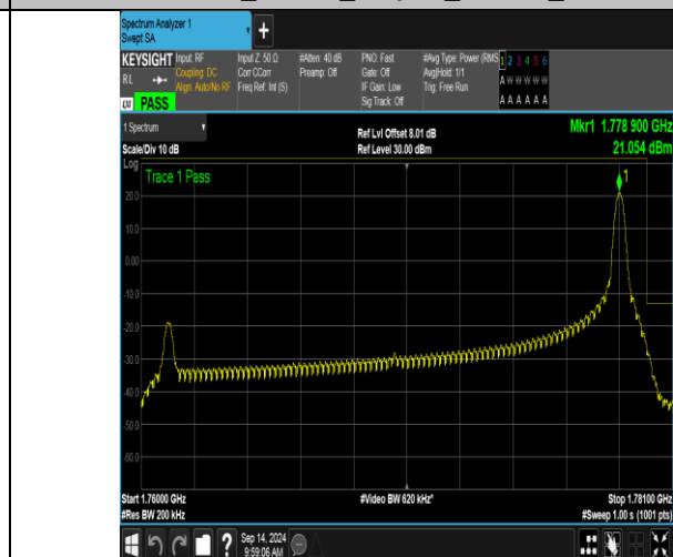
Band66_20MHz_16QAM_132572_1RB#99
