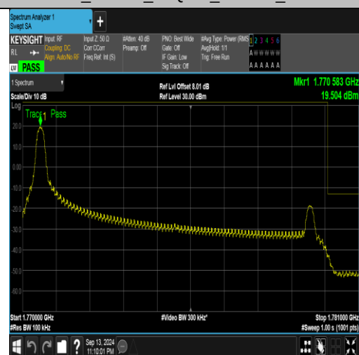
Band66_10MHz_16QAM_132622_1RB#0
