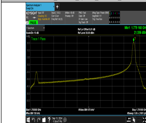
Band66_15MHz_QPSK_132597_1RB#74
