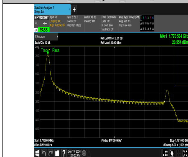
Band66_10MHz_QPSK_132622_1RB#0
