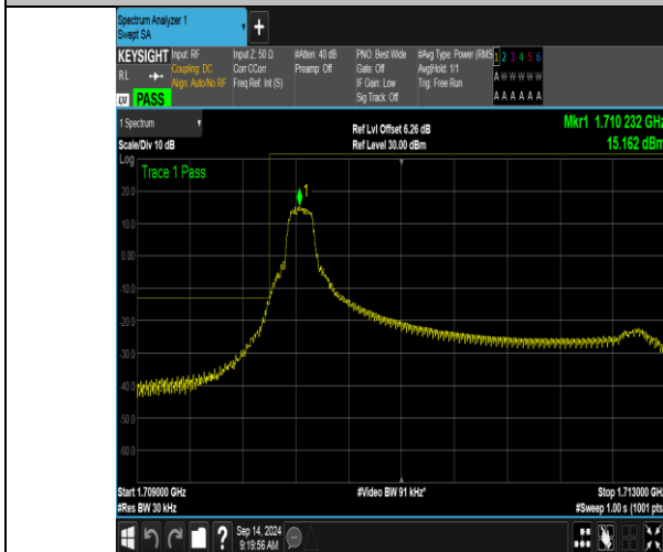
Band66_3MHz_QPSK_131987_1RB#0
