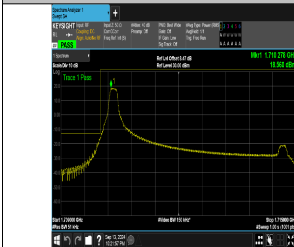
Band66_5MHz_QPSK_131997_1RB#0
