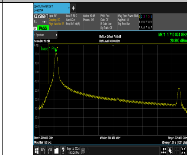
Band66_15MHz_16QAM_132047_1RB#0
