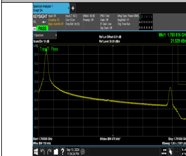
Band66_15MHz_QPSK_132597_1RB#0
