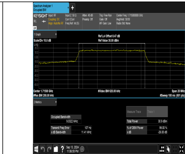
Band66-10MHz-16QAM-132022-50RB#0-PASS
