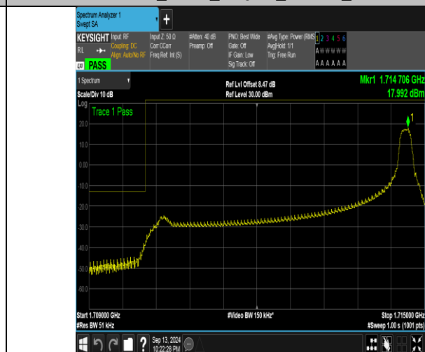
Band66_5MHz_16QAM_131997_1RB#24
