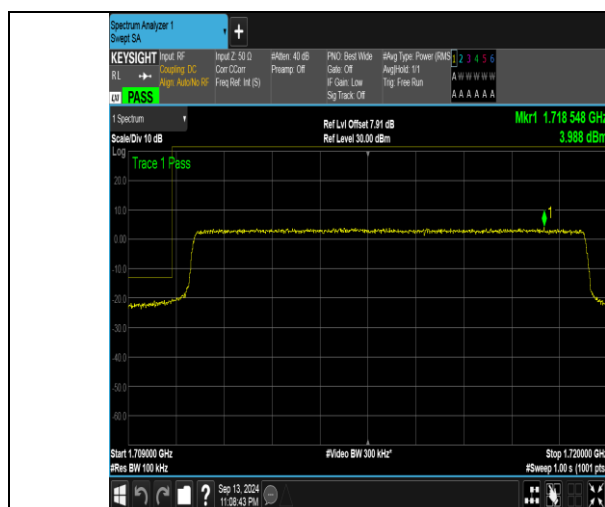
Band66_10MHz_QPSK_132022_50RB#0
