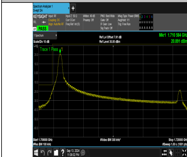
Band66_10MHz_QPSK_132022_1RB#0
