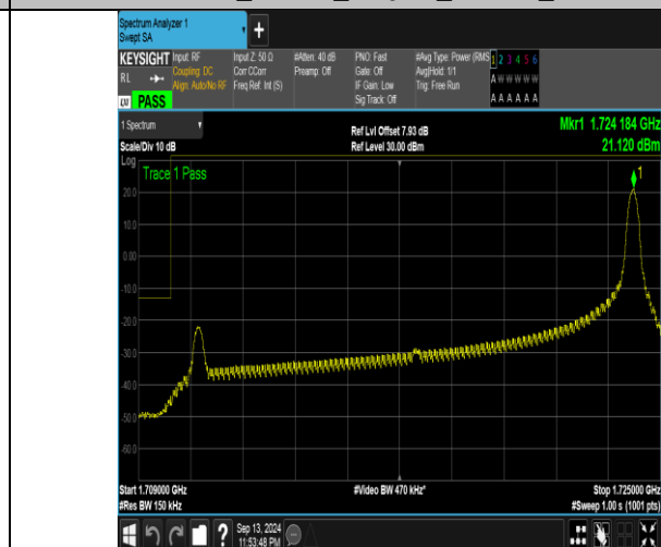
Band66_15MHz_16QAM_132047_1RB#74
