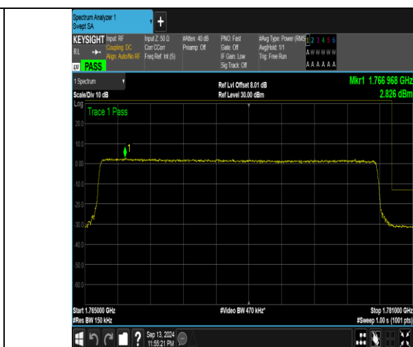
Band66_15MHz_16QAM_132597_75RB#0
