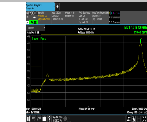
Band66_10MHz_16QAM_132022_1RB#49
