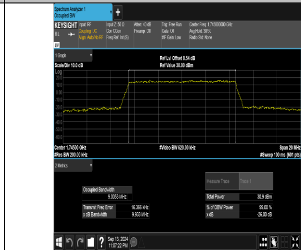
Band66-10MHz-16QAM-132322-50RB#0-PASS
