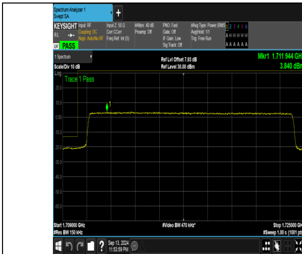
Band66_15MHz_QPSK_132047_75RB#0
