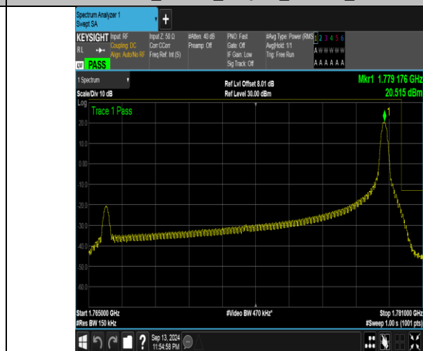
Band66_15MHz_16QAM_132597_1RB#74
