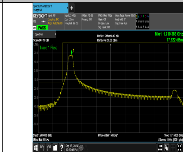
Band66_5MHz_16QAM_131997_1RB#0
