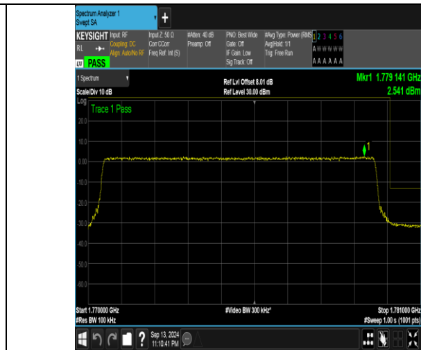
Band66_10MHz_16QAM_132622_50RB#0
