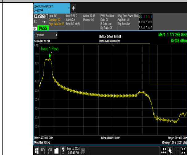
Band66_3MHz_16QAM_132657_1RB#0
