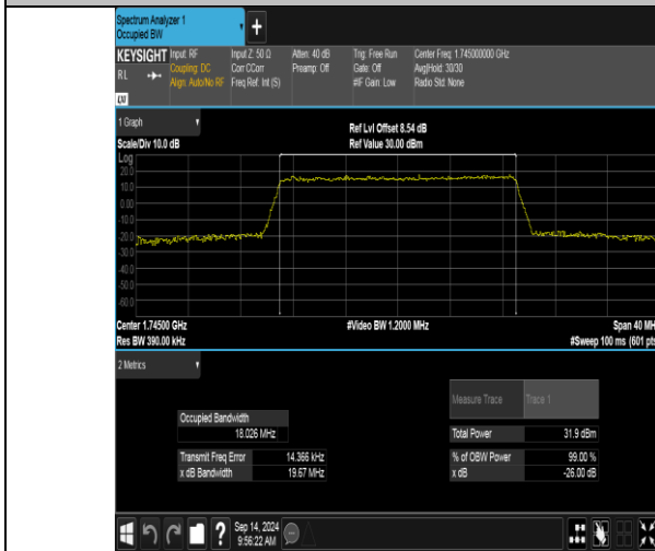
Band66-20MHz-QPSK-132322-100RB#0-PASS
