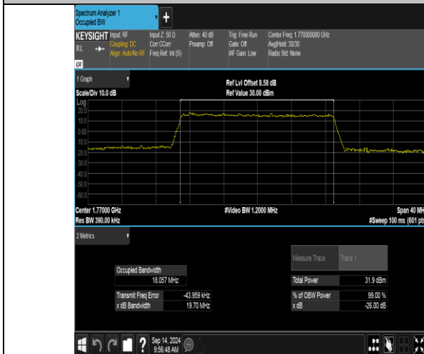
Band66-20MHz-QPSK-132572-100RB#0-PASS
