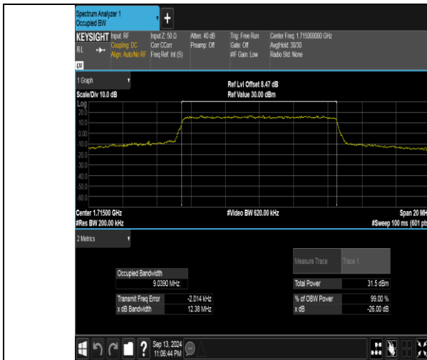
Band66-10MHz-QPSK-132022-50RB#0-PASS
