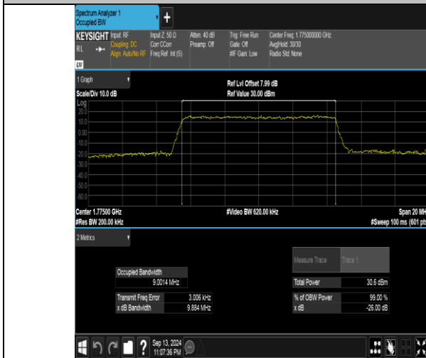
Band66-10MHz-QPSK-132622-50RB#0-PASS
