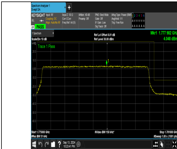
Band66_5MHz_QPSK_132647_25RB#0
