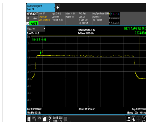
Band66_15MHz_QPSK_132597_75RB#0
