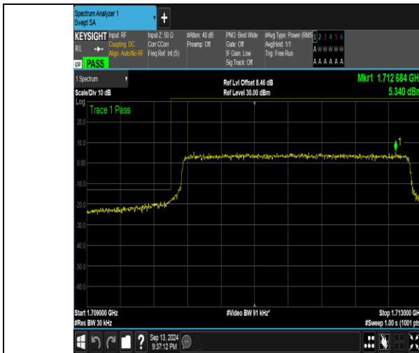
Band66_3MHz_QPSK_131987_15RB#0
