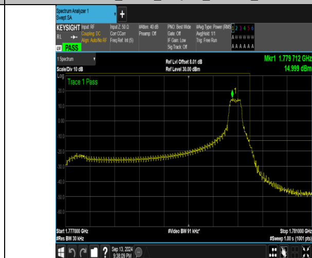
Band66_3MHz_16QAM_132657_1RB#14
