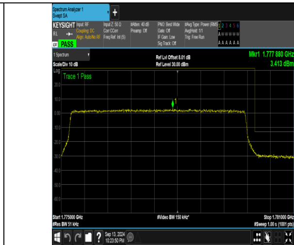
Band66_5MHz_16QAM_132647_25RB#0
