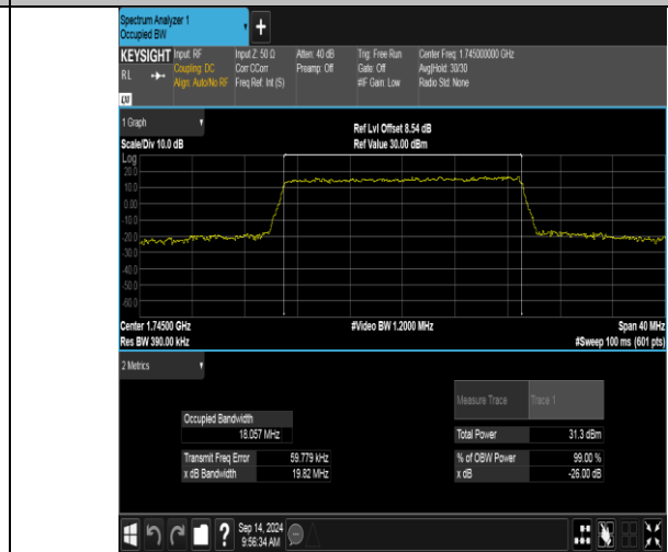
Band66-20MHz-16QAM-132322-100RB#0-PASS
