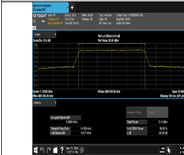
Band66-10MHz-QPSK-132322-50RB#0-PASS
