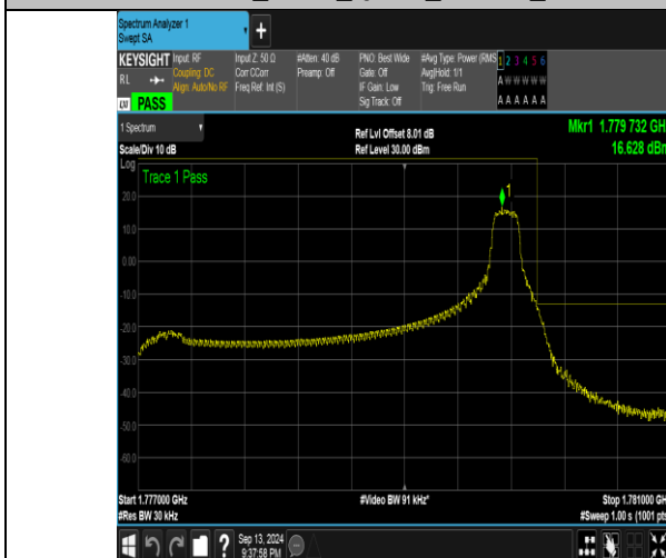
Band66_3MHz_QPSK_132657_1RB#14
