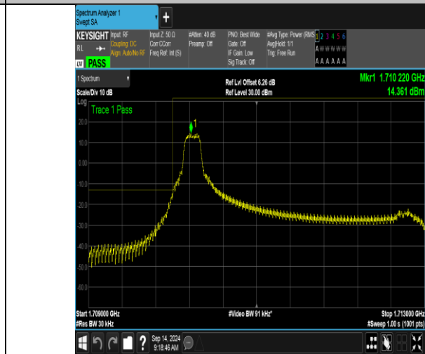
Band66_3MHz_16QAM_131987_1RB#0
