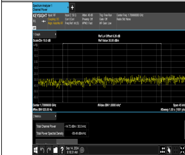
Band66_3MHz_QPSK_131987_1RB#0_Final1
