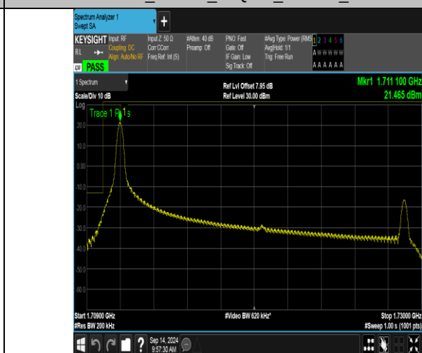
Band66_20MHz_16QAM_132072_1RB#0
