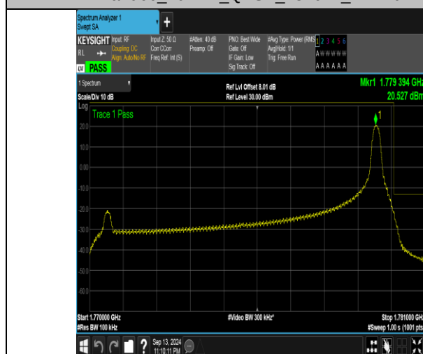
Band66_10MHz_QPSK_132622_1RB#49
