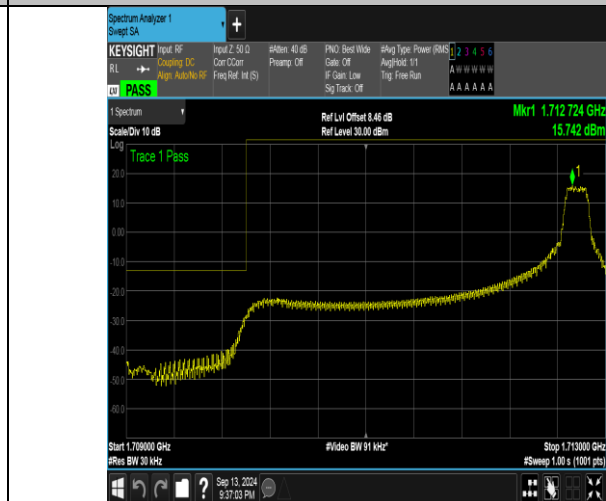
Band66_3MHz_16QAM_131987_1RB#14
