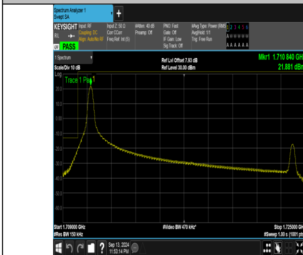
Band66_15MHz_QPSK_132047_1RB#0
