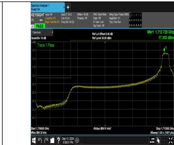
Band66_3MHz_QPSK_131987_1RB#14
