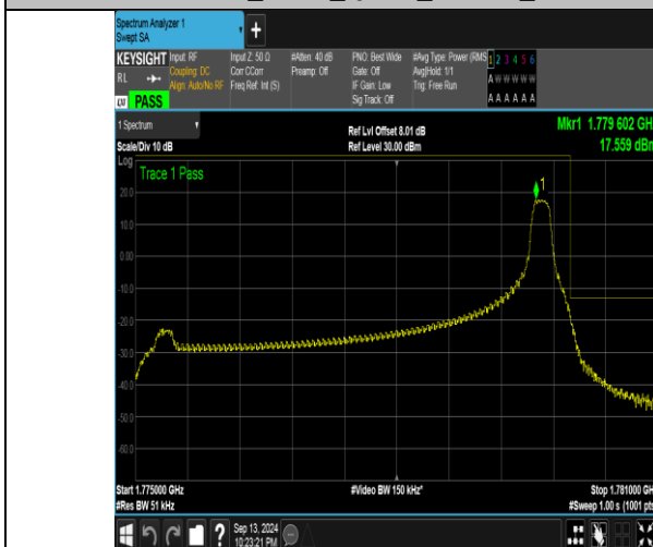
Band66_5MHz_QPSK_132647_1RB#24
