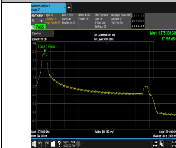
Band66_5MHz_QPSK_132647_1RB#0
