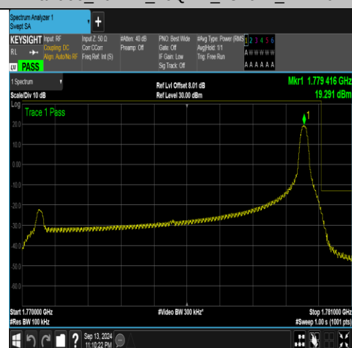
Band66_10MHz_16QAM_132622_1RB#49
