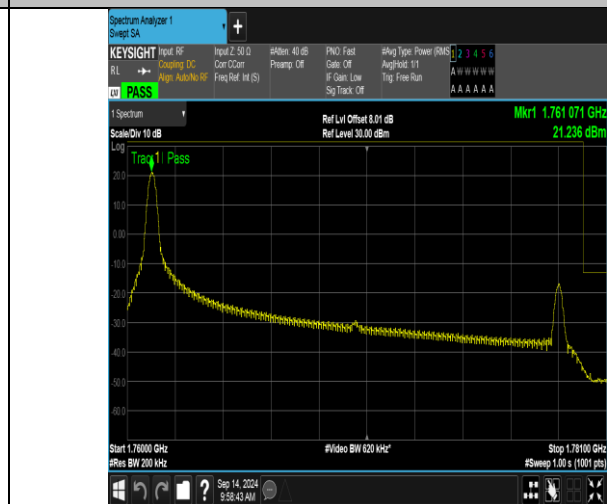
Band66_20MHz_16QAM_132572_1RB#0
