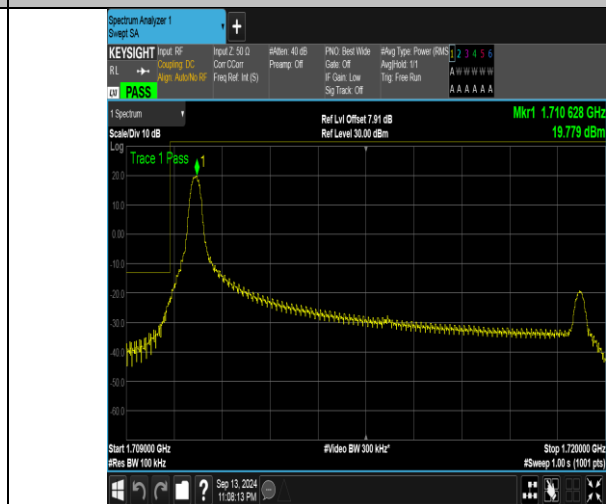
Band66_10MHz_16QAM_132022_1RB#0
