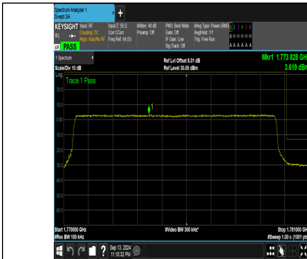
Band66_10MHz_QPSK_132622_50RB#0
