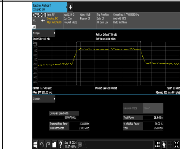
Band66-10MHz-16QAM-132622-50RB#0-PASS
