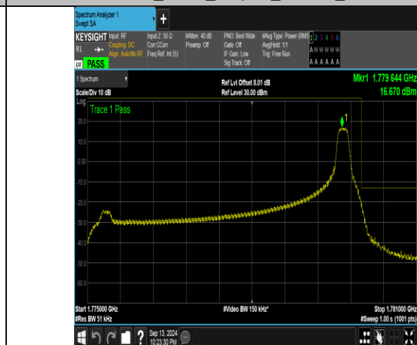
Band66_5MHz_16QAM_132647_1RB#24
