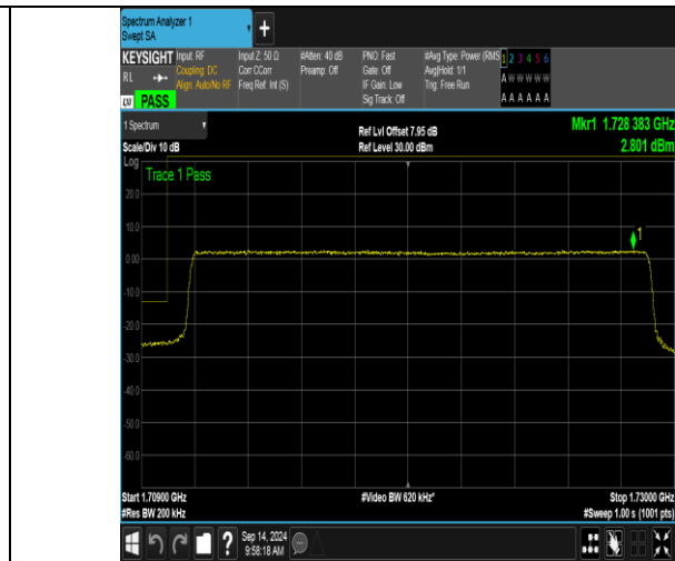
Band66_20MHz_16QAM_132072_100RB#0
