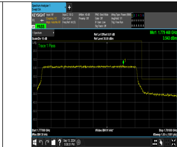
Band66_3MHz_16QAM_132657_15RB#0
