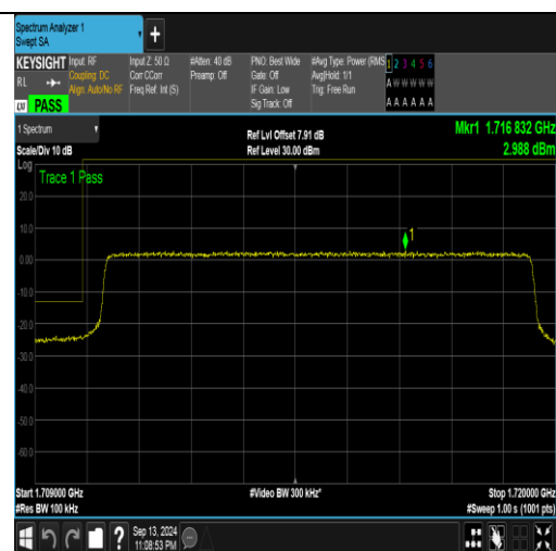
Band66_10MHz_16QAM_132022_50RB#0
