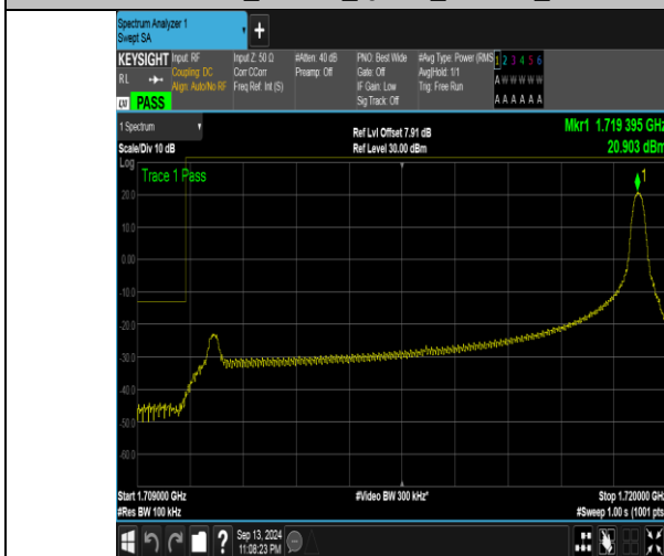
Band66_10MHz_QPSK_132022_1RB#49
