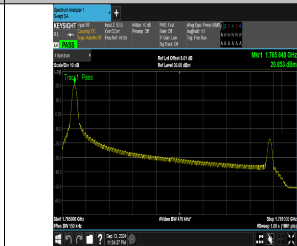
Band66_15MHz_16QAM_132597_1RB#0
