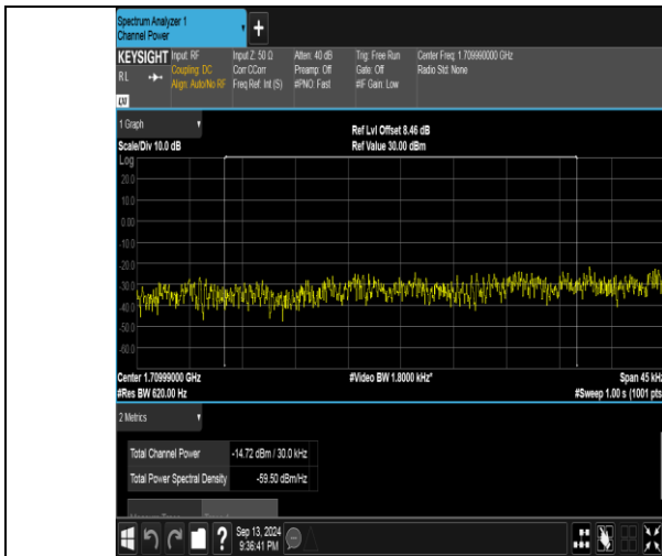
Band66_3MHz_16QAM_131987_1RB#0_Final1
