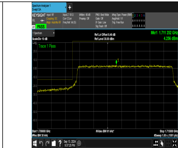
Band66_3MHz_16QAM_131987_15RB#0
