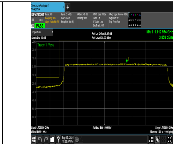
Band66_5MHz_16QAM_131997_25RB#0
