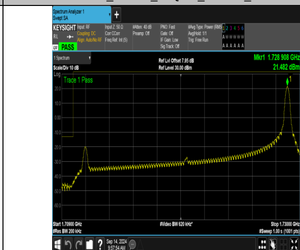
Band66_20MHz_16QAM_132072_1RB#99
