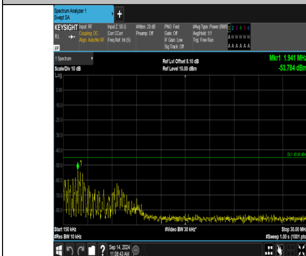
Band41_5MHz_16QAM_40065_1RB#0_0.15~30_0.15~30
