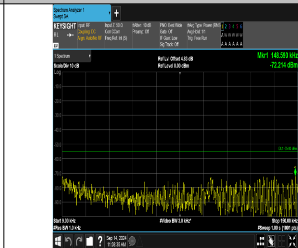
Band41_5MHz_16QAM_40065_1RB#0_0.009~0.15_0.009~0.15
