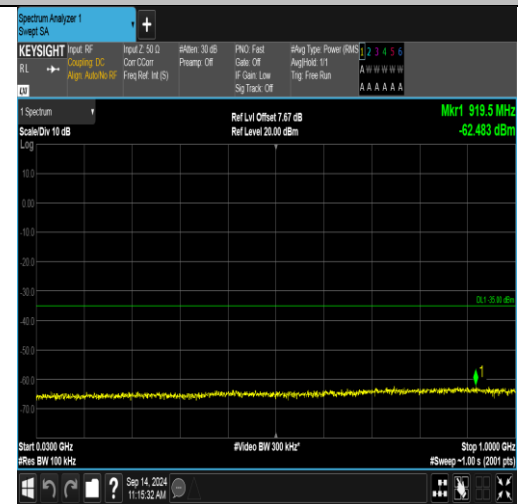
Band41_5MHz_16QAM_40590_1RB#24_30~1000_30~1000
