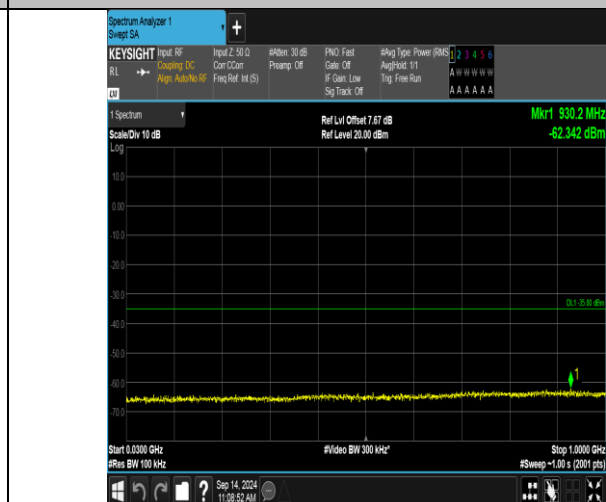
Band41_5MHz_16QAM_40065_1RB#0_30~1000_30~1000
