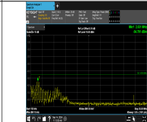
Band41_5MHz_QPSK_40590_1RB#0_0.15~30_0.15~30
