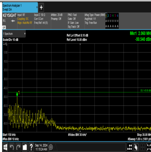
Band41_5MHz_16QAM_40590_1RB#24_0.15~30_0.15~30
