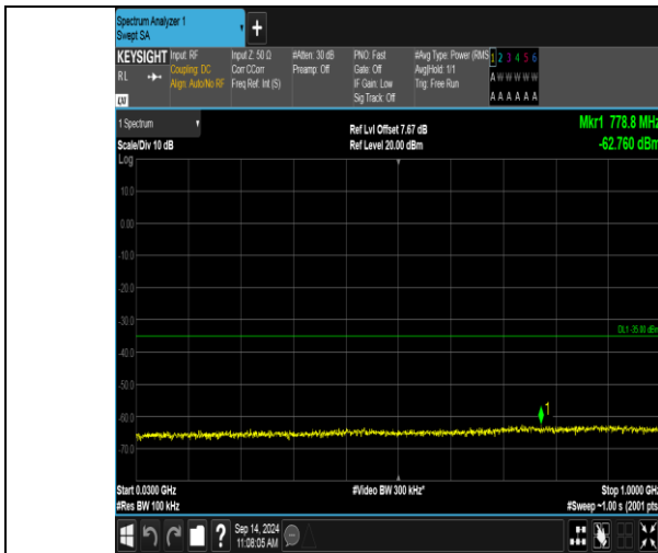
Band41_5MHz_QPSK_40065_1RB#0_30~1000_30~1000
