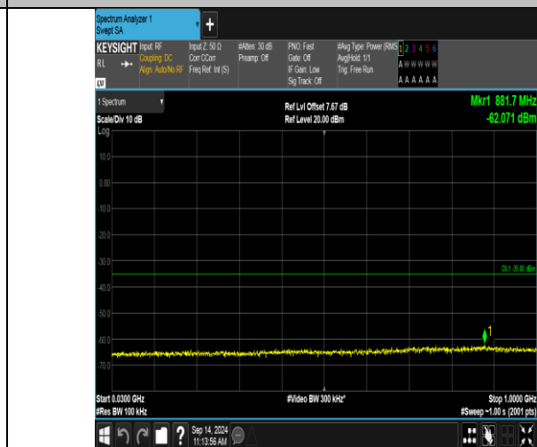
Band41_5MHz_16QAM_40590_1RB#0_30~1000_30~1000
