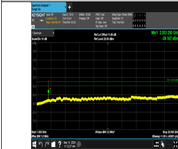
Band41_5MHz_16QAM_40065_25RB#0_1000~20000_1000~20000
