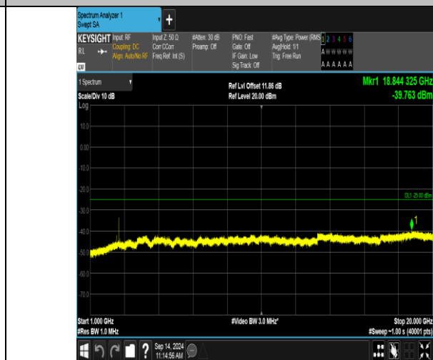
Band41_5MHz_QPSK_40590_1RB#24_1000~20000_1000~20000
