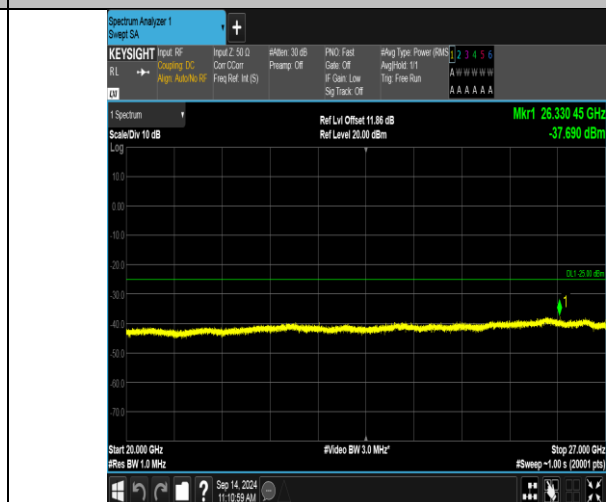
Band41_5MHz_16QAM_40065_1RB#24_20000~27000_20000~27000
