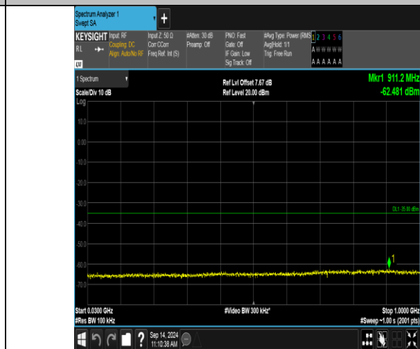
Band41_5MHz_16QAM_40065_1RB#24_30~1000_30~1000
