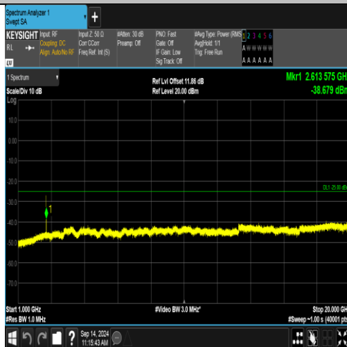
Band41_5MHz_16QAM_40590_1RB#24_1000~20000_1000~20000
