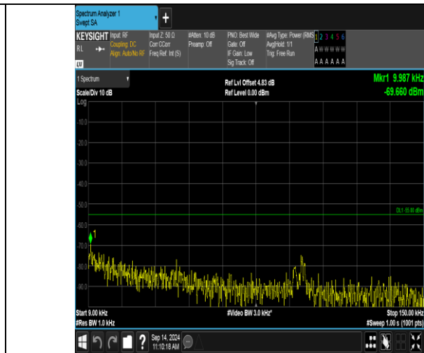
Band41_5MHz_16QAM_40065_1RB#24_0.009~0.15_0.009~0.15
