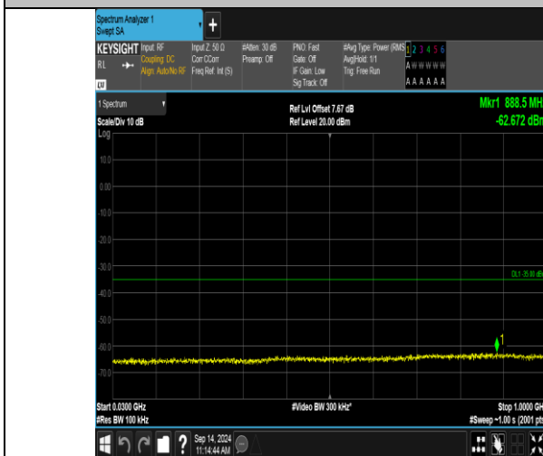
Band41_5MHz_QPSK_40590_1RB#24_30~1000_30~1000
