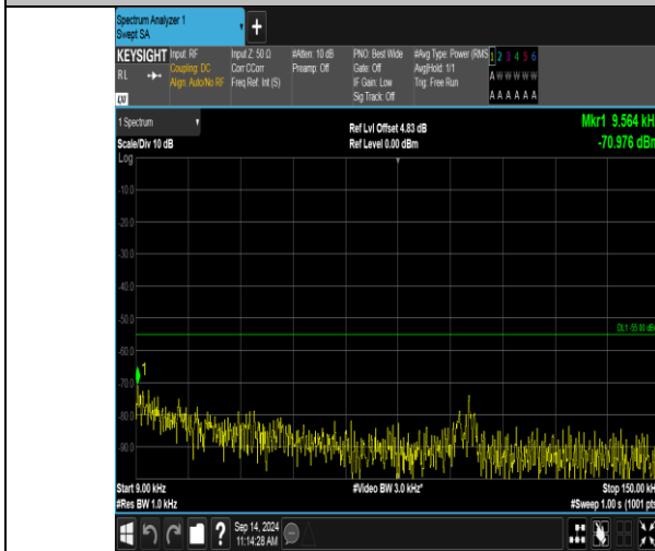
Band41_5MHz_QPSK_40590_1RB#24_0.009~0.15_0.009~0.15
