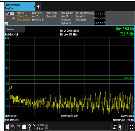
Band41_5MHz_16QAM_40590_1RB#24_0.009~0.15_0.009~0.15
