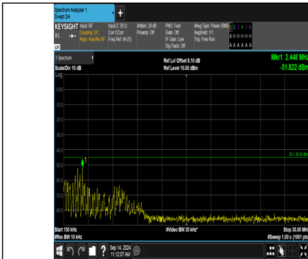
Band41_5MHz_16QAM_40065_25RB#0_0.15~30_0.15~30
