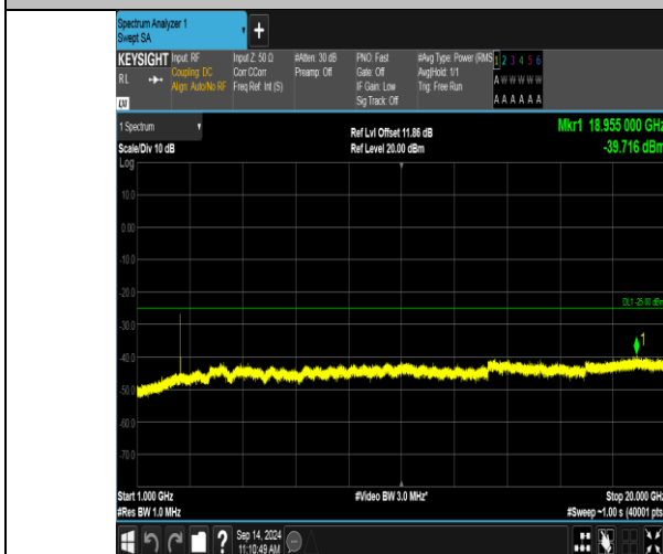
Band41_5MHz_16QAM_40065_1RB#24_1000~20000_1000~20000
