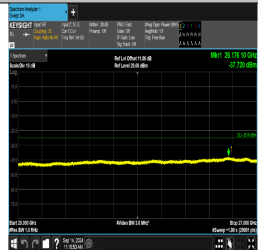
Band41_5MHz_16QAM_40590_1RB#24_20000~27000_20000~27000
