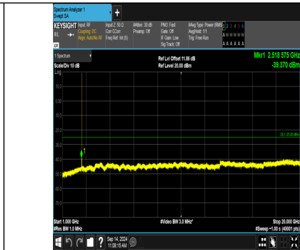
Band41_5MHz_QPSK_40065_1RB#0_1000~20000_1000~20000
