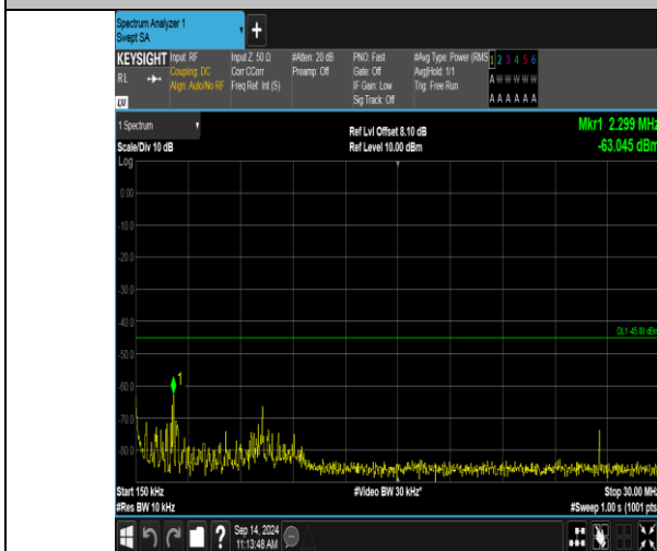
Band41_5MHz_16QAM_40590_1RB#0_0.15~30_0.15~30
