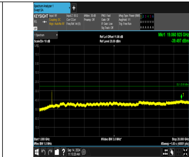
Band41_5MHz_QPSK_40590_1RB#0_1000~20000_1000~20000
