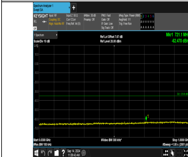
Band41_5MHz_QPSK_40065_1RB#24_30~1000_30~1000
