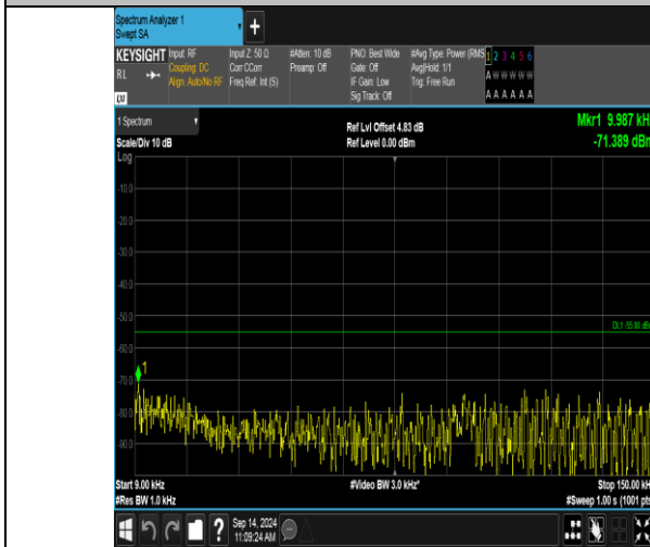
Band41_5MHz_QPSK_40065_1RB#24_0.009~0.15_0.009~0.15
