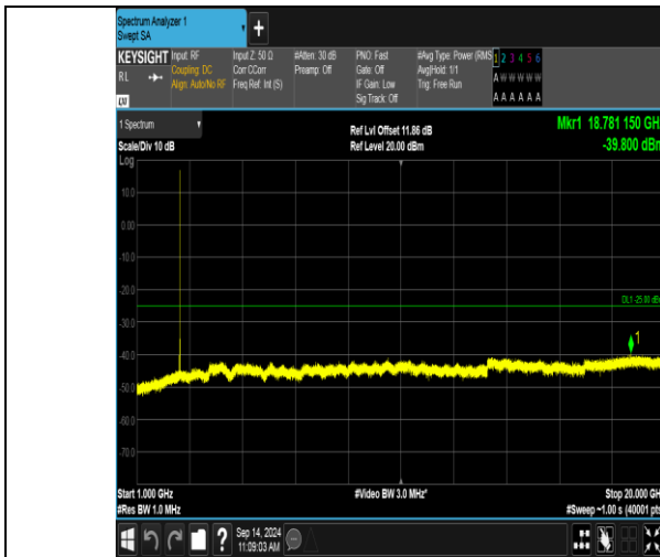
Band41_5MHz_16QAM_40065_1RB#0_1000~20000_1000~20000
