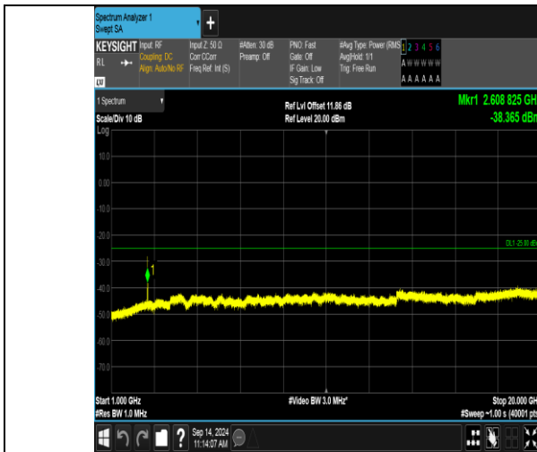
Band41_5MHz_16QAM_40590_1RB#0_1000~20000_1000~20000
