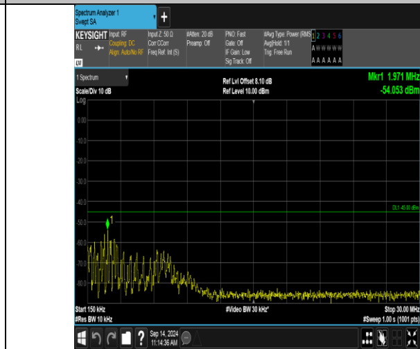
Band41_5MHz_QPSK_40590_1RB#24_0.15~30_0.15~30
