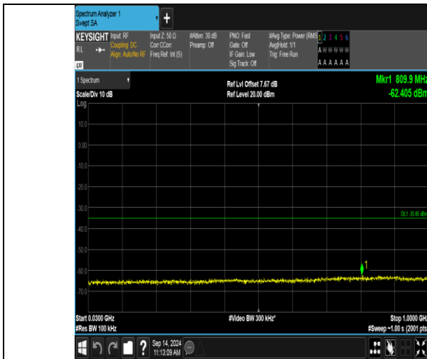
Band41_5MHz_QPSK_40590_1RB#0_30~1000_30~1000
