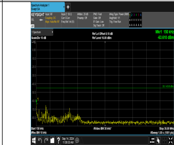
Band41_5MHz_QPSK_40065_1RB#24_0.15~30_0.15~30
