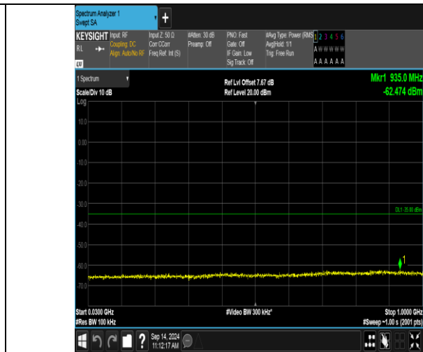
Band41_5MHz_16QAM_40065_25RB#0_30~1000_30~1000
