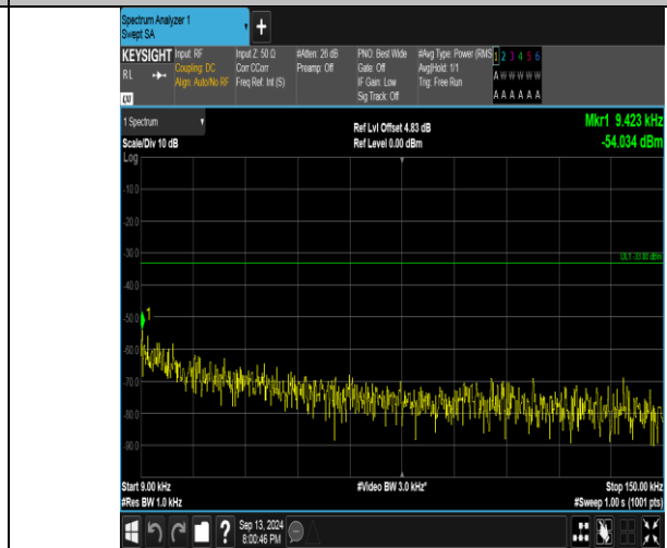
Band26_10MHz_16QAM_26990_1RB#0_0.009~0.15_0.009~0.15
