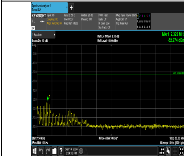
Band26_10MHz_16QAM_26990_50RB#0_0.15~30_0.15~30
