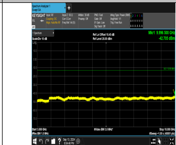
Band26_10MHz_16QAM_26990_50RB#0_3000~10000_3000~10000
