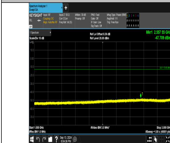
Band26_10MHz_16QAM_26990_50RB#0_1000~3000_1000~3000
