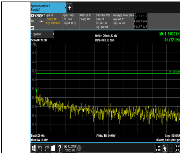
Band26_10MHz_QPSK_26990_1RB#0_0.009~0.15_0.009~0.15
