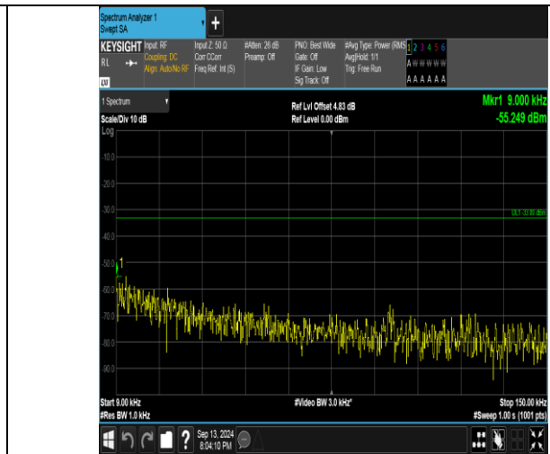
Band26_10MHz_16QAM_26990_50RB#0_0.009~0.15_0.009~0.15
