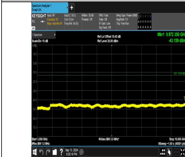
Band26_15MHz_QPSK_26865_1RB#74_3000~10000_3000~10000
