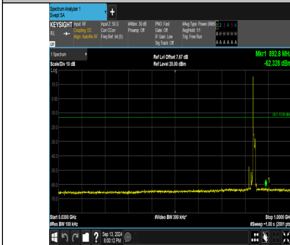
Band26_10MHz_QPSK_26990_1RB#0_30~1000_30~1000
