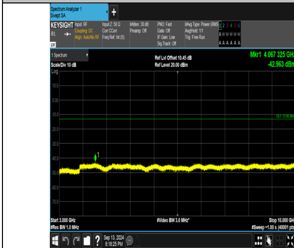
Band26_15MHz_QPSK_26865_1RB#0_3000~10000_3000~10000
