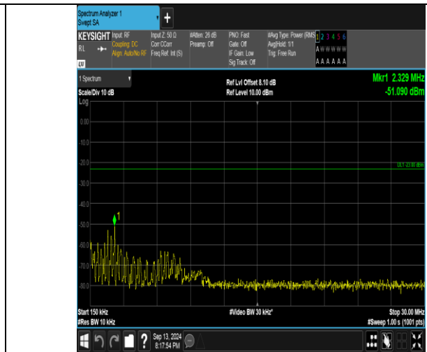
Band26_15MHz_QPSK_26865_1RB#0_0.15~30_0.15~30
