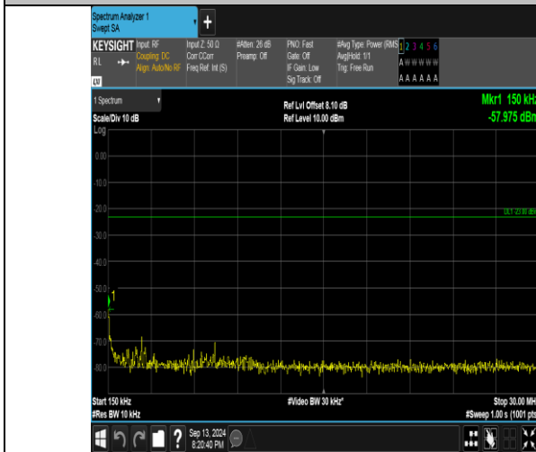
Band26_15MHz_16QAM_26865_1RB#74_0.15~30_0.15~30
