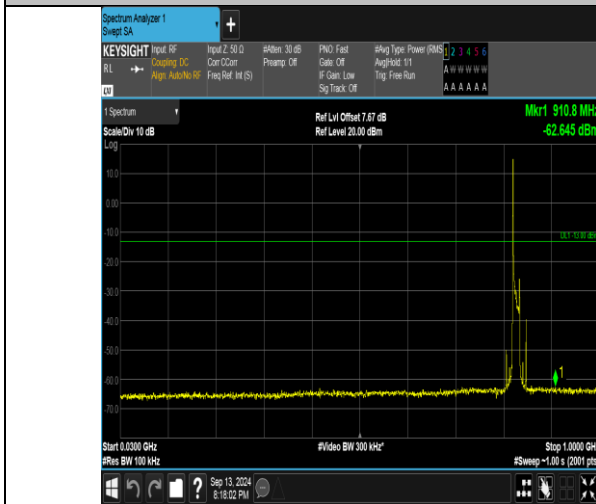
Band26_15MHz_QPSK_26865_1RB#0_30~1000_30~1000
