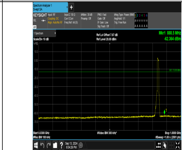
Band26_10MHz_16QAM_26990_50RB#0_30~1000_30~1000
