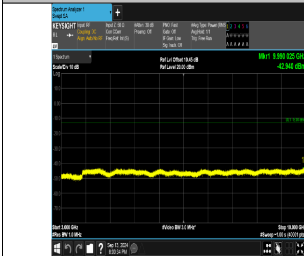
Band26_10MHz_QPSK_26990_1RB#0_3000~10000_3000~10000
