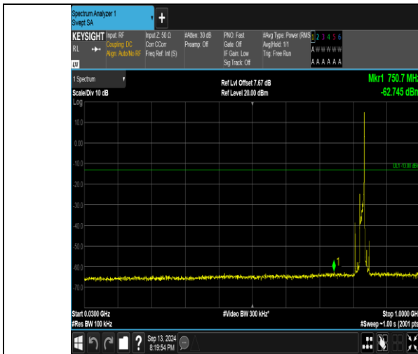
Band26_15MHz_QPSK_26865_1RB#74_30~1000_30~1000
