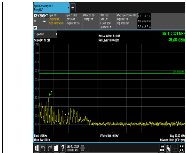
Band26_10MHz_QPSK_26990_1RB#0_0.15~30_0.15~30
