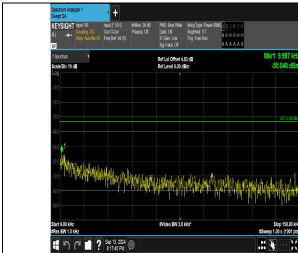
Band26_15MHz_QPSK_26865_1RB#0_0.009~0.15_0.009~0.15
