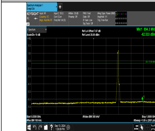
Band12_10MHz_QPSK_23060_50RB#0_30~1000_30~1000
