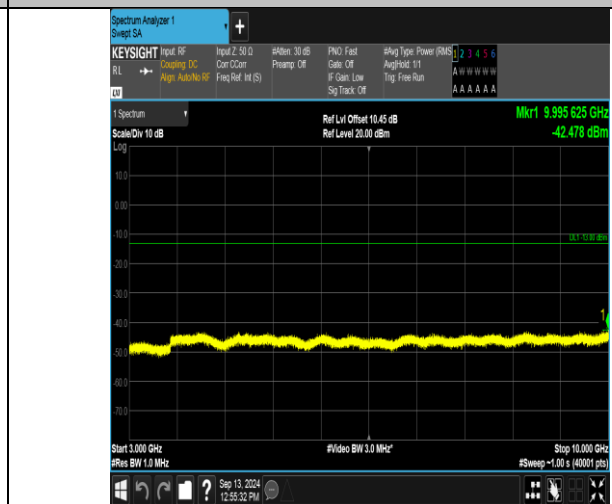
Band12_5MHz_16QAM_23155_25RB#0_3000~10000_3000~10000
