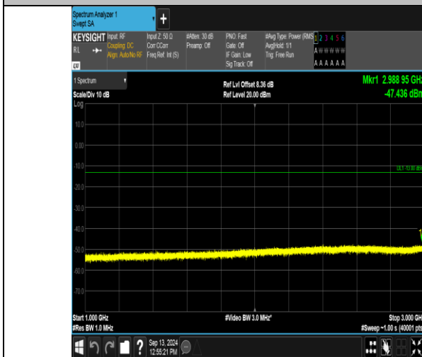
Band12_5MHz_16QAM_23155_25RB#0_1000~3000_1000~3000
