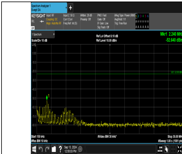
Band12_5MHz_16QAM_23155_25RB#0_0.15~30_0.15~30
