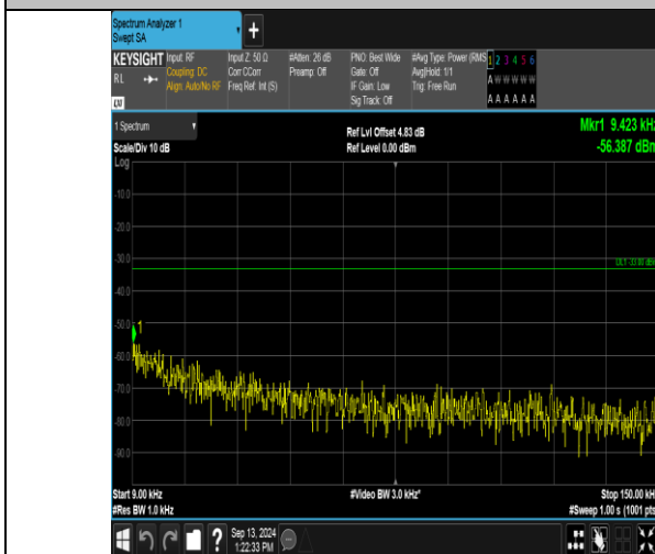
Band12_10MHz_QPSK_23060_1RB#0_0.009~0.15_0.009~0.15
