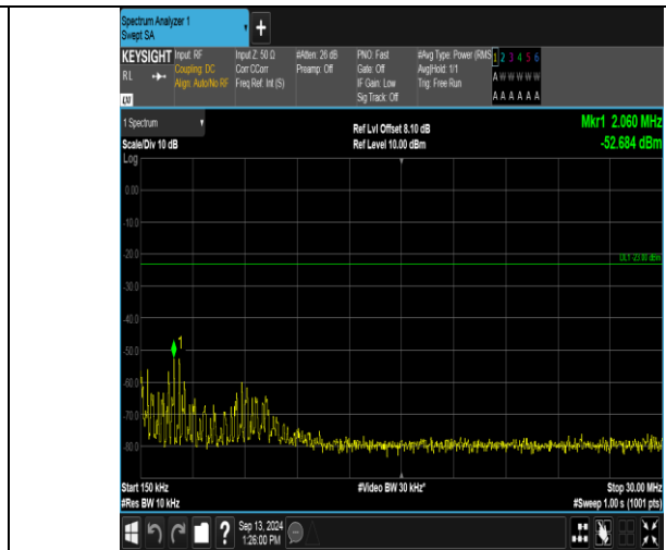
Band12_10MHz_QPSK_23060_50RB#0_0.15~30_0.15~30
