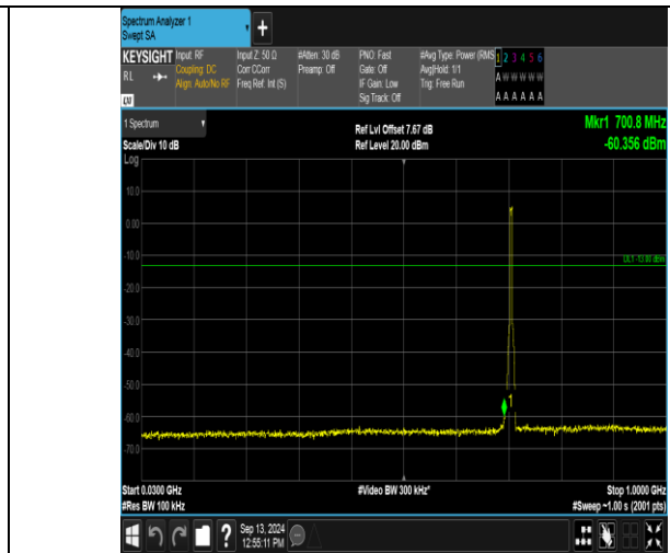
Band12_5MHz_16QAM_23155_25RB#0_30~1000_30~1000
