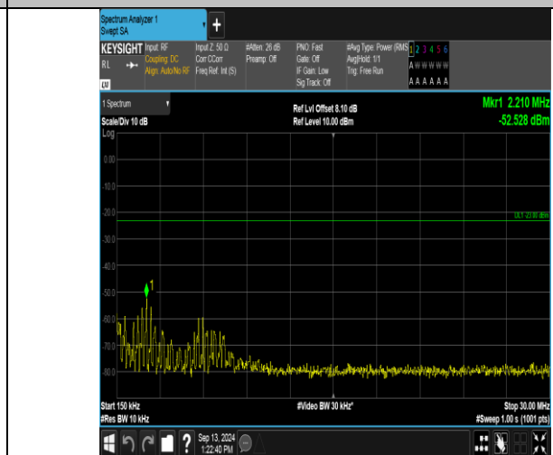
Band12_10MHz_QPSK_23060_1RB#0_0.15~30_0.15~30
