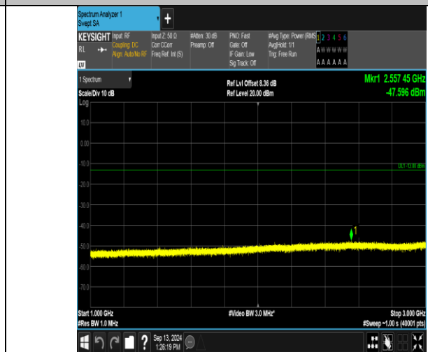
Band12_10MHz_QPSK_23060_50RB#0_1000~3000_1000~3000
