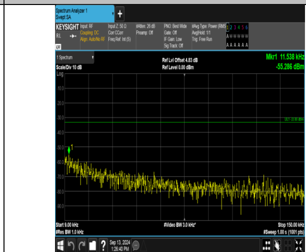
Band12_10MHz_16QAM_23060_50RB#0_0.009~0.15_0.009~0.15
