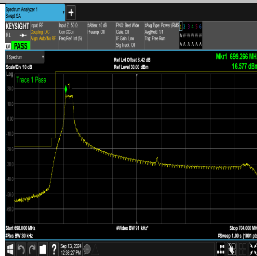
Band12_5MHz_QPSK_23035_1RB#0
