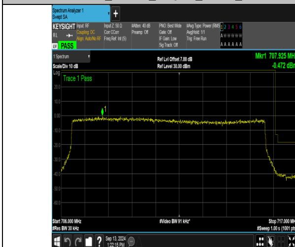
Band12_10MHz_16QAM_23130_50RB#0
