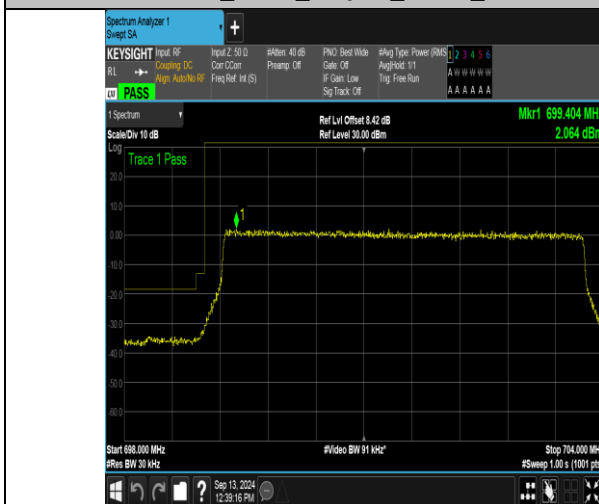
Band12_5MHz_16QAM_23035_25RB#0
