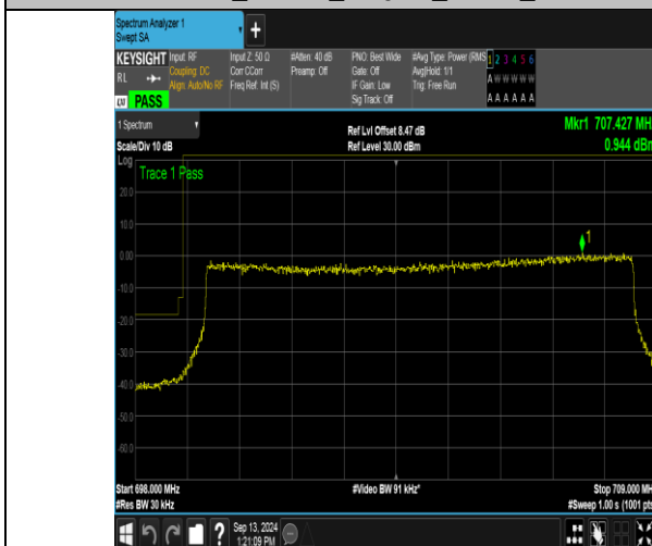
Band12_10MHz_16QAM_23060_50RB#0
