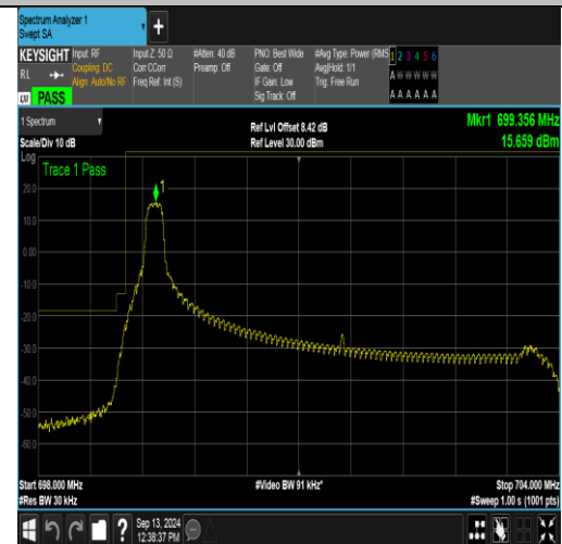
Band12_5MHz_16QAM_23035_1RB#0
