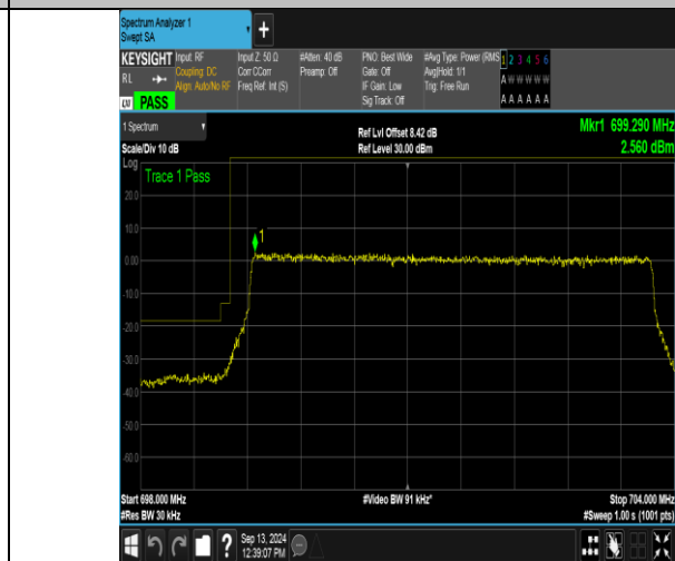
Band12_5MHz_QPSK_23035_25RB#0
