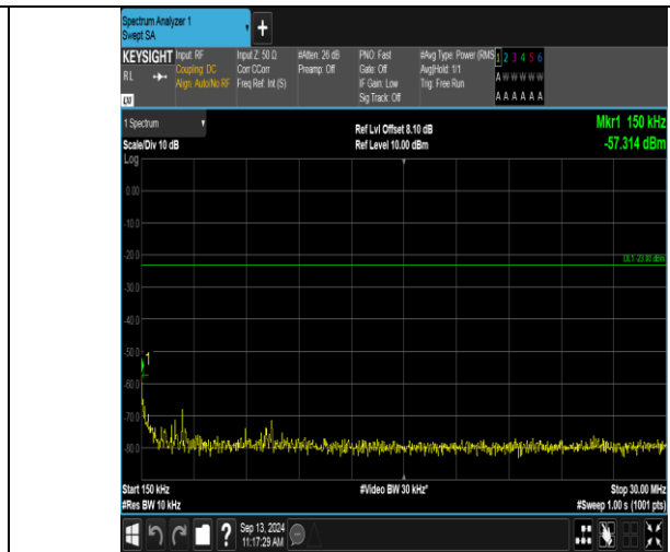
Band12_1.4MHz_QPSK_23017_6RB#0_0.15~30_0.15~30
