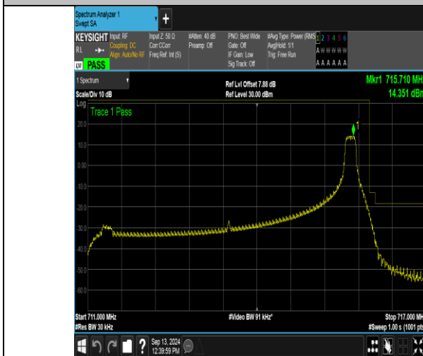
Band12_5MHz_16QAM_23155_1RB#24
