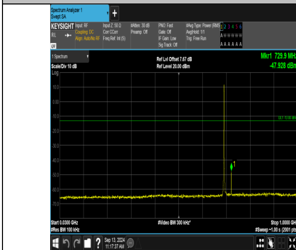
Band12_1.4MHz_QPSK_23017_6RB#0_30~1000_30~1000
