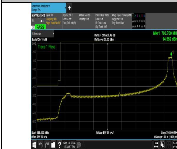
Band12_5MHz_16QAM_23035_1RB#24
