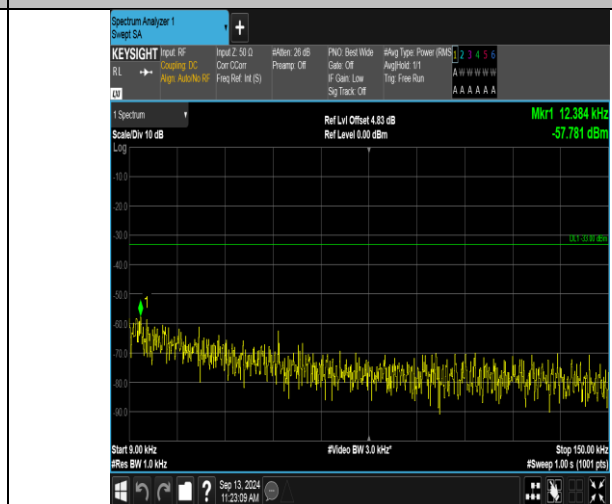
Band12_1.4MHz_16QAM_23095_6RB#0_0.009~0.15_0.009~0.15
