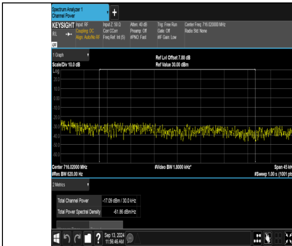
Band12_3MHz_QPSK_23165_1RB#14_Final1
