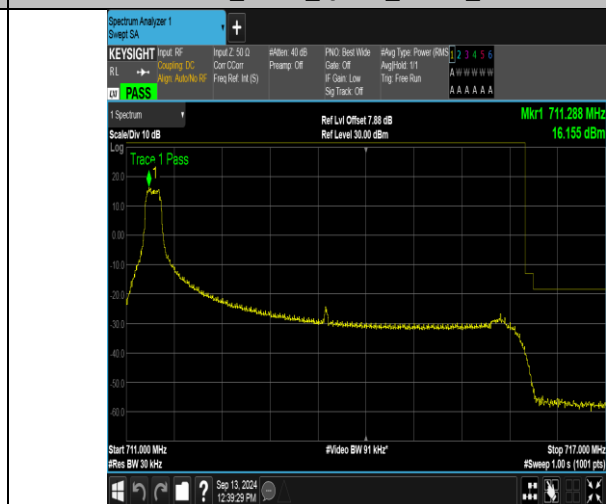
Band12_5MHz_QPSK_23155_1RB#0
