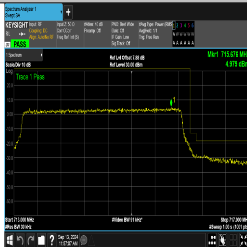
Band12_3MHz_QPSK_23165_15RB#0
