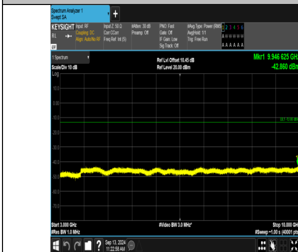
Band12_1.4MHz_QPSK_23095_6RB#0_3000~10000_3000~10000
