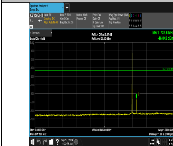
Band12_1.4MHz_QPSK_23095_6RB#0_30~1000_30~1000
