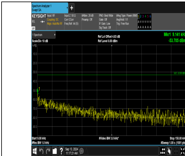
Band12_1.4MHz_QPSK_23017_6RB#0_0.009~0.15_0.009~0.15
