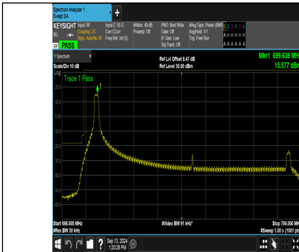
Band12_10MHz_16QAM_23060_1RB#0
