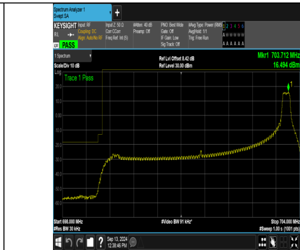
Band12_5MHz_QPSK_23035_1RB#24
