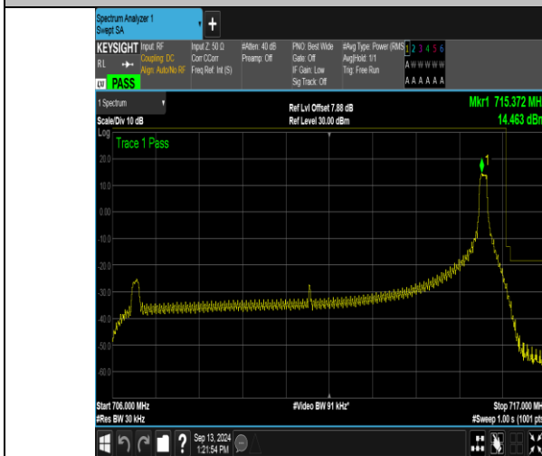
Band12_10MHz_16QAM_23130_1RB#49
