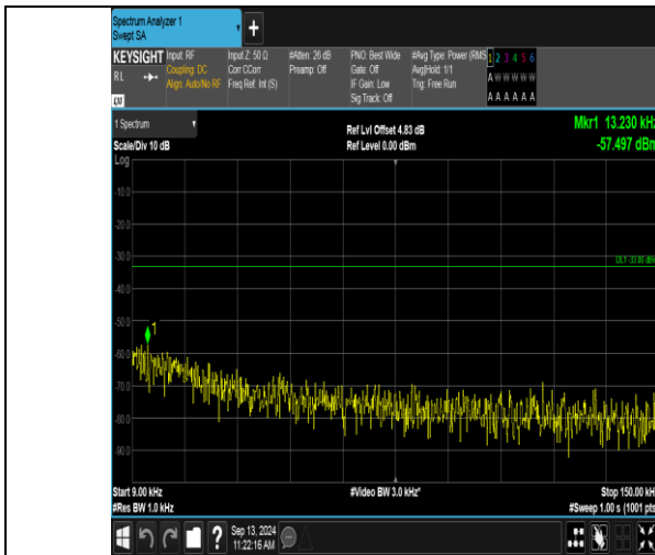
Band12_1.4MHz_QPSK_23095_6RB#0_0.009~0.15_0.009~0.15
