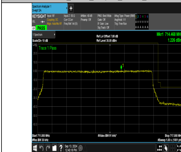
Band12_5MHz_16QAM_23155_25RB#0
