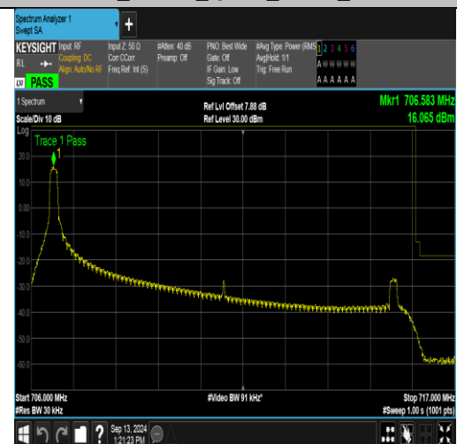
Band12_10MHz_QPSK_23130_1RB#0
