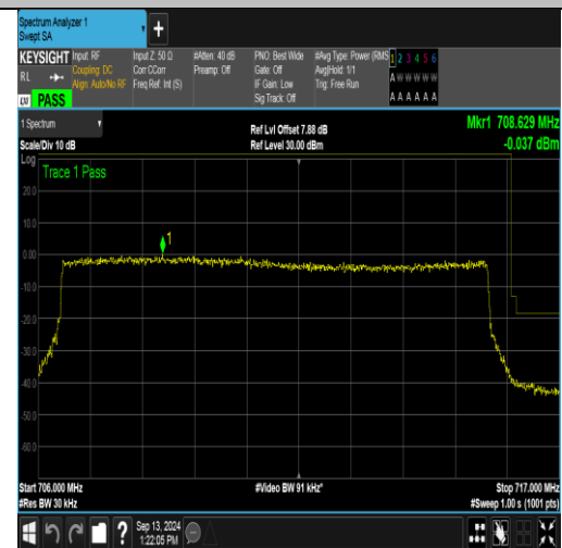
Band12_10MHz_QPSK_23130_50RB#0
