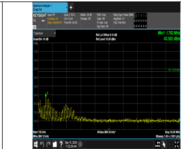
Band12_1.4MHz_QPSK_23095_6RB#0_0.15~30_0.15~30
