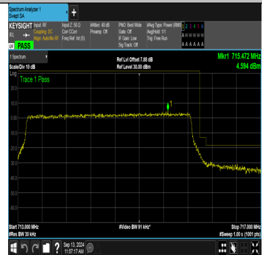
Band12_3MHz_16QAM_23165_15RB#0
