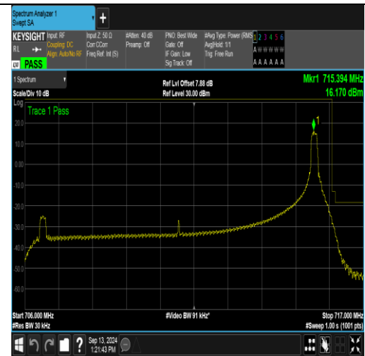
Band12_10MHz_QPSK_23130_1RB#49
