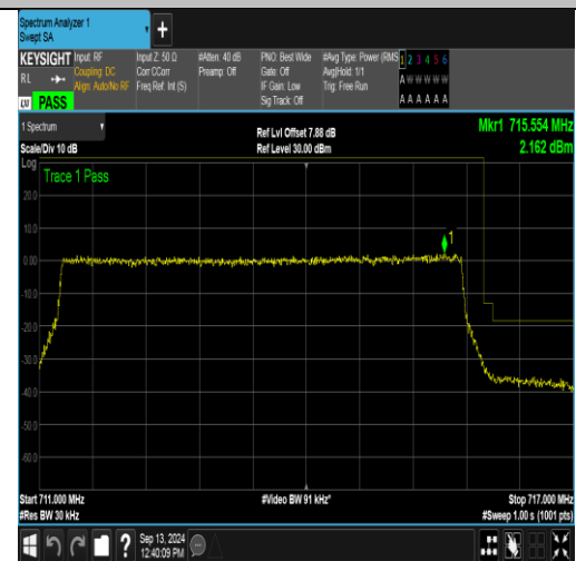
Band12_5MHz_QPSK_23155_25RB#0
