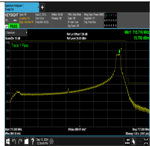
Band12_5MHz_QPSK_23155_1RB#24
