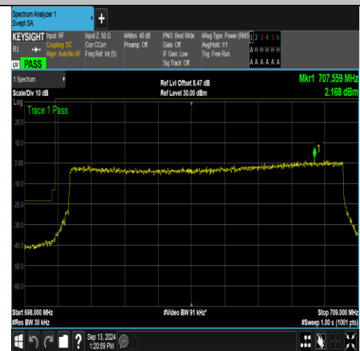
Band12_10MHz_QPSK_23060_50RB#0
