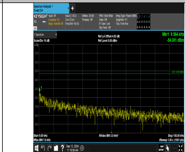
Band12_1.4MHz_16QAM_23017_6RB#0_0.009~0.15_0.009~0.15
