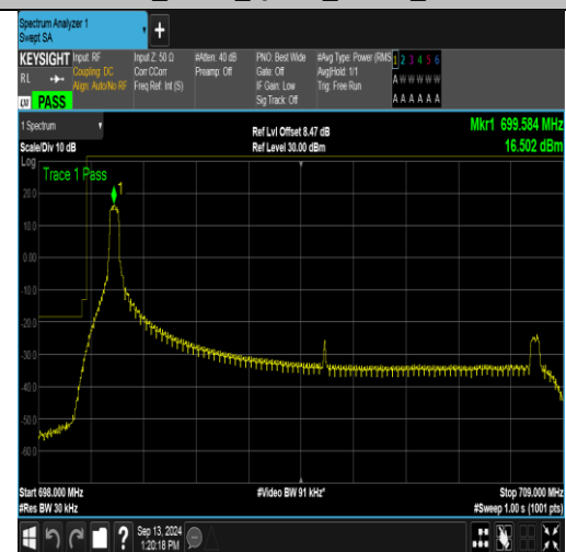
Band12_10MHz_QPSK_23060_1RB#0
