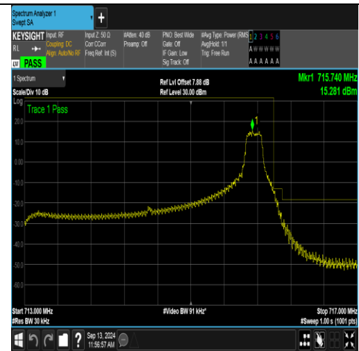
Band12_3MHz_16QAM_23165_1RB#14
