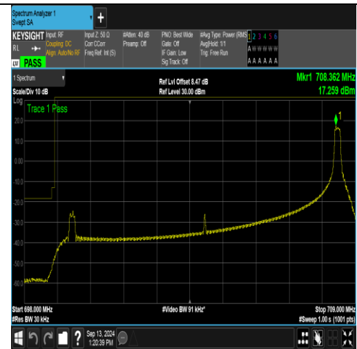
Band12_10MHz_QPSK_23060_1RB#49
