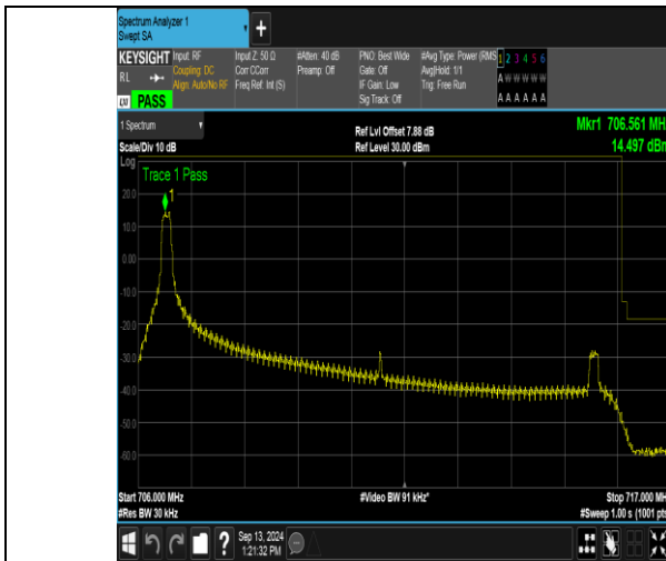
Band12_10MHz_16QAM_23130_1RB#0
