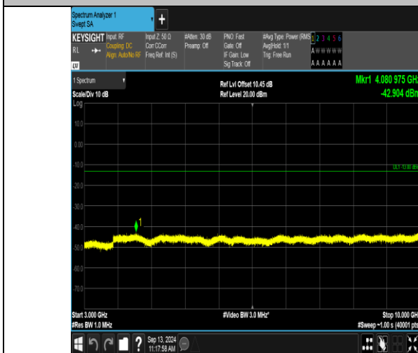
Band12_1.4MHz_QPSK_23017_6RB#0_3000~10000_3000~10000
