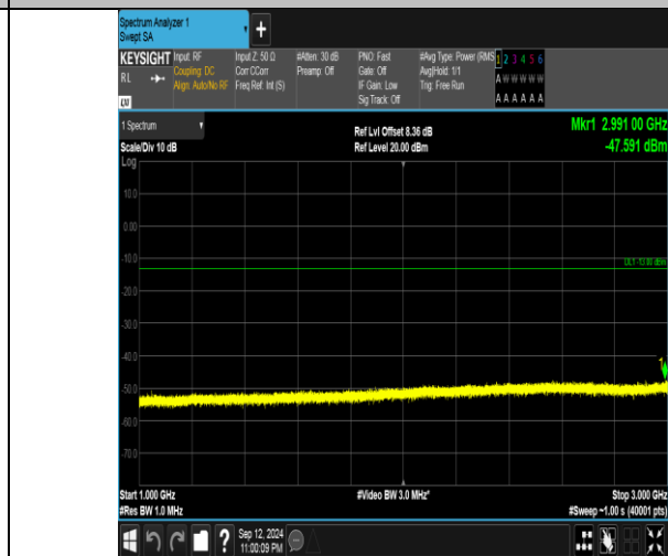
Band5_1.4MHz_QPSK_20407_6RB#0_1000~3000_1000~3000
