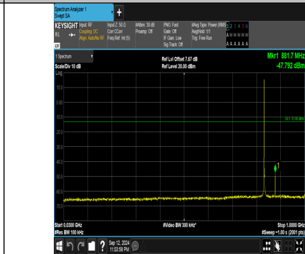
Band5_1.4MHz_16QAM_20525_1RB#5_30~1000_30~1000
