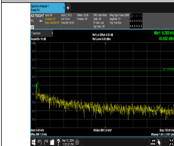
Band5_1.4MHz_QPSK_20525_1RB#0_0.009~0.15_0.009~0.15
