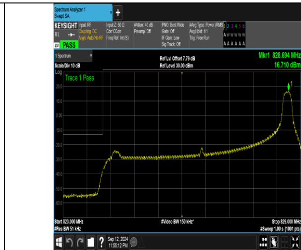
Band5_5MHz_16QAM_20425_1RB#24
