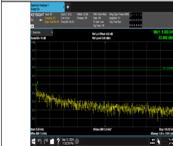
Band5_1.4MHz_QPSK_20525_1RB#5_0.009~0.15_0.009~0.15
