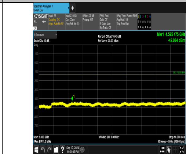
Band5_1.4MHz_16QAM_20407_6RB#0_3000~10000_3000~10000
