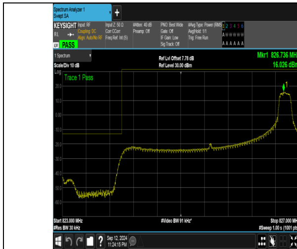
Band5_3MHz_QPSK_20415_1RB#14
