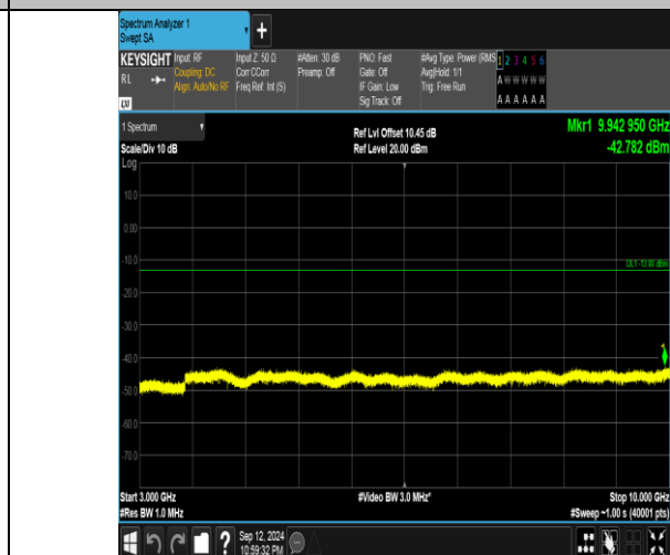
Band5_1.4MHz_16QAM_20407_1RB#5_3000~10000_3000~10000
