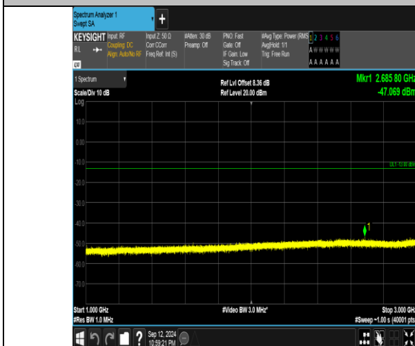
Band5_1.4MHz_16QAM_20407_1RB#5_1000~3000_1000~3000
