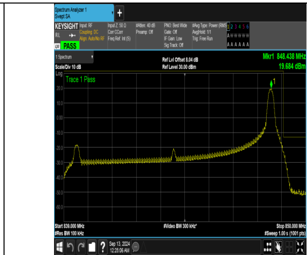
Band5_10MHz_16QAM_20600_1RB#49
