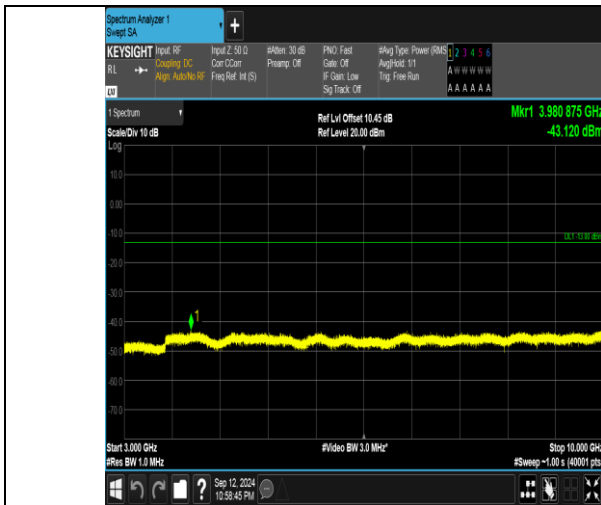
Band5_1.4MHz_QPSK_20407_1RB#5_3000~10000_3000~10000
