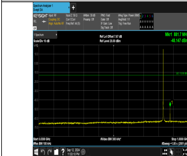
Band5_1.4MHz_QPSK_20525_1RB#5_30~1000_30~1000
