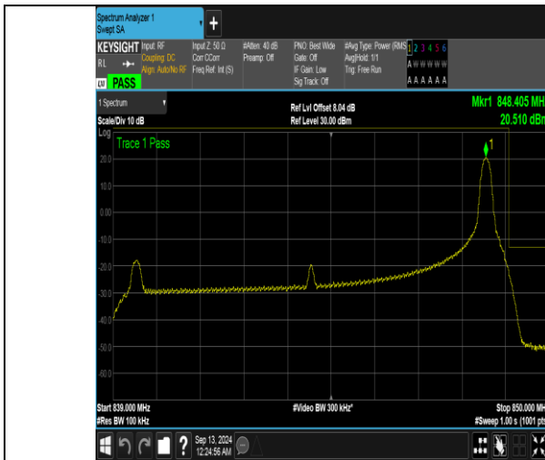
Band5_10MHz_QPSK_20600_1RB#49
