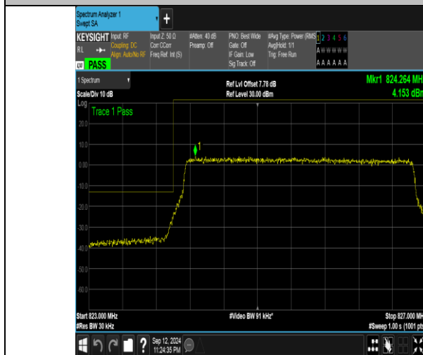
Band5_3MHz_QPSK_20415_15RB#0
