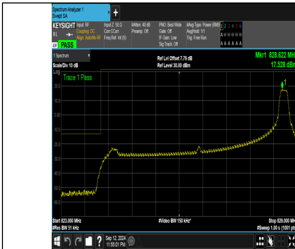
Band5_5MHz_QPSK_20425_1RB#24
