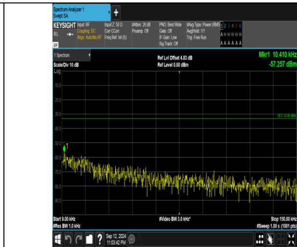
Band5_1.4MHz_16QAM_20525_1RB#5_0.009~0.15_0.009~0.15
