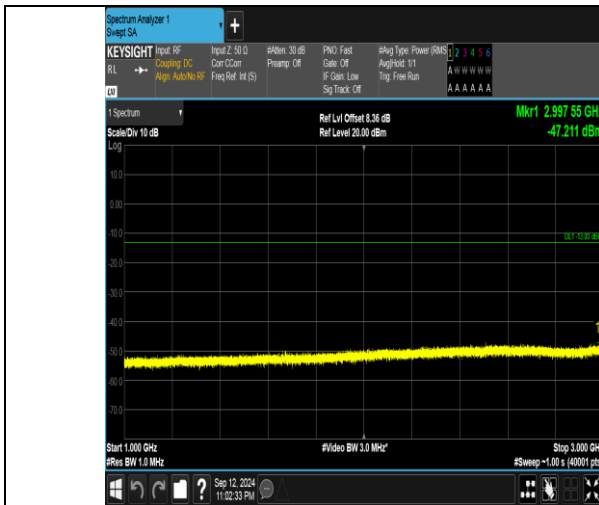
Band5_1.4MHz_16QAM_20525_1RB#0_1000~3000_1000~3000
