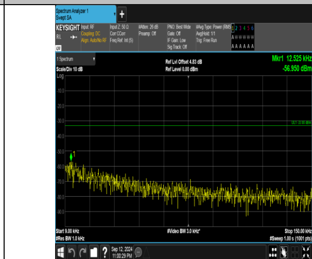
Band5_1.4MHz_16QAM_20407_6RB#0_0.009~0.15_0.009~0.15
