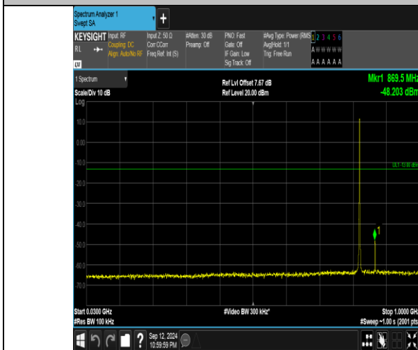
Band5_1.4MHz_QPSK_20407_6RB#0_30~1000_30~1000
