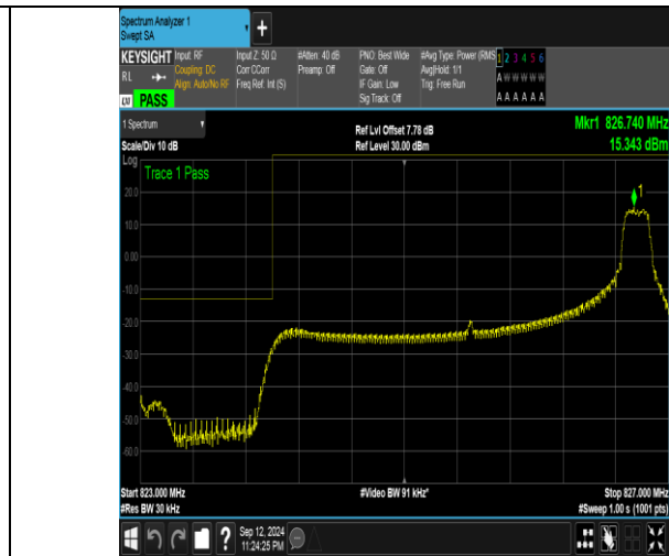
Band5_3MHz_16QAM_20415_1RB#14
