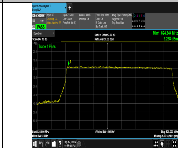
Band5_5MHz_16QAM_20425_25RB#0
