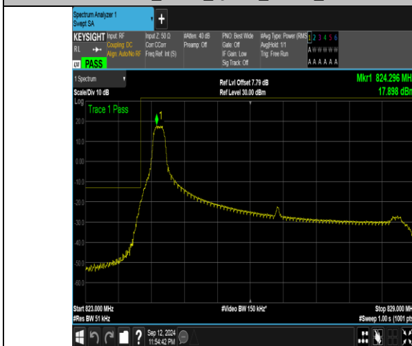
Band5_5MHz_QPSK_20425_1RB#0
