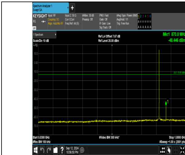
Band5_1.4MHz_QPSK_20407_1RB#0_30~1000_30~1000
