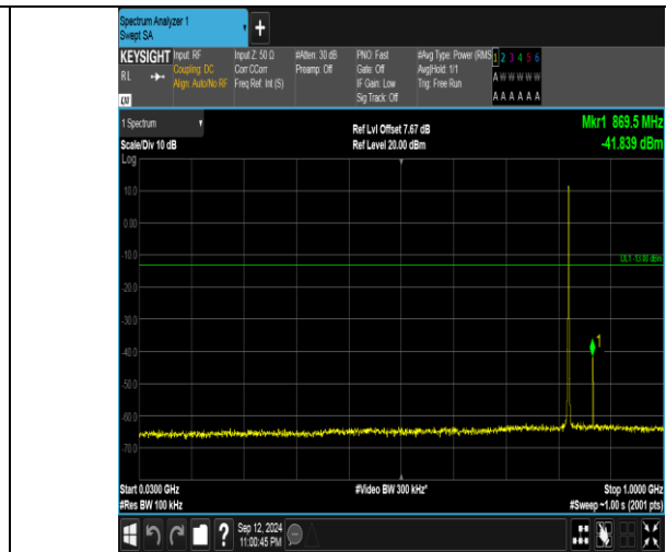
Band5_1.4MHz_16QAM_20407_6RB#0_30~1000_30~1000
