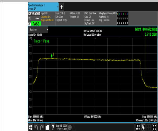
Band5_10MHz_16QAM_20600_50RB#0
