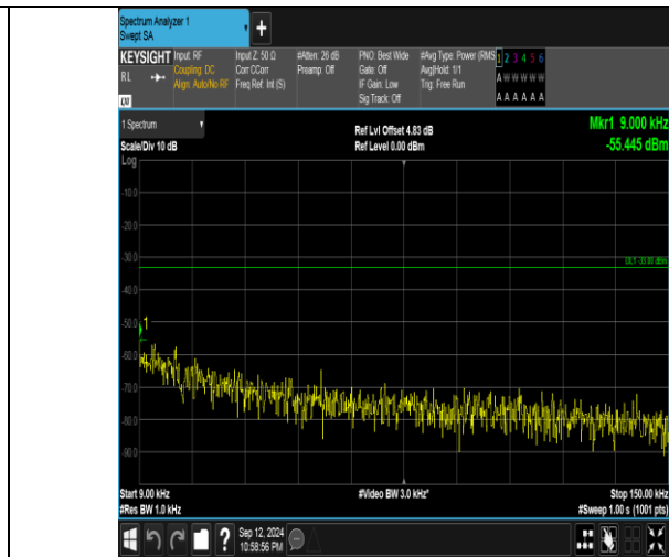
Band5_1.4MHz_16QAM_20407_1RB#5_0.009~0.15_0.009~0.15
