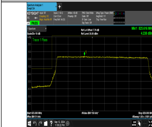
Band5_5MHz_QPSK_20425_25RB#0
