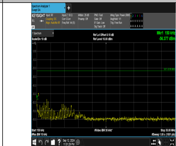
Band5_1.4MHz_QPSK_20525_1RB#0_0.15~30_0.15~30
