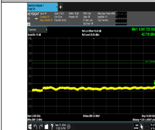
Band5_1.4MHz_QPSK_20407_6RB#0_3000~10000_3000~10000
