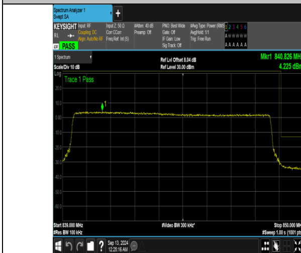
Band5_10MHz_QPSK_20600_50RB#0
