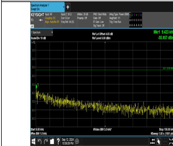
Band5_1.4MHz_QPSK_20407_1RB#5_0.009~0.15_0.009~0.15
