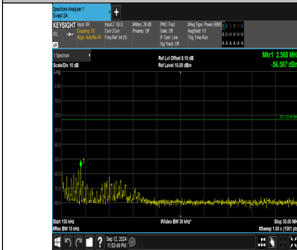
Band5_1.4MHz_16QAM_20525_1RB#5_0.15~30_0.15~30
