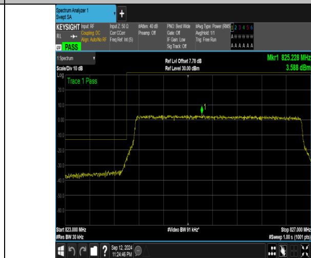
Band5_3MHz_16QAM_20415_15RB#0
