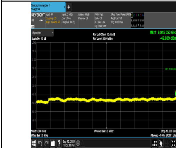
Band5_1.4MHz_QPSK_20407_1RB#0_3000~10000_3000~10000
