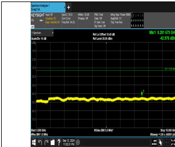
Band5_1.4MHz_QPSK_20525_1RB#5_3000~10000_3000~10000
