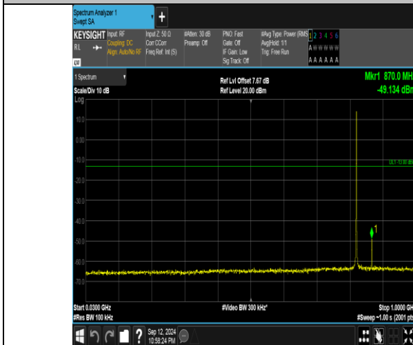
Band5_1.4MHz_QPSK_20407_1RB#5_30~1000_30~1000
