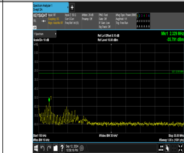
Band5_1.4MHz_QPSK_20407_1RB#5_0.15~30_0.15~30
