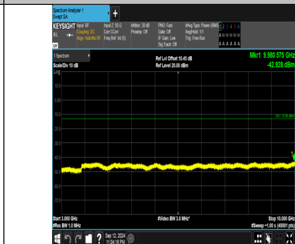
Band5_1.4MHz_16QAM_20525_1RB#5_3000~10000_3000~10000
