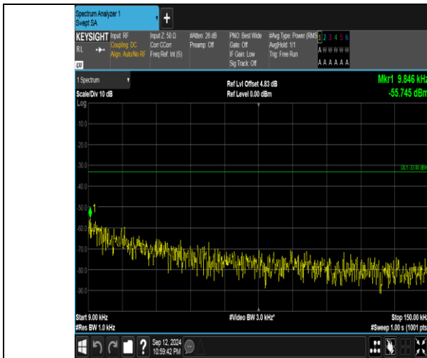
Band5_1.4MHz_QPSK_20407_6RB#0_0.009~0.15_0.009~0.15
