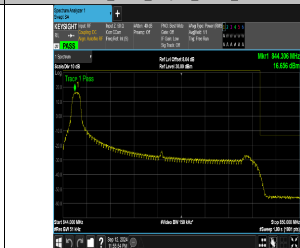
Band5_5MHz_16QAM_20625_1RB#0
