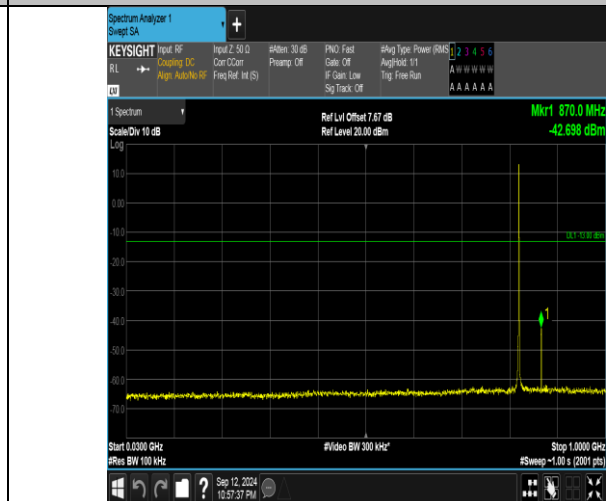
Band5_1.4MHz_16QAM_20407_1RB#0_30~1000_30~1000
