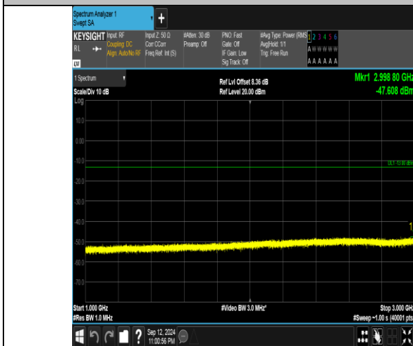
Band5_1.4MHz_16QAM_20407_6RB#0_1000~3000_1000~3000
