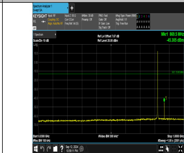
Band5_1.4MHz_16QAM_20407_1RB#5_30~1000_30~1000
