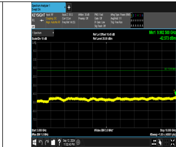
Band5_1.4MHz_16QAM_20525_1RB#0_3000~10000_3000~10000
