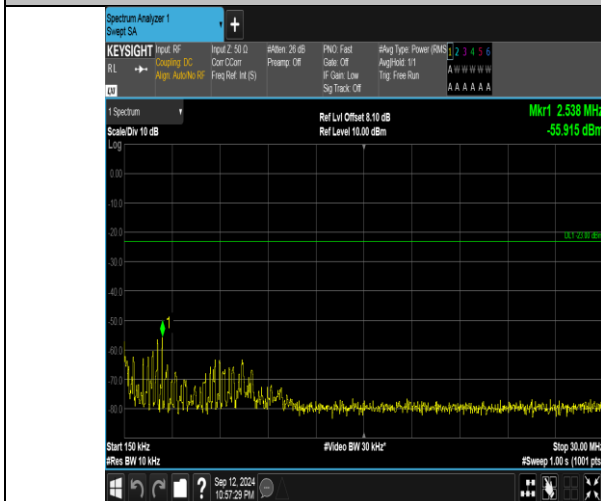
Band5_1.4MHz_16QAM_20407_1RB#0_0.15~30_0.15~30
