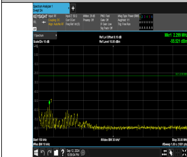
Band5_1.4MHz_16QAM_20407_1RB#5_0.15~30_0.15~30
