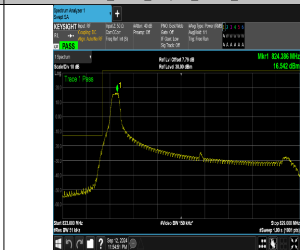
Band5_5MHz_16QAM_20425_1RB#0
