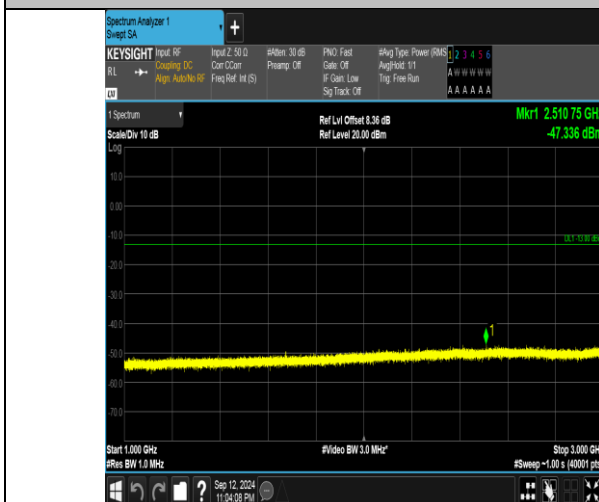
Band5_1.4MHz_16QAM_20525_1RB#5_1000~3000_1000~3000
