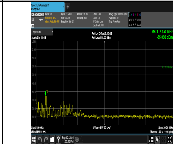
Band5_1.4MHz_QPSK_20525_1RB#5_0.15~30_0.15~30
