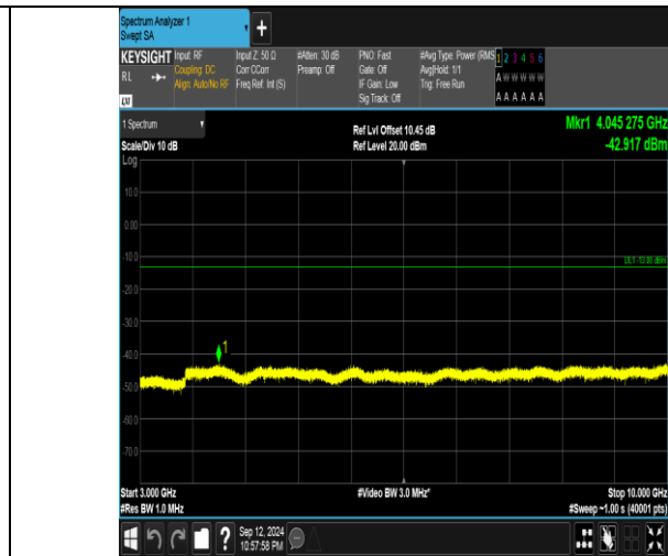
Band5_1.4MHz_16QAM_20407_1RB#0_3000~10000_3000~10000
