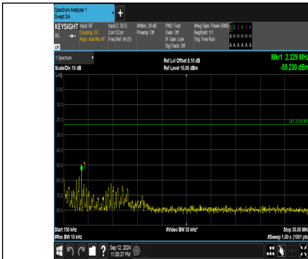
Band5_1.4MHz_16QAM_20407_6RB#0_0.15~30_0.15~30
