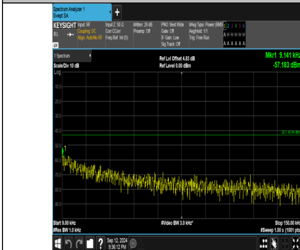
Band4_15MHz_QPSK_20325_1RB#74_0.009~0.15_0.009~0.15
