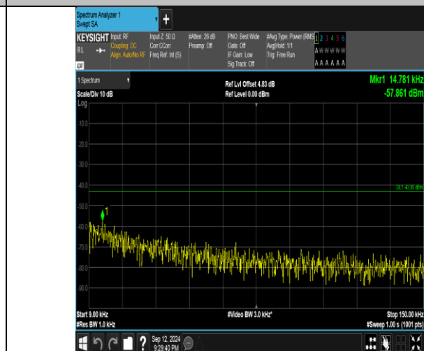
Band4_15MHz_16QAM_20175_1RB#0_0.009~0.15_0.009~0.15
