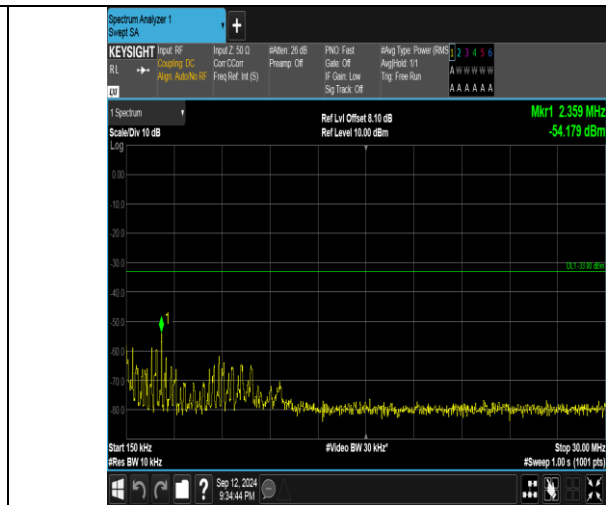
Band4_15MHz_QPSK_20325_1RB#0_0.15-30_0.15-30
