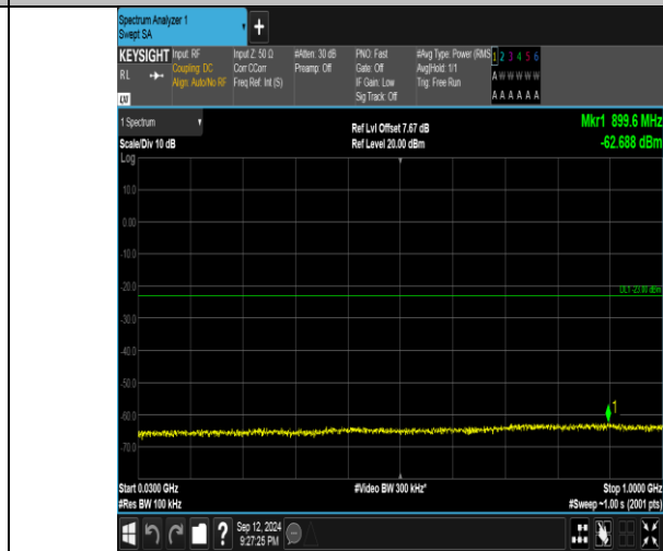
Band4_15MHz_16QAM_20025_75RB#0_30~1000_30~1000
