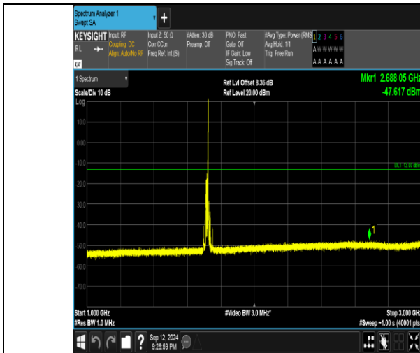
Band4_15MHz_16QAM_20025_1RB#74_1000~3000_1000~3000
