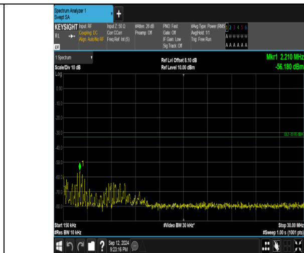
Band4_15MHz_QPSK_20025_1RB#0_0.15-30_0.15-30
