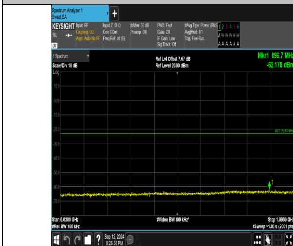
Band4_15MHz_QPSK_20025_75RB#0_30~1000_30~1000
