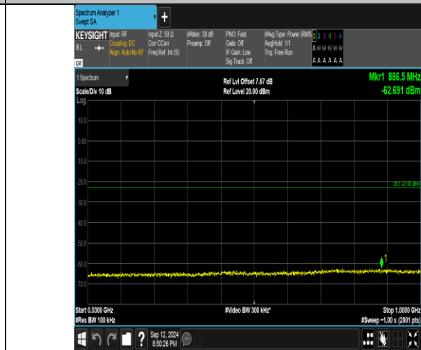
Band4_10MHz_16QAM_20350_50RB#0_30~1000_30~1000
