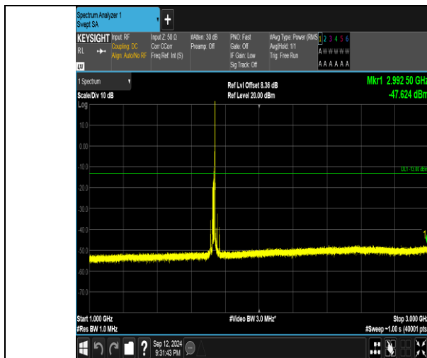
Band4_15MHz_16QAM_20175_1RB#74_1000~3000_1000~3000
