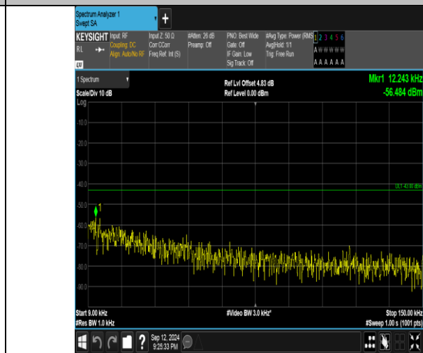
Band4_15MHz_16QAM_2025_1RB#74_0.009~0.15_0.009~0.15
