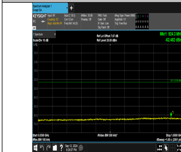
Band4_15MHz_QPSK_20175_1RB#0_30~1000_30~1000
