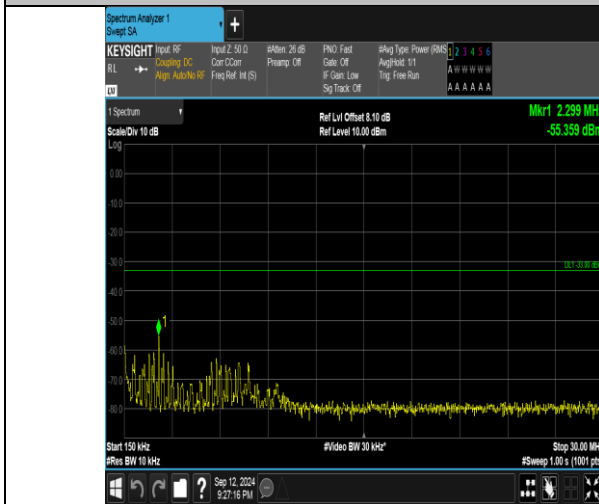
Band4_15MHz_16QAM_20025_75RB#0_0.15~30_0.15~30
