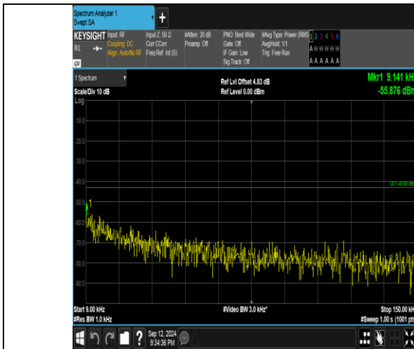
Band4_15MHz_QPSK_20325_1RB#0_0.009-0.15_0.009-0.15
