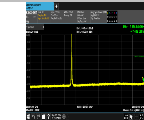
Band4_15MHz_QPSK_20175_1RB#0_1000~3000_1000~3000
