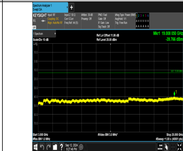
Band4_15MHz_16QAM_20025_75RB#0_3000~20000_3000~20000
