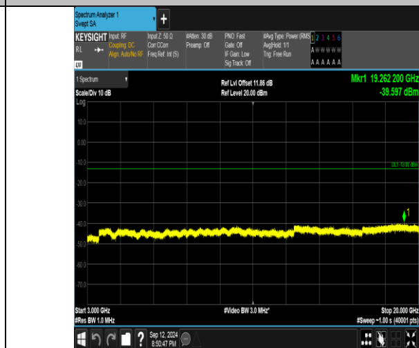
Band4_10MHz_16QAM_20350_50RB#0_3000~20000_3000~20000
