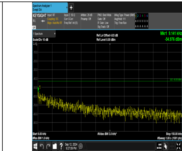
Band4_15MHz_16QAM_20025_75RB#0_0.009~0.15_0.009~0.15
