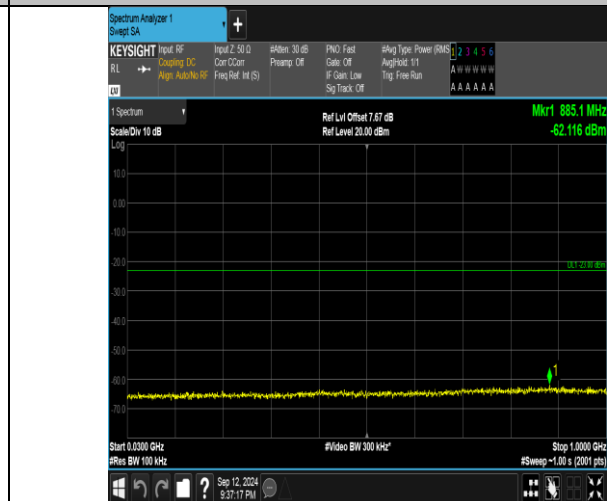
Band4_15MHz_16QAM_20325_1RB#74_30~1000_30~1000
