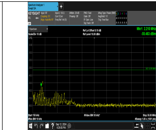
Band4_15MHz_QPSK_20175_1RB#0_0.15~30_0.15~30
