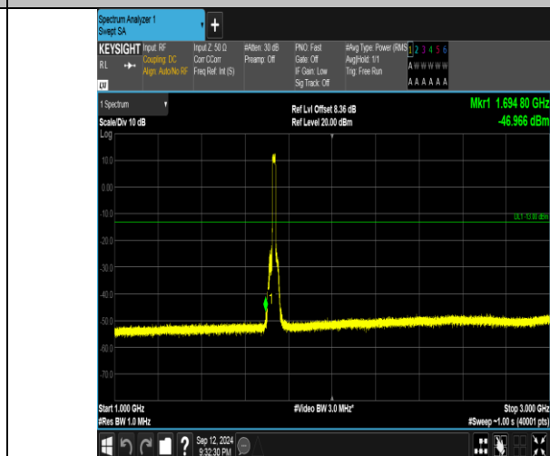
Band4_15MHz_QPSK_20175_75RB#0_1000~3000_1000~3000
