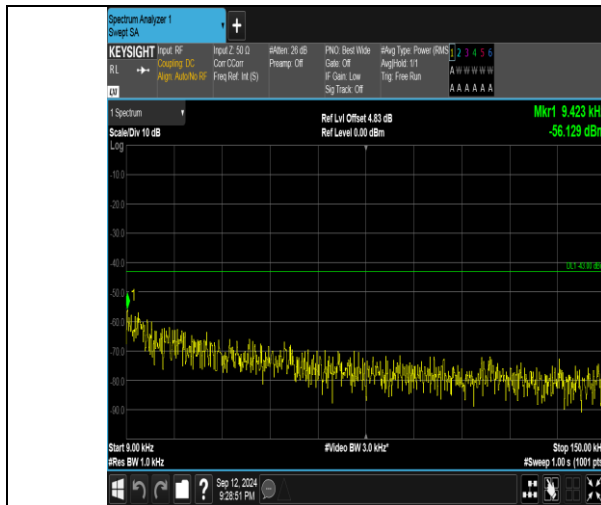
Band4_15MHz_QPSK_20175_1RB#0_0.009~0.15_0.009~0.15
