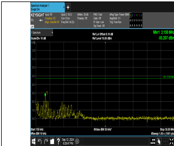
Band4_15MHz_16QAM_20175_1RB#0_0.15~30_0.15~30
