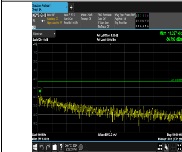
Band4_15MHz_QPSK_20025_75RB#0_0.009~0.15_0.009~0.15
