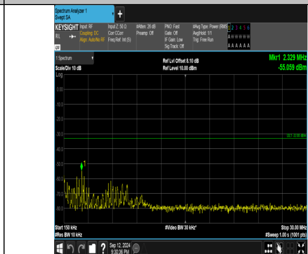
Band4_15MHz_QPSK_20175_1RB#74_0.15~30_0.15~30
