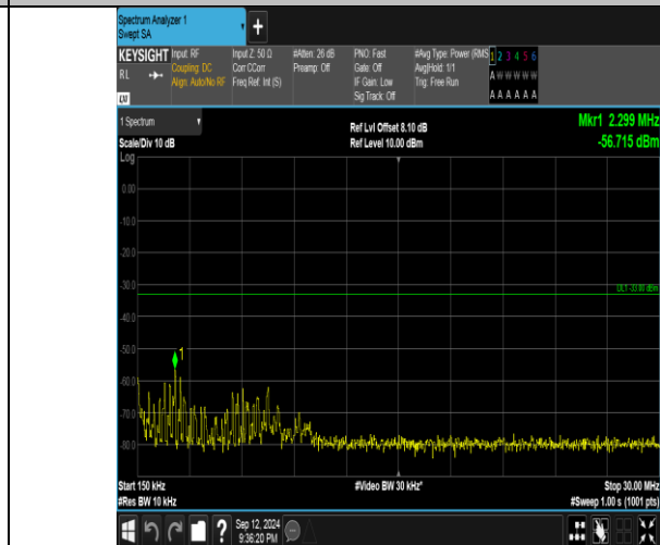
Band4_15MHz_QPSK_20325_1RB#74_0.15~30_0.15~30
