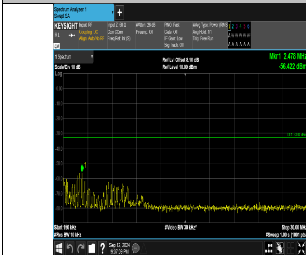
Band4_15MHz_16QAM_20325_1RB#74_0.15~30_0.15~30
