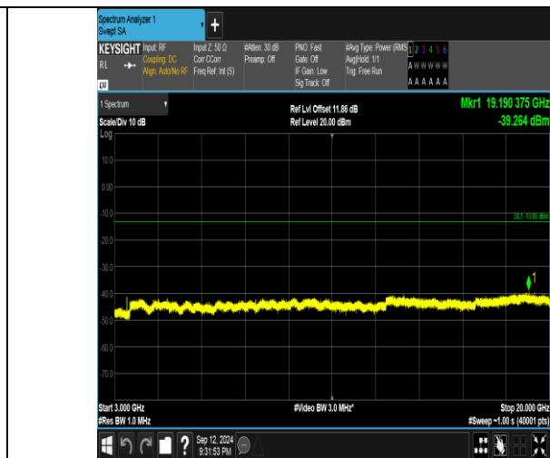
Band4_15MHz_16QAM_20175_1RB#74_3000~20000_3000~20000
