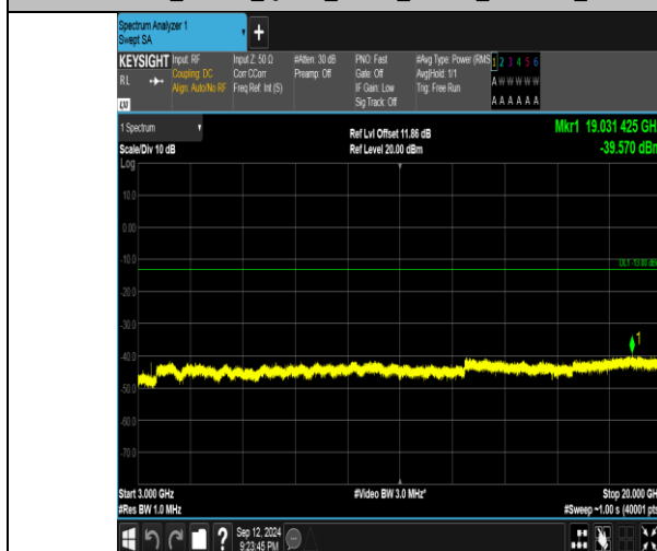
Band4_15MHz_QPSK_20025_1RB#0_3000-20000_3000-20000
