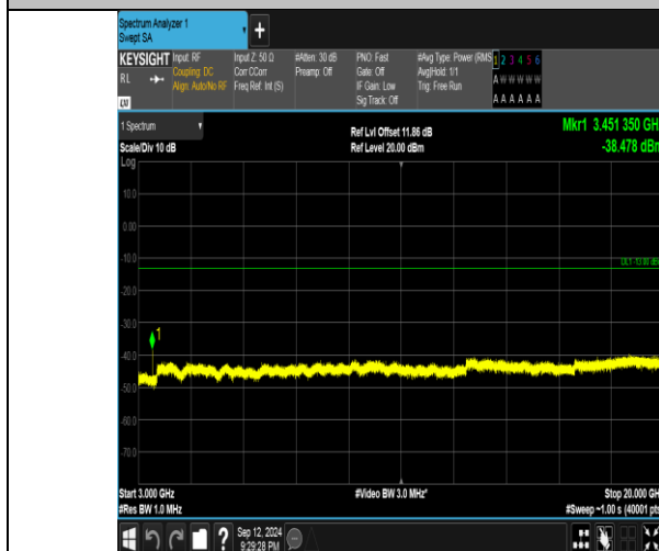
Band4_15MHz_QPSK_20175_1RB#0_3000~20000_3000~20000
