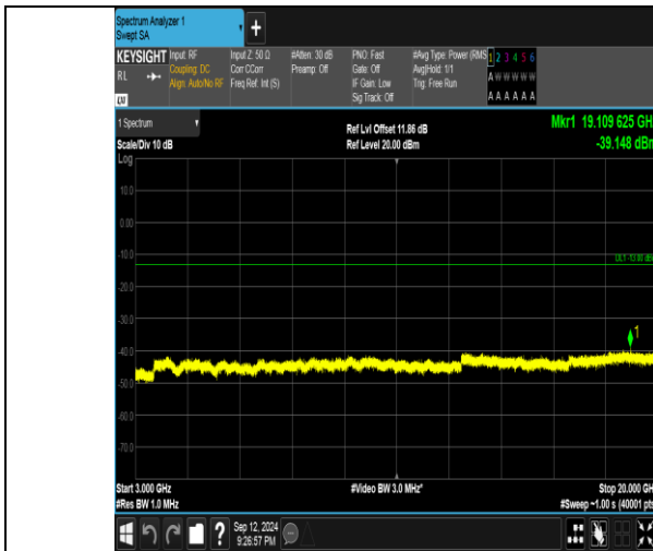
Band4_15MHz_QPSK_20025_75RB#0_3000~20000_3000~20000
