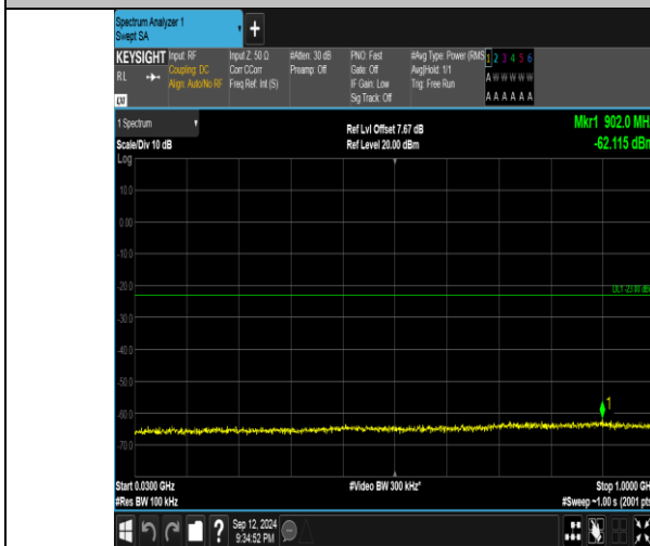
Band4_15MHz_QPSK_20325_1RB#0_30-1000_30-1000
