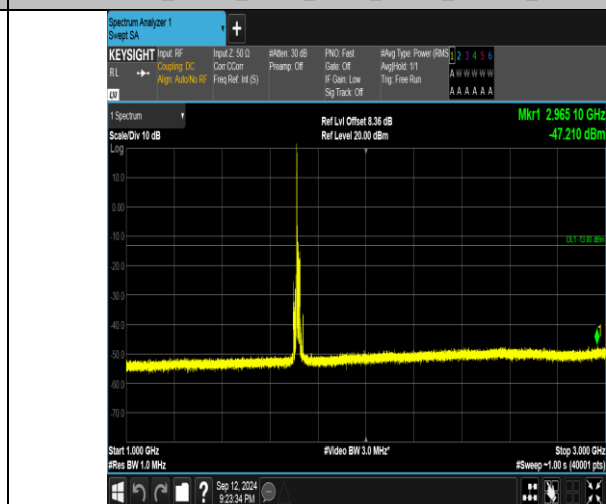
Band4_15MHz_QPSK_20025_1RB#0_1000-3000_1000-3000
