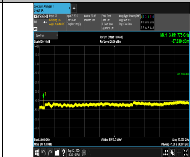
Band4_15MHz_16QAM_20175_1RB#0_3000~20000_3000~20000
