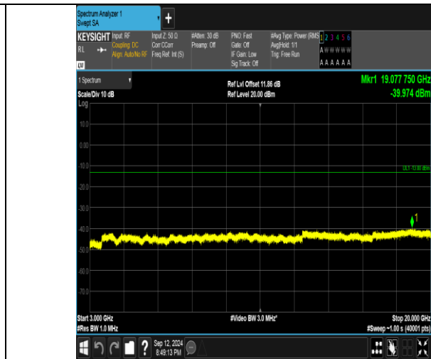
Band4_10MHz_16QAM_20350_1RB#49_3000~20000_3000~20000
