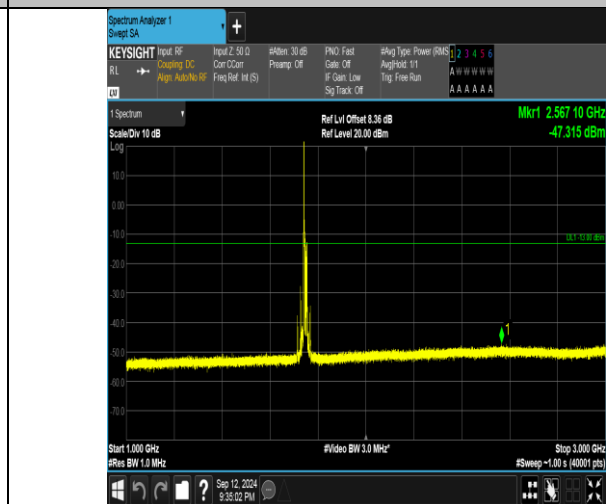
Band4_15MHz_QPSK_20325_1RB#0_1000-3000_1000-3000
