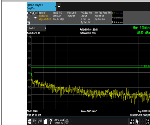
Band4_15MHz_QPSK_20175_75RB#0_0.009~0.15_0.009~0.15
