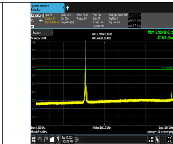
Band4_15MHz_QPSK_2025_1RB#74_1000~3000_1000~3000
