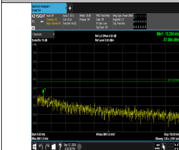
Band4_15MHz_QPSK_20175_1RB#74_0.009~0.15_0.009~0.15
