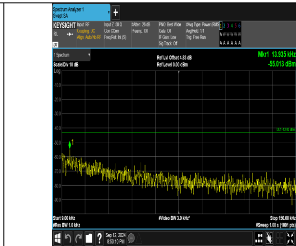
Band4_10MHz_16QAM_20350_50RB#0_0.009~0.15_0.009~0.15
