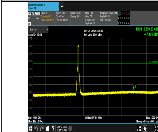
Band4_15MHz_16QAM_20025_75RB#0_1000~3000_1000~3000
