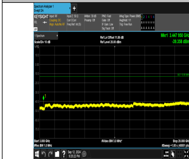
Band4_15MHz_QPSK_2025_1RB#74_3000~20000_3000~20000
