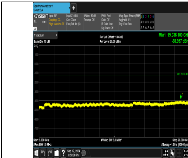
Band4_10MHz_QPSK_20350_50RB#0_3000~20000_3000~20000
