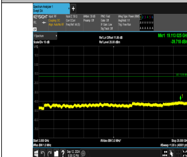
Band4_15MHz_QPSK_20325_1RB#0_3000-20000_3000-20000
