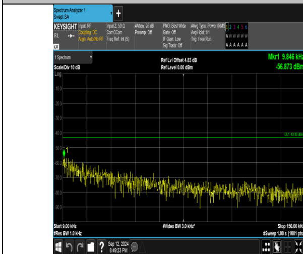
Band4_10MHz_QPSK_20350_50RB#0_0.009~0.15_0.009~0.15
