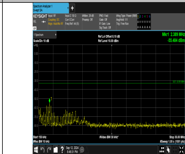
Band4_10MHz_QPSK_20350_50RB#0_0.15~30_0.15~30
