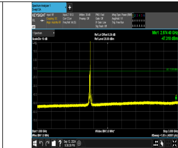
Band4_15MHz_QPSK_20325_1RB#74_1000~3000_1000~3000
