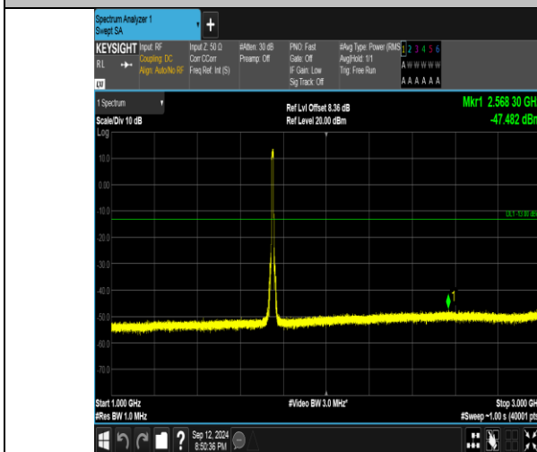
Band4_10MHz_16QAM_20350_50RB#0_1000~3000_1000~3000
