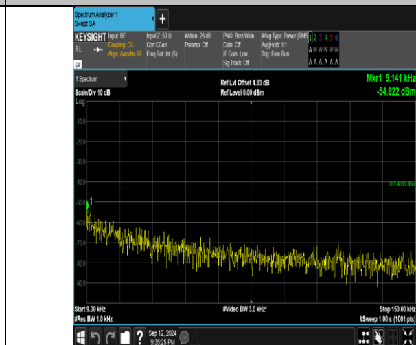
Band4_15MHz_16QAM_20325_1RB#0_0.009-0.15_0.009-0.15
