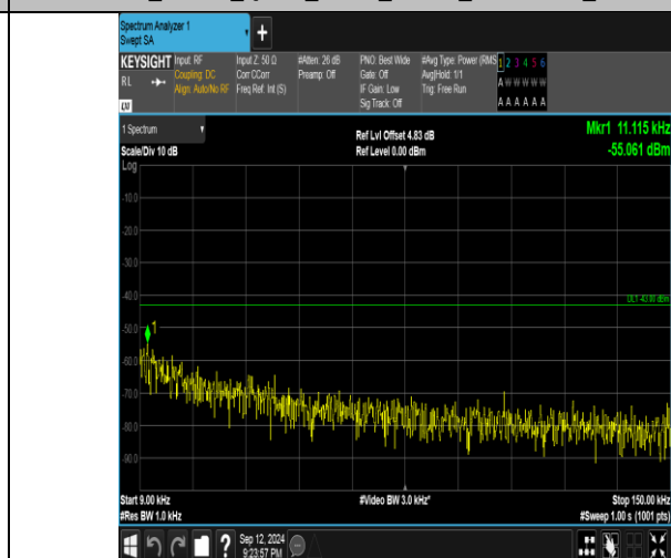
Band4_15MHz_16QAM_20025_1RB#0_0.009-0.15_0.009-0.15
