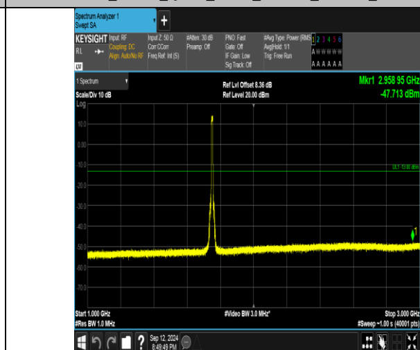
Band4_10MHz_QPSK_20350_50RB#0_1000~3000_1000~3000
