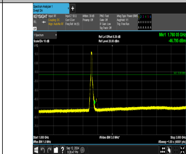
Band4_15MHz_QPSK_20025_75RB#0_1000~3000_1000~3000
