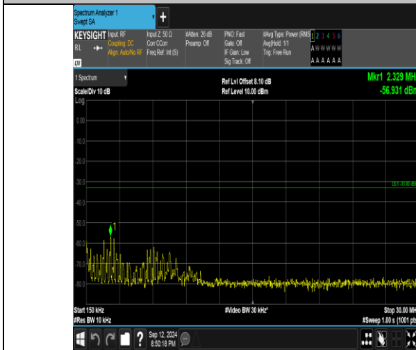
Band4_10MHz_16QAM_20350_50RB#0_0.15~30_0.15~30
