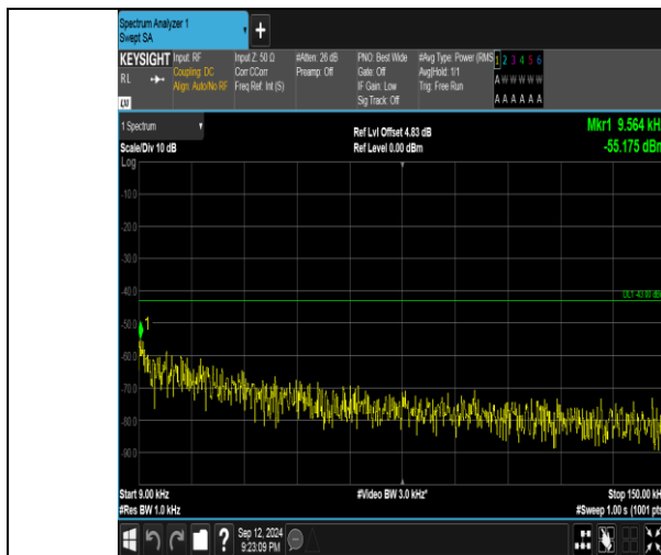
Band4_15MHz_QPSK_20025_1RB#0_0.009-0.15_0.009-0.15
