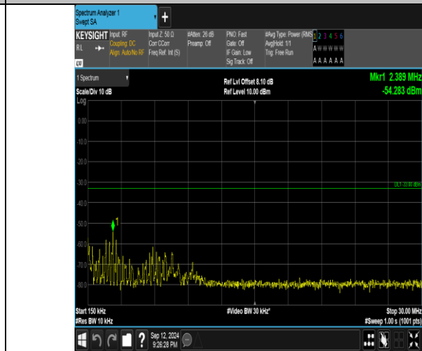
Band4_15MHz_QPSK_20025_75RB#0_0.15~30_0.15~30
