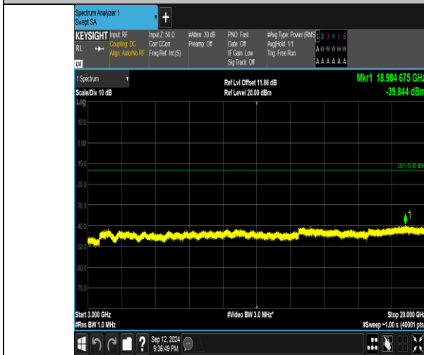
Band4_15MHz_QPSK_20325_1RB#74_3000~20000_3000~20000
