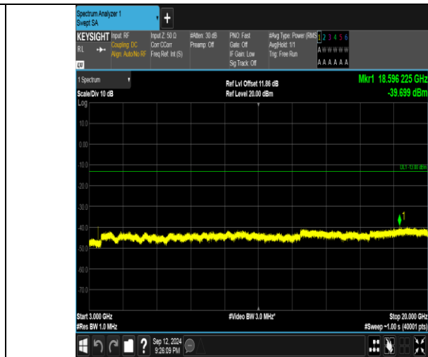
Band4_15MHz_16QAM_20025_1RB#74_3000~20000_3000~20000
