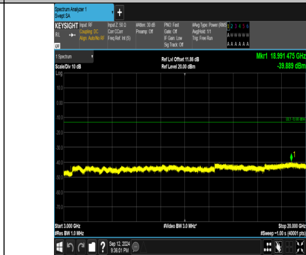
Band4_15MHz_16QAM_20325_1RB#0_3000~20000_3000~20000
