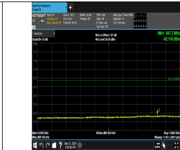
Band4_15MHz_16QAM_20325_1RB#0_30~1000_30~1000
