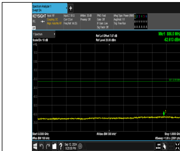
Band4_15MHz_QPSK_2025_1RB#74_30~1000_30~1000
