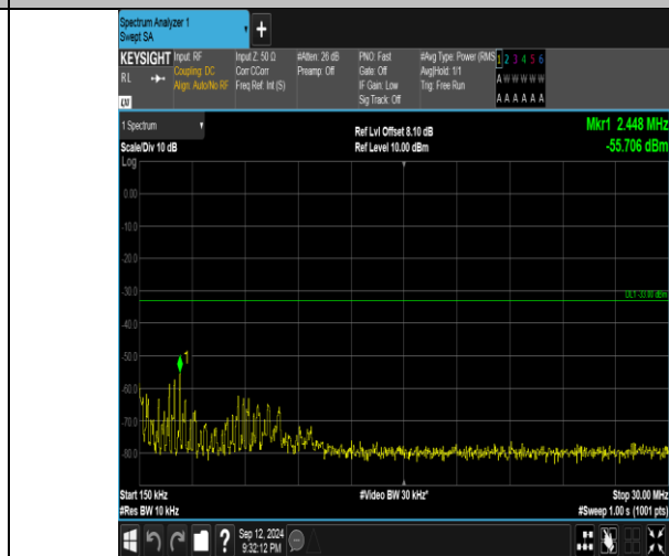
Band4_15MHz_QPSK_20175_75RB#0_0.15~30_0.15~30
