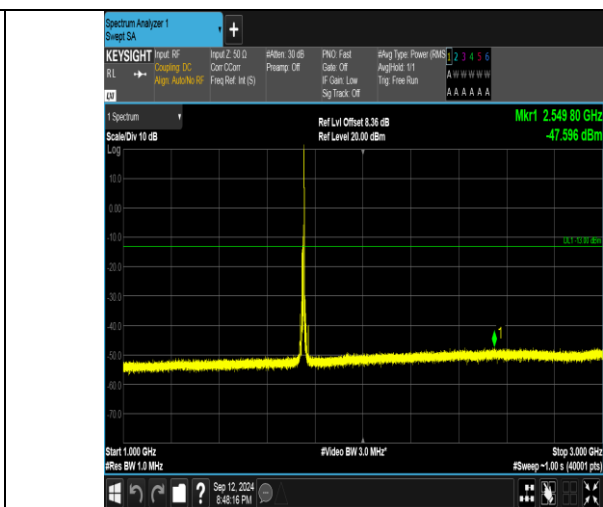
Band4_10MHz_QPSK_20350_1RB#49_1000~3000_1000~3000
