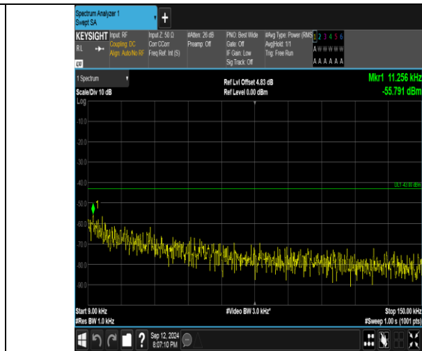
Band4_5MHz_16QAM_20375_25RB#0_0.009~0.15_0.009~0.15
