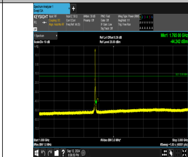
Band4_5MHz_QPSK_20375_25RB#0_1000~3000_1000~3000
