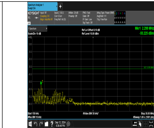
Band4_10MHz_QPSK_20000_1RB#0_0.15~30_0.15~30
