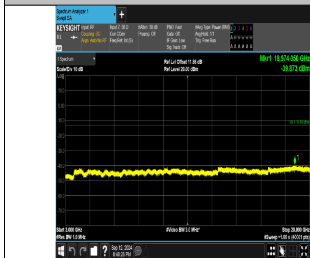
Band4_10MHz_QPSK_20350_1RB#49_3000~20000_3000~20000
