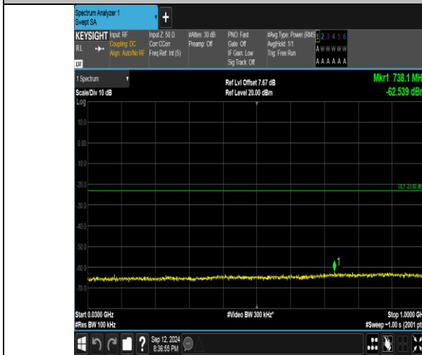
Band4_10MHz_QPSK_20000_1RB#0_30~1000_30~1000
