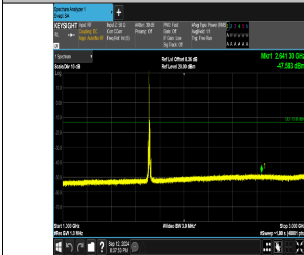
Band4_10MHz_16QAM_20000_1RB#0_1000~3000_1000~3000
