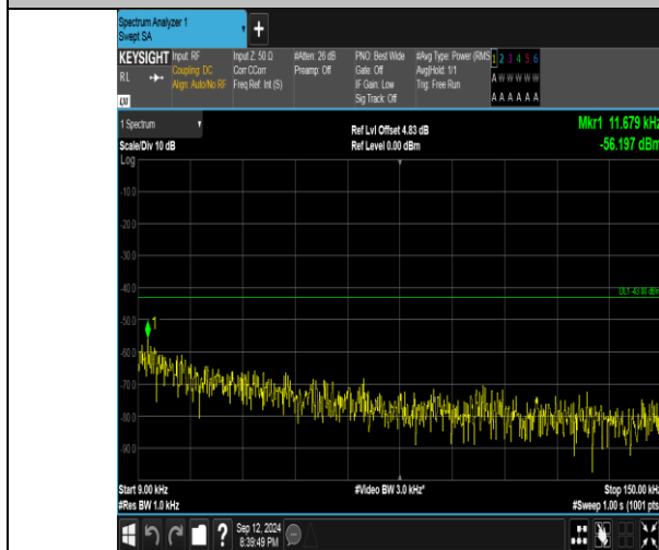
Band4_10MHz_QPSK_20000_50RB#0_0.009~0.15_0.009~0.15
