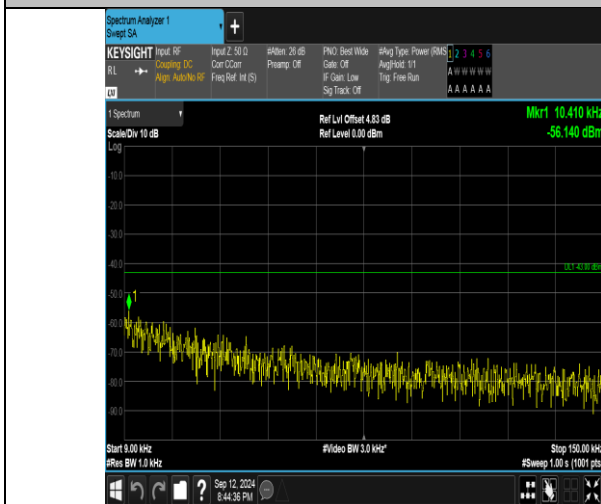
Band4_10MHz_QPSK_20175_50RB#0_0.009~0.15_0.009~0.15
