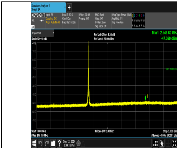
Band4_10MHz_16QAM_20175_1RB#49_1000~3000_1000~3000
