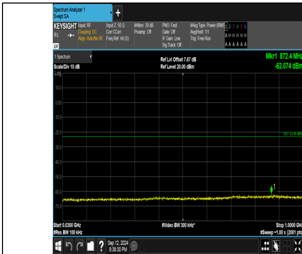
Band4_10MHz_QPSK_20000_1RB#49_30~1000_30~1000
