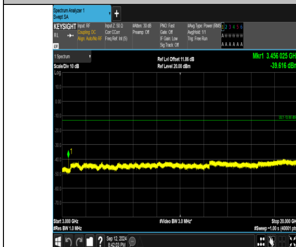
Band4_10MHz_QPSK_20175_1RB#0_3000-20000_3000-20000
