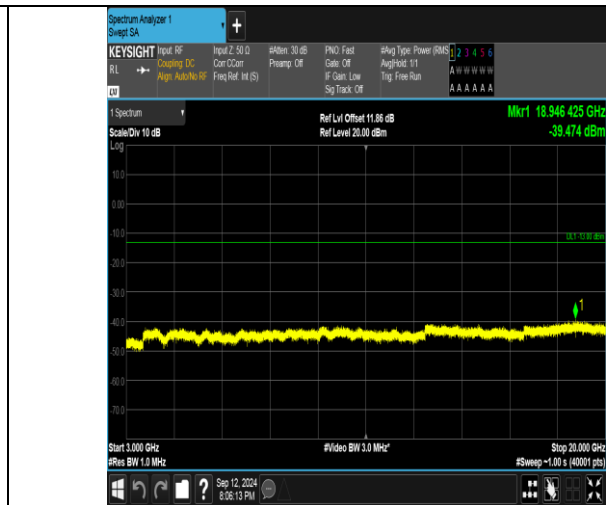
Band4_5MHz_16QAM_20375_1RB#24_3000~20000_3000~20000
