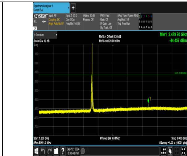
Band4_10MHz_QPSK_20000_1RB#49_1000~3000_1000~3000
