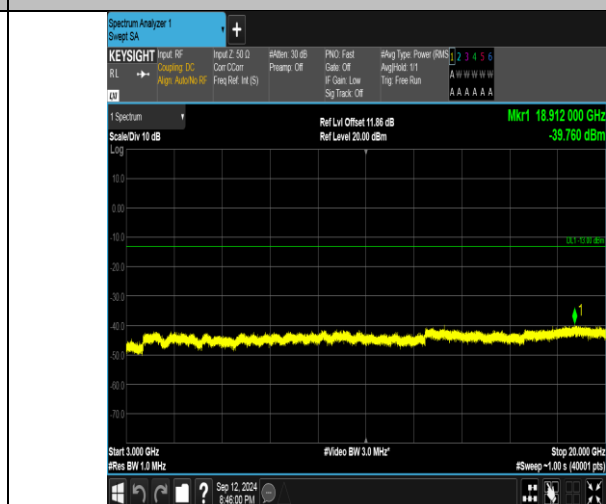
Band4_10MHz_16QAM_20175_50RB#0_3000~20000_3000~20000
