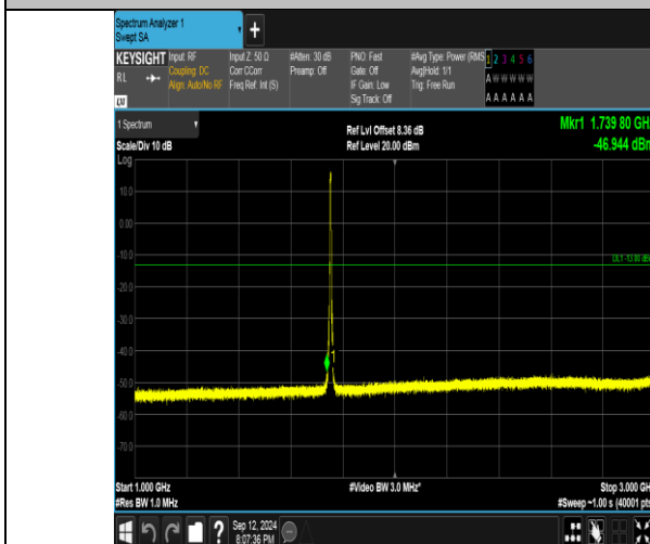
Band4_5MHz_16QAM_20375_25RB#0_1000~3000_1000~3000
