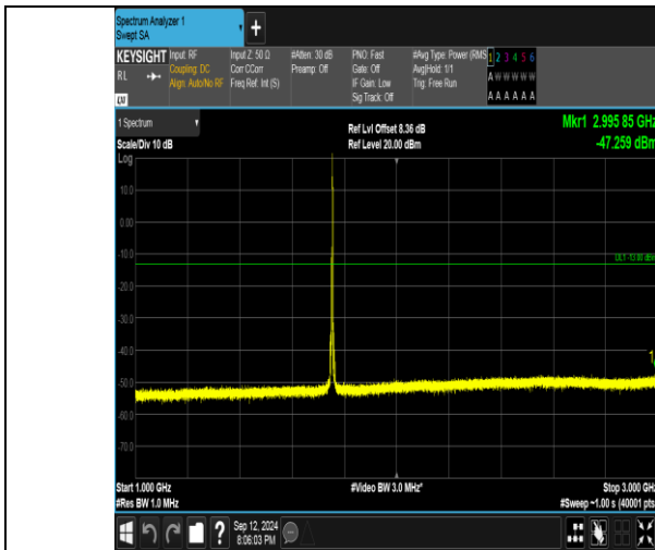
Band4_5MHz_16QAM_20375_1RB#24_1000~3000_1000~3000
