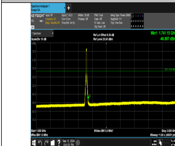
Band4_10MHz_16QAM_20000_50RB#0_1000~3000_1000~3000
