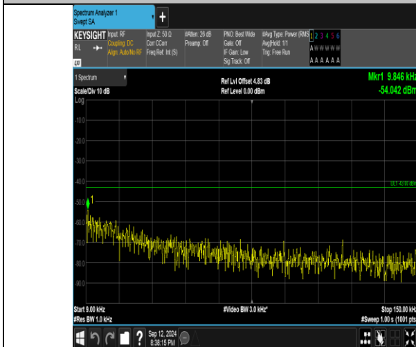
Band4_10MHz_QPSK_20000_1RB#49_0.009~0.15_0.009~0.15
