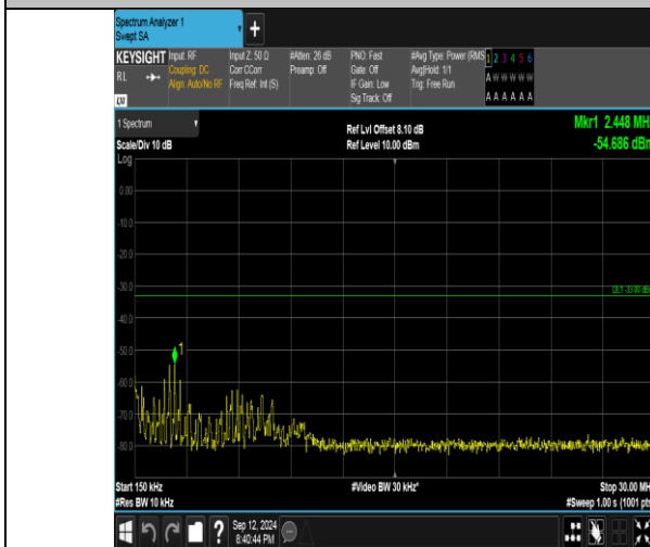
Band4_10MHz_16QAM_20000_50RB#0_0.15~30_0.15~30
