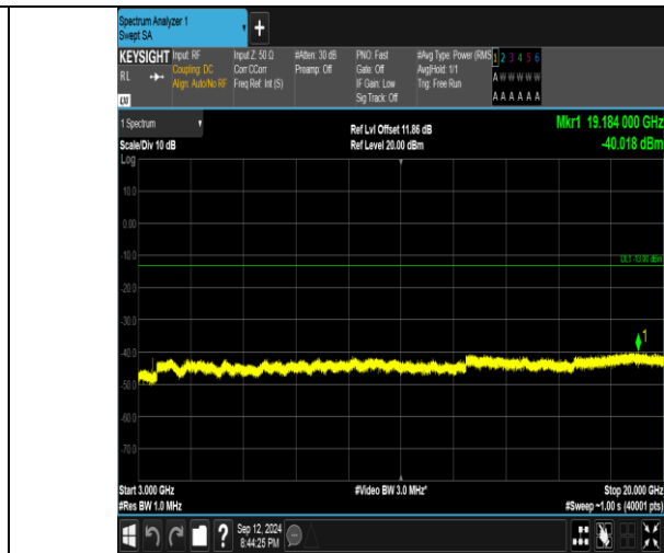
Band4_10MHz_16QAM_20175_1RB#49_3000~20000_3000~20000
