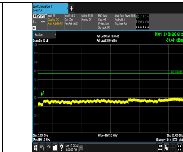
Band4_10MHz_16QAM_20000_1RB#49_3000~20000_3000~20000
