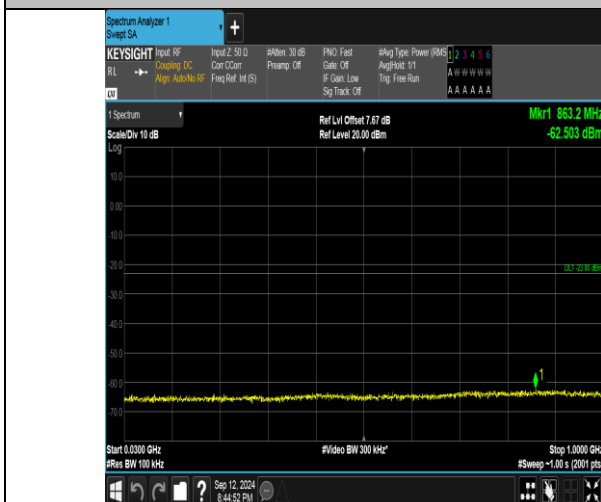
Band4_10MHz_QPSK_20175_50RB#0_30~1000_30~1000
