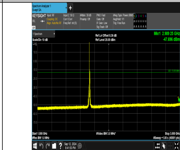
Band4_10MHz_QPSK_20175_1RB#0_1000-3000_1000-3000
