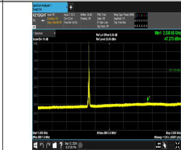
Band4_10MHz_QPSK_20000_1RB#0_1000~3000_1000~3000
