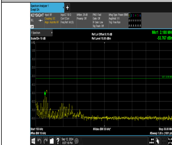
Band4_5MHz_16QAM_20375_25RB#0_0.15~30_0.15~30
