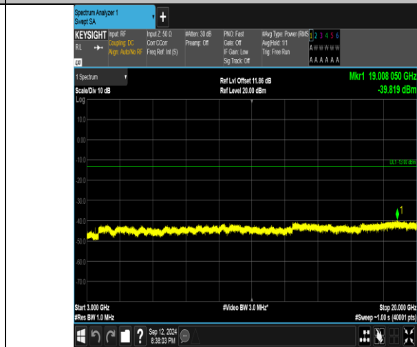
Band4_10MHz_16QAM_20000_1RB#0_3000~20000_3000~20000
