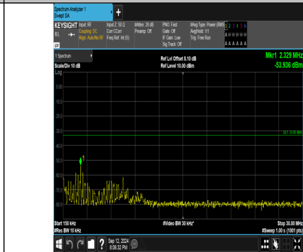
Band4_5MHz_QPSK_20375_25RB#0_0.15~30_0.15~30
