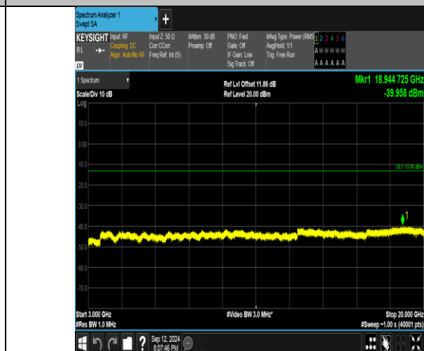
Band4_5MHz_16QAM_20375_25RB#0_3000~20000_3000~20000
