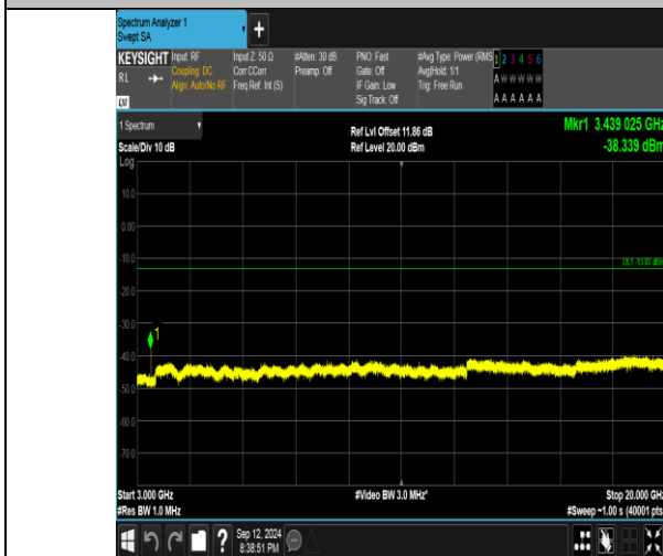
Band4_10MHz_QPSK_20000_1RB#49_3000~20000_3000~20000
