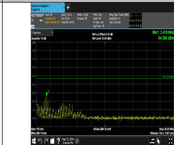
Band4_10MHz_QPSK_20175_50RB#0_0.15~30_0.15~30
