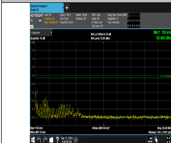
Band4_10MHz_16QAM_20000_1RB#49_0.15~30_0.15~30
