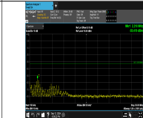
Band4_10MHz_QPSK_20000_1RB#49_0.15~30_0.15~30
