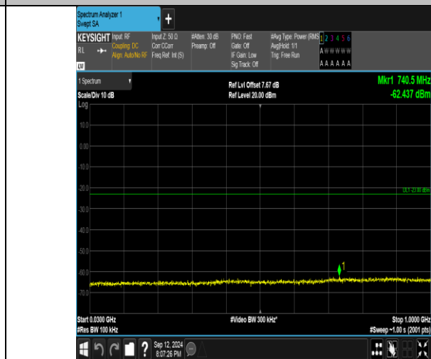
Band4_5MHz_16QAM_20375_25RB#0_30~1000_30~1000
