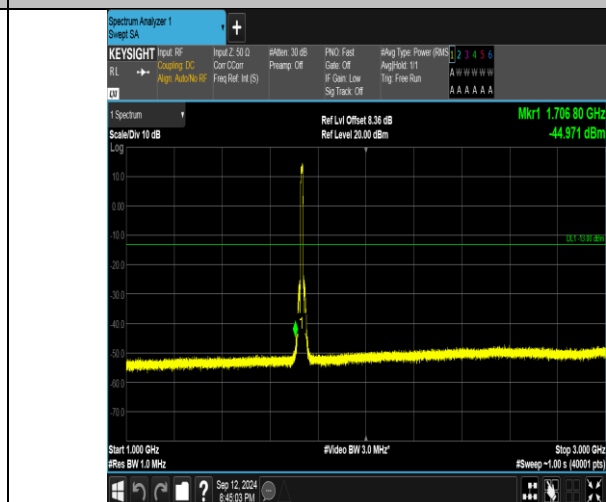
Band4_10MHz_QPSK_20175_50RB#0_1000~3000_1000~3000
