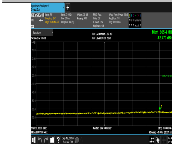
Band4_10MHz_QPSK_20175_1RB#0_30-1000_30-1000
