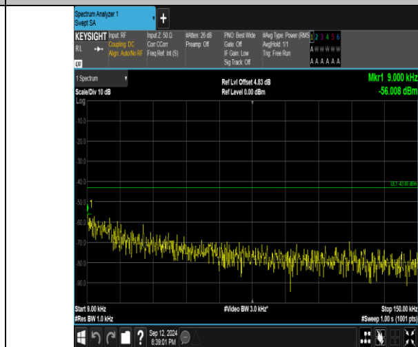
Band4_10MHz_16QAM_20000_1RB#49_0.009~0.15_0.009~0.15
