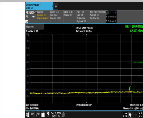
Band4_10MHz_16QAM_20000_50RB#0_30~1000_30~1000
