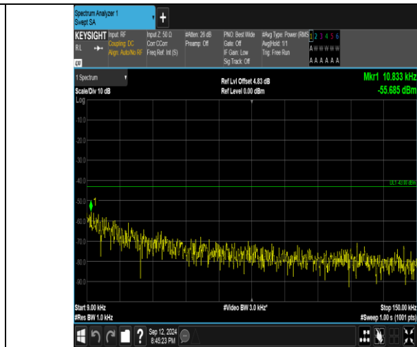
Band4_10MHz_16QAM_20175_50RB#0_0.009~0.15_0.009~0.15
