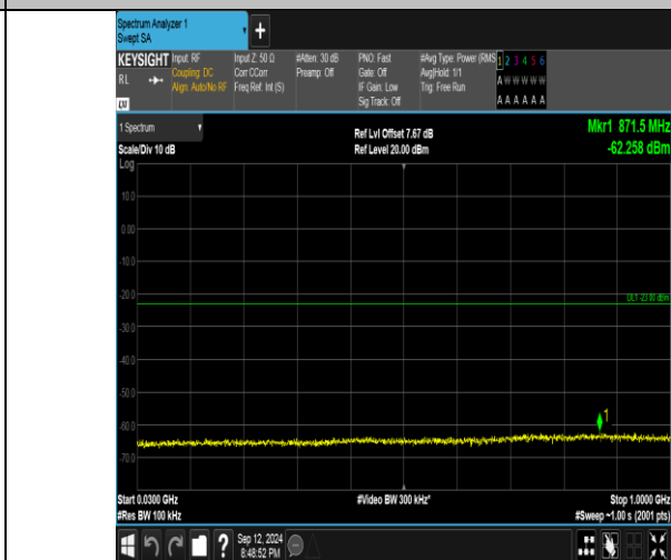
Band4_10MHz_16QAM_20350_1RB#49_30~1000_30~1000
