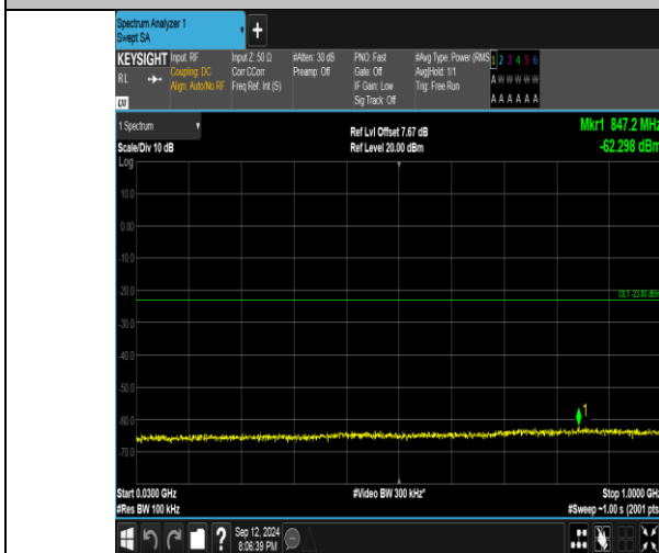
Band4_5MHz_QPSK_20375_25RB#0_30~1000_30~1000
