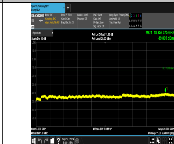
Band4_10MHz_16QAM_20000_50RB#0_3000~20000_3000~20000
