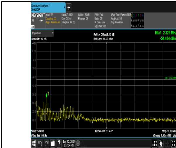
Band4_10MHz_16QAM_20000_1RB#0_0.15~30_0.15~30
