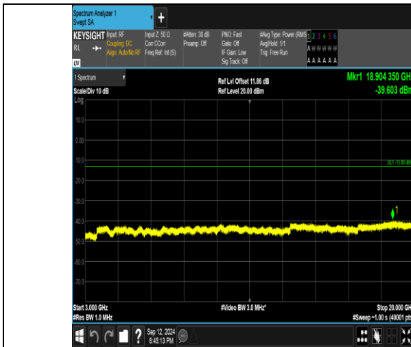
Band4_10MHz_QPSK_20175_50RB#0_3000~20000_3000~20000
