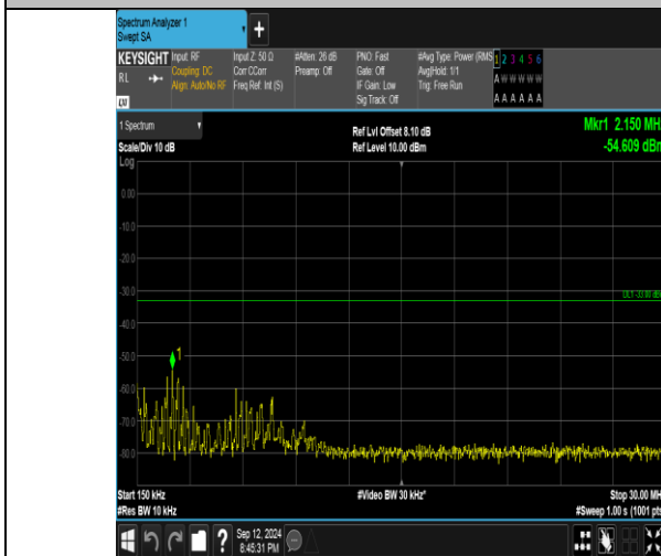
Band4_10MHz_16QAM_20175_50RB#0_0.15~30_0.15~30
