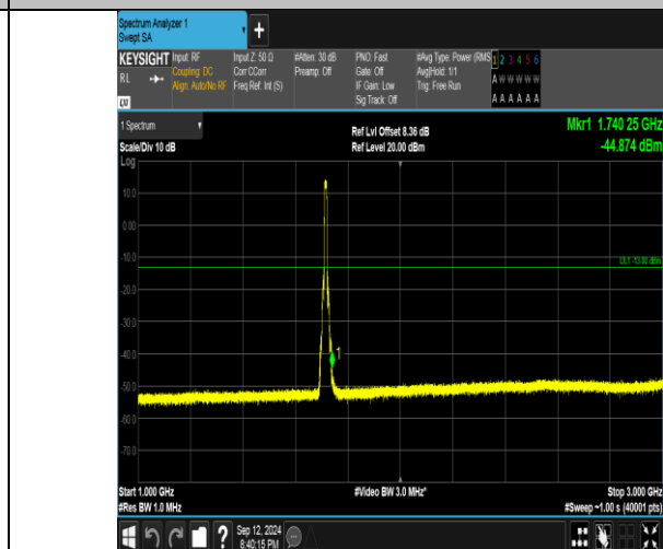
Band4_10MHz_QPSK_20000_50RB#0_1000~3000_1000~3000
