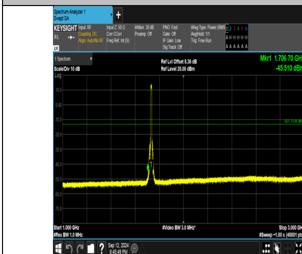
Band4_10MHz_16QAM_20175_50RB#0_1000~3000_1000~3000
