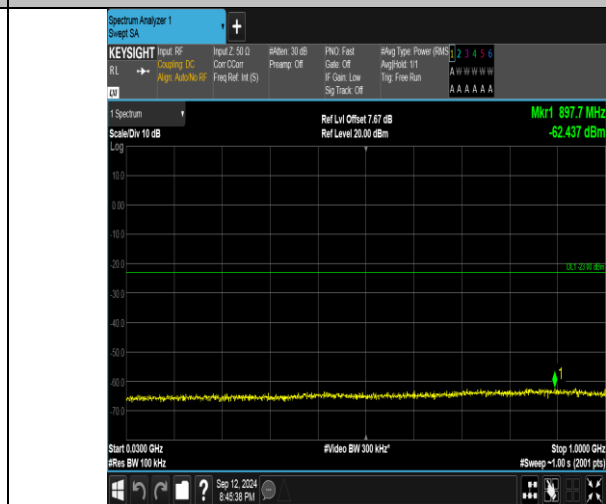
Band4_10MHz_16QAM_20175_50RB#0_30~1000_30~1000
