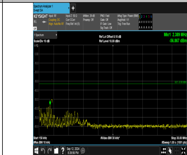
Band4_10MHz_QPSK_20000_50RB#0_0.15~30_0.15~30
