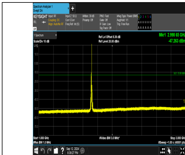
Band4_10MHz_16QAM_20000_1RB#49_1000~3000_1000~3000
