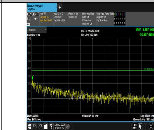
Band4_10MHz_16QAM_20350_1RB#49_0.009~0.15_0.009~0.15
