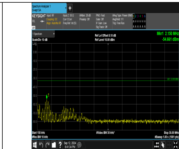
Band4_10MHz_QPSK_20175_1RB#0_0.15-30_0.15-30
