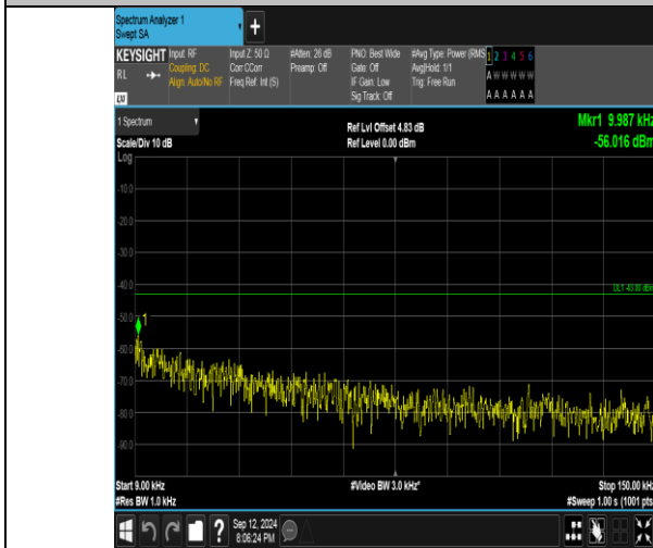
Band4_5MHz_QPSK_20375_25RB#0_0.009~0.15_0.009~0.15
