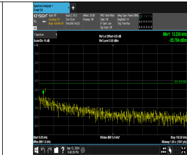
Band4_10MHz_16QAM_20000_50RB#0_0.009~0.15_0.009~0.15
