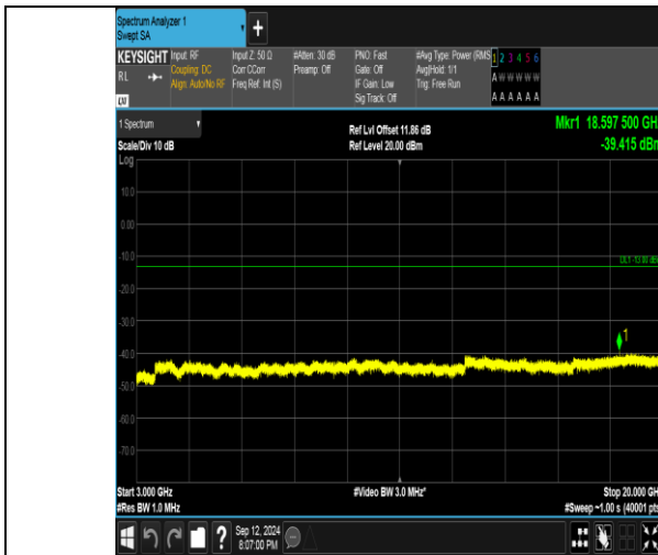
Band4_5MHz_QPSK_20375_25RB#0_3000~20000_3000~20000
