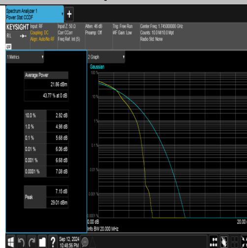
Band4-20MHz-16QAM-20300-1RB#0-PASS
