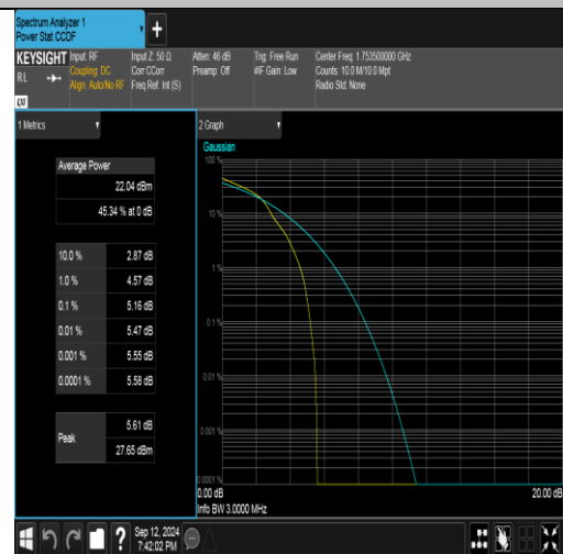
Band4-3MHz-16QAM-20385-1RB#0-PASS
