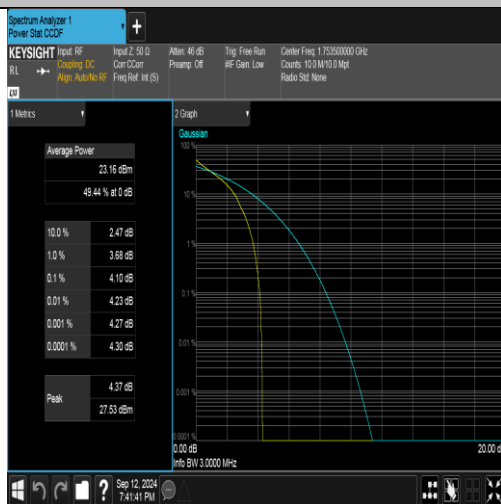
Band4-3MHz-QPSK-20385-1RB#0-PASS
