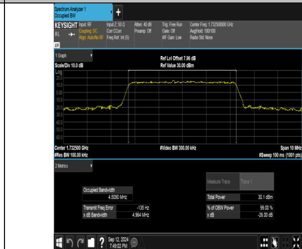
Band4-5MHz-16QAM-20175-25RB#0-PASS
