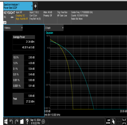
Band4-10MHz-16QAM-20000-50RB#0-PASS
