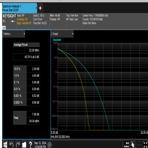
Band4-20MHz-QPSK-20300-100RB#0-PASS
