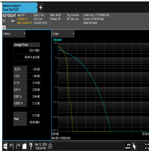
Band4-15MHz-QPSK-20025-1RB#0-PASS
