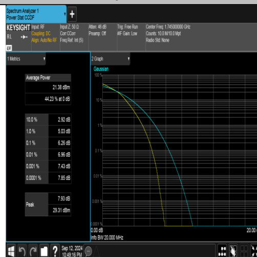
Band4-20MHz-16QAM-20300-100RB#0-PASS
