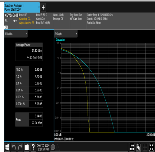
Band4-5MHz-16QAM-20375-1RB#0-PASS
