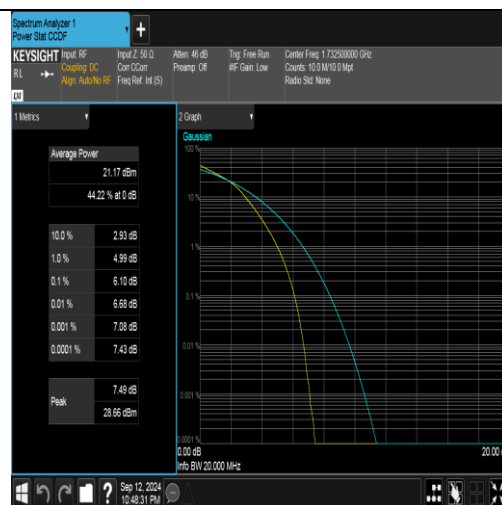
Band4-20MHz-16QAM-20175-100RB#0-PASS
