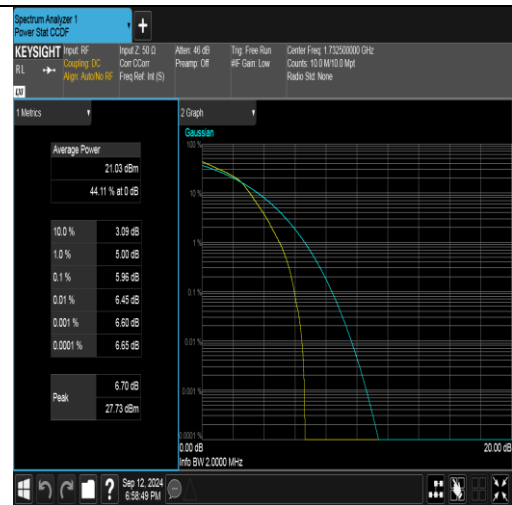
Band4-1.4MHz-16QAM-20175-6RB#0-PASS
