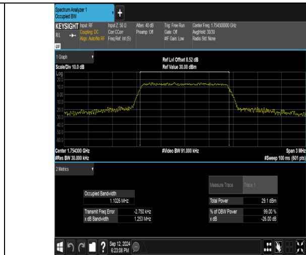
Band4-1.4MHz-16QAM-20393-6RB#0-PASS
