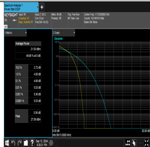
Band4-5MHz-16QAM-19975-25RB#0-PASS
