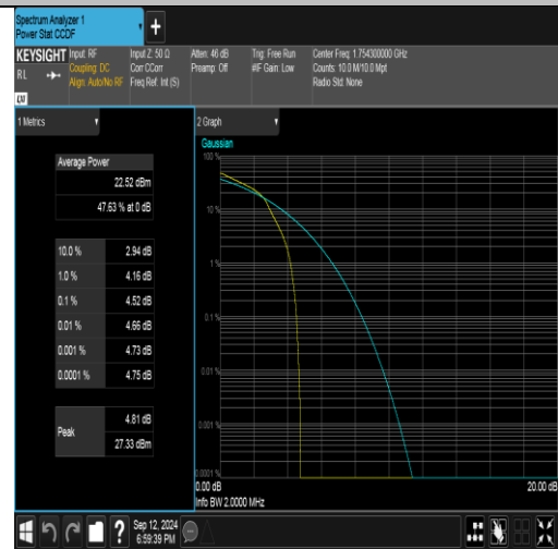
Band4-1.4MHz-16QAM-20393-1RB#0-PASS
