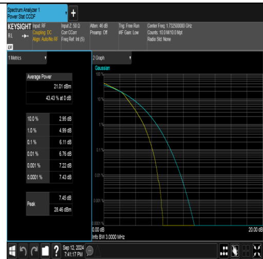
Band4-3MHz-16QAM-20175-15RB#0-PASS
