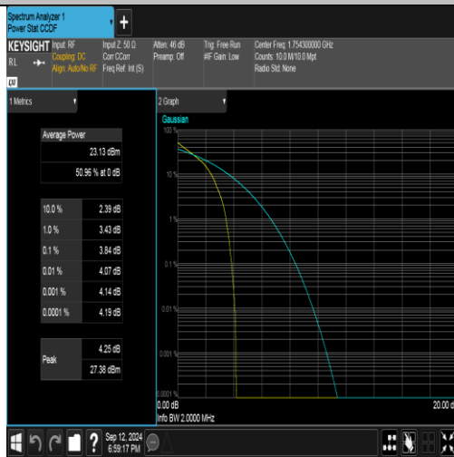
Band4-1.4MHz-QPSK-20393-1RB#0-PASS
