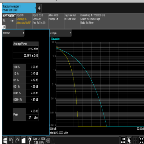
Band4-3MHz-QPSK-19965-15RB#0-PASS
