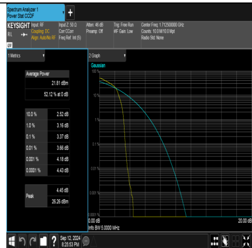
Band4-5MHz-16QAM-19975-1RB#0-PASS
