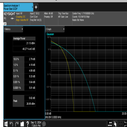
Band4-3MHz-16QAM-19965-15RB#0-PASS
