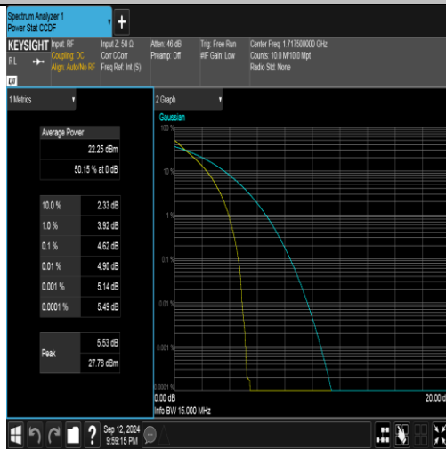
Band4-15MHz-QPSK-20025-75RB#0-PASS
