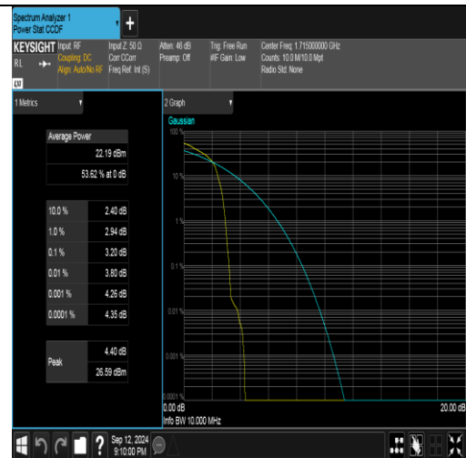
Band4-10MHz-16QAM-20000-1RB#0-PASS
