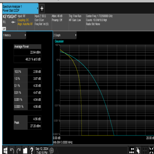
Band4-3MHz-QPSK-20175-1RB#0-PASS
