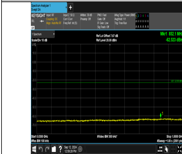
Band2_5MHz_QPSK_18900_1RB#0_30~1000_30~1000
