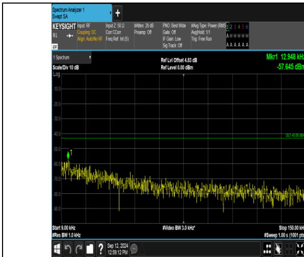
Band2_5MHz_QPSK_18900_1RB#0_0.009~0.15_0.009~0.15
