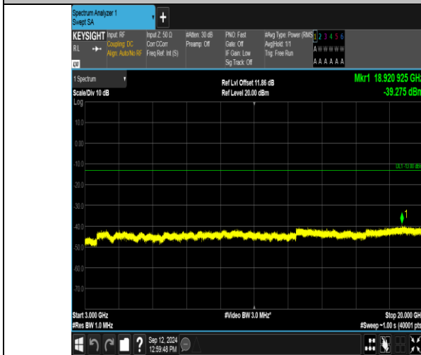
Band2_5MHz_QPSK_18900_1RB#0_3000~20000_3000~20000
