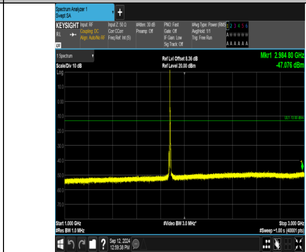
Band2_5MHz_QPSK_18900_1RB#0_1000~3000_1000~3000
