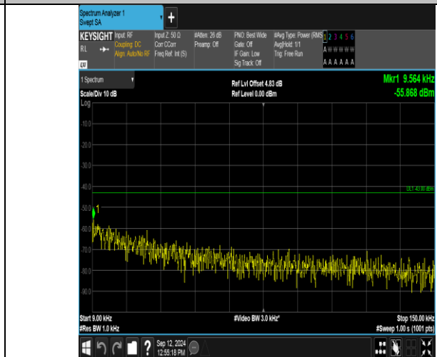
Band2_5MHz_16QAM_18625_1RB#0_0.009~0.15_0.009~0.15
