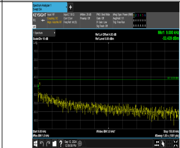
Band2_5MHz_16QAM_18900_1RB#0_0.009~0.15_0.009~0.15
