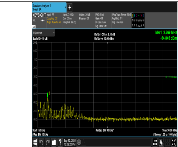
Band2_5MHz_QPSK_18900_1RB#0_0.15~30_0.15~30
