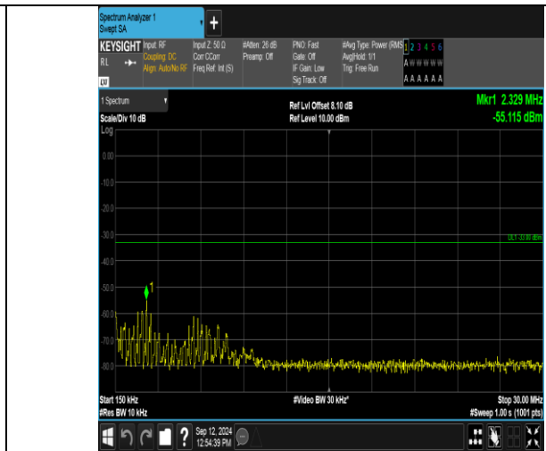
Band2_5MHz_QPSK_18625_1RB#0_0.15~30_0.15~30
