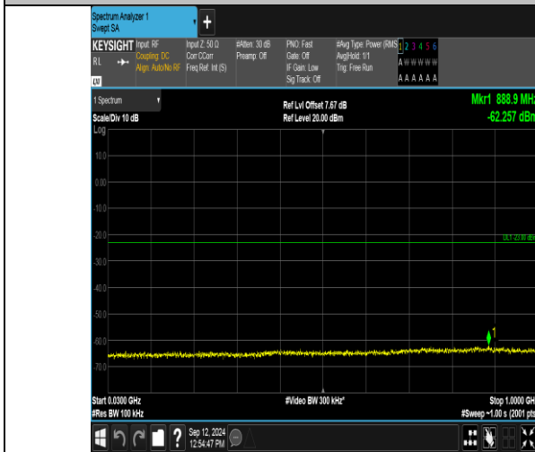
Band2_5MHz_QPSK_18625_1RB#0_30~1000_30~1000
