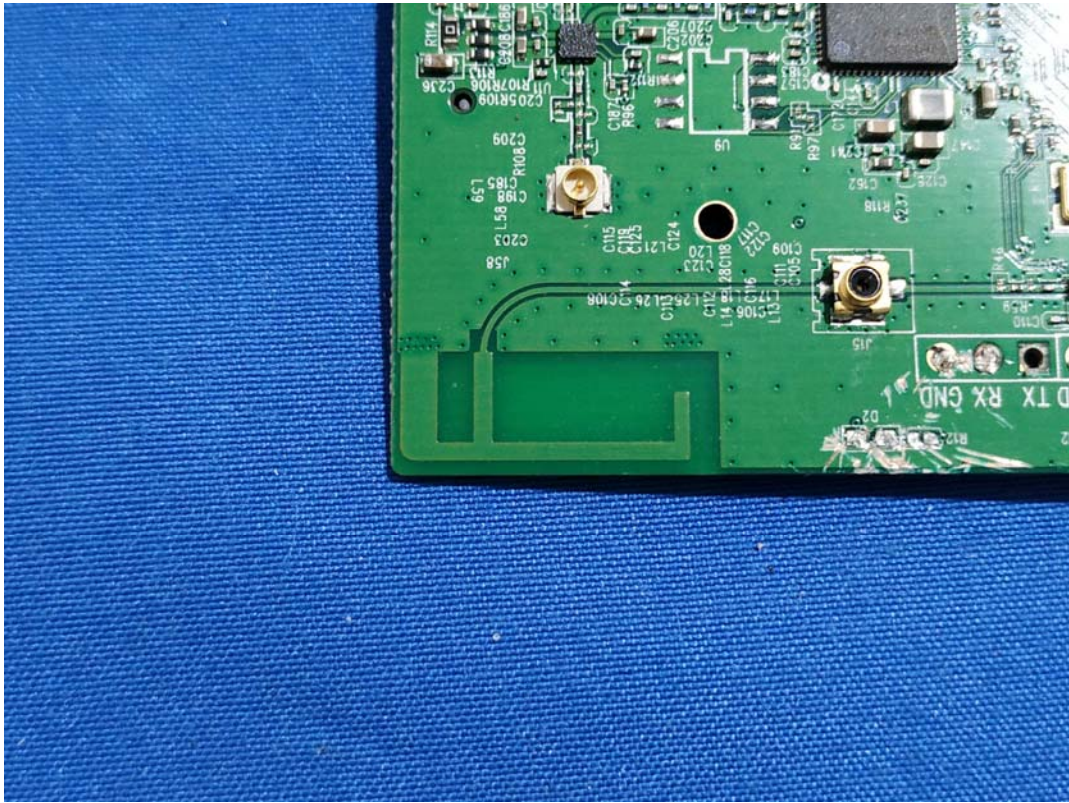
2.4G Wi-Fi Chain 1
