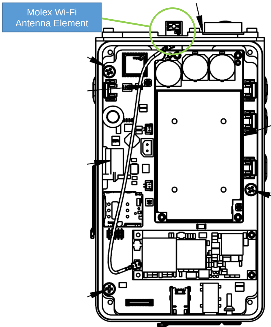
SHOUT sp Assembly instruction diagram showing Wi-Fi cable routing
