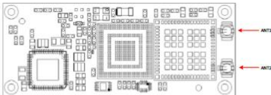
Image from Variscite DART SoM Integrators Guide with Antenna Ports
