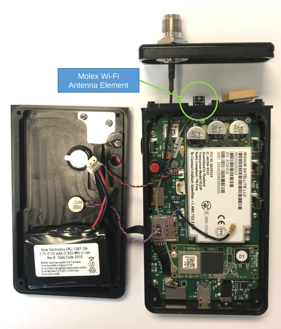
SHOUT sp Internal Views – Radome Removed
