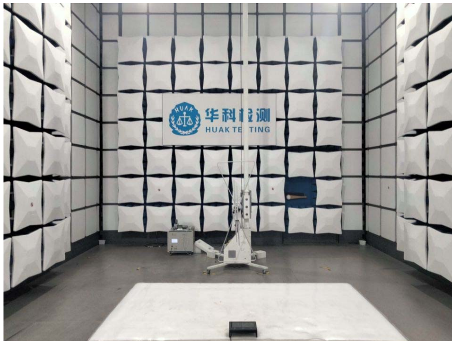
Model: CTR69Q Radiated Emissions
