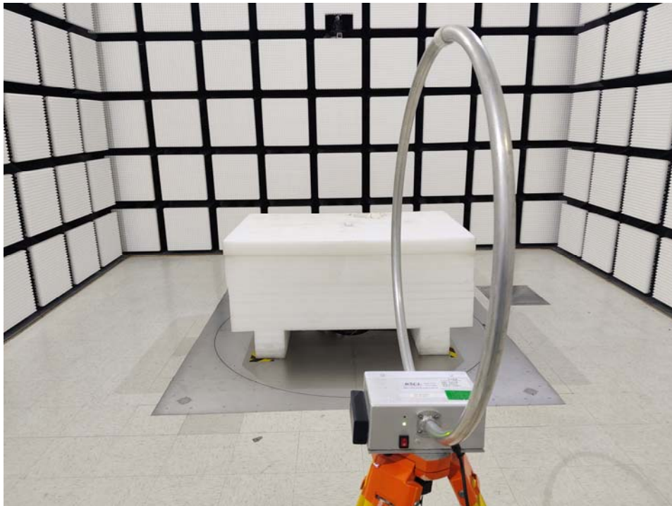
Radiated Emission 9 kHz-30 MHz Ground-parallel View
