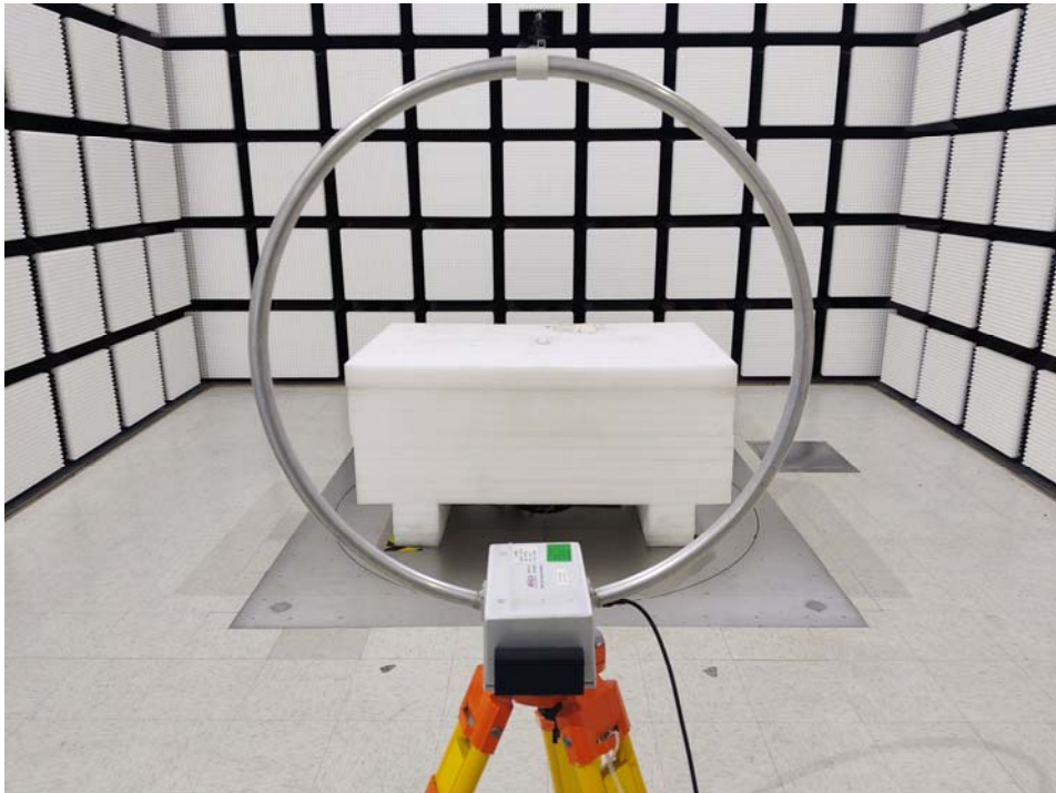
Radiated Emission 9 kHz-30 MHz Parallel View
