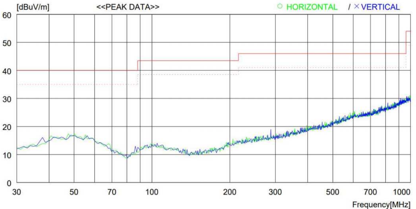
Graphical Test Data – Below 1 GHz – Middle Channel (Peak)
