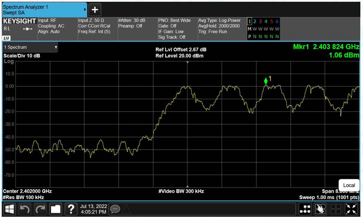
Band Edge(Hopping) NVNT user 2402MHz Ant1 Hopping Emission
