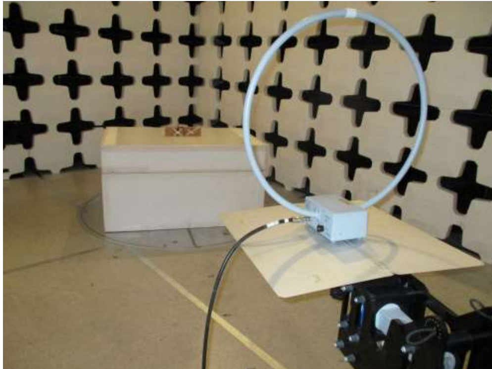
Figure 2. Radiated Emissions Test Configuration (below 30 MHz)
