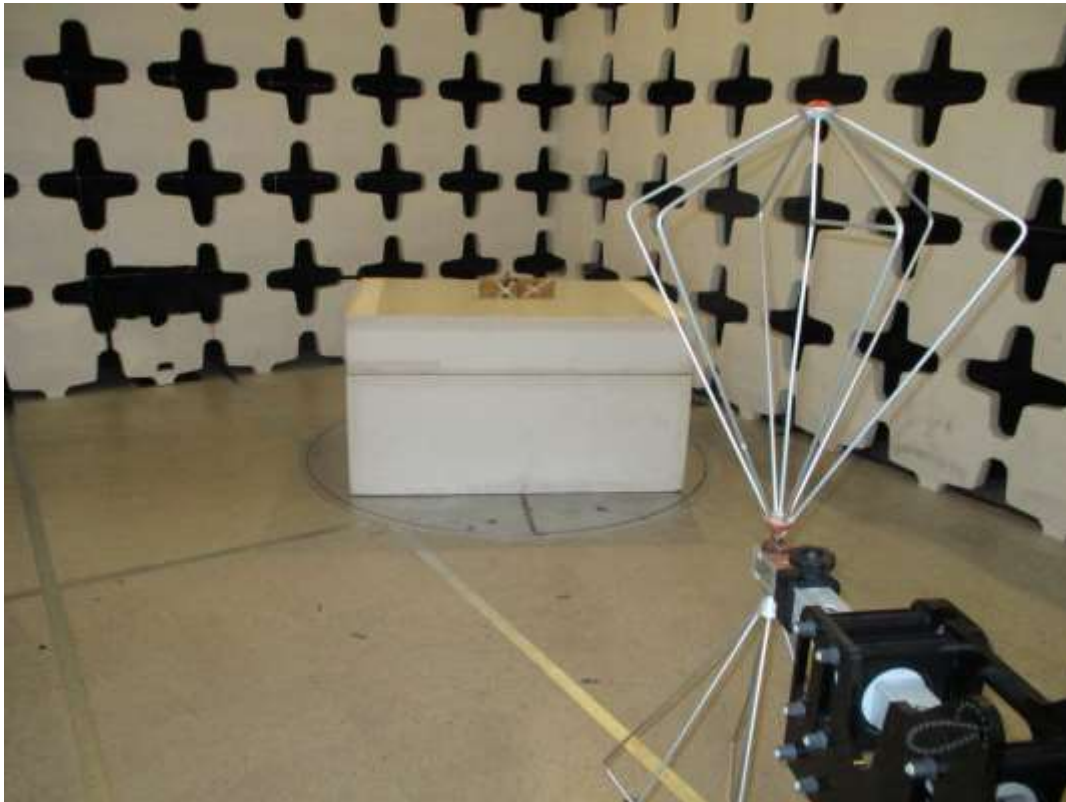
Figure 2. Radiated Emissions Test Configuration (30 - 200 MHz)
