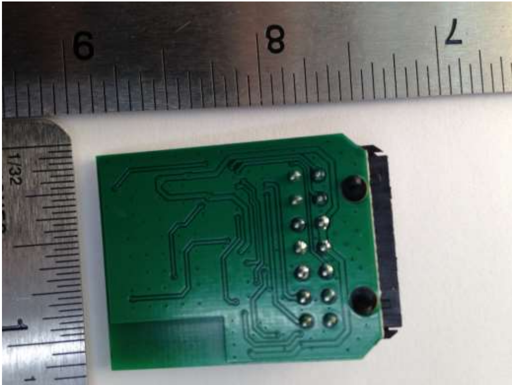
Figure 2. PCB, Solder Side
