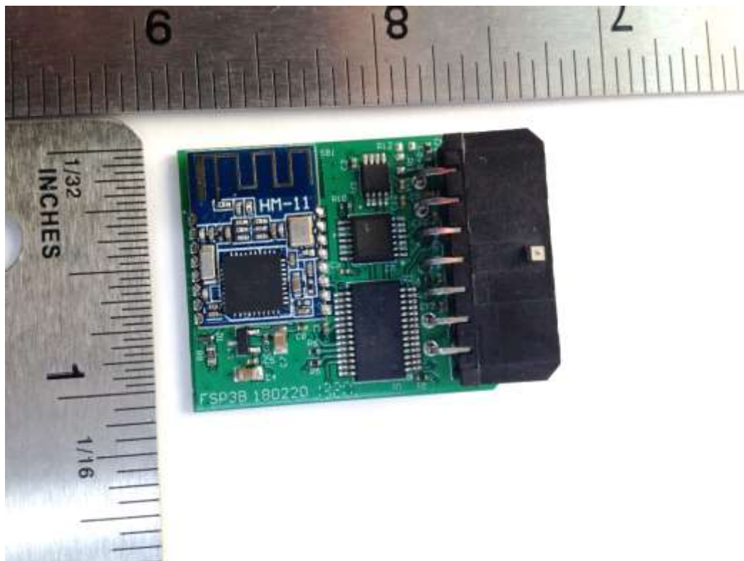
Figure 1. PCB, Component Side
