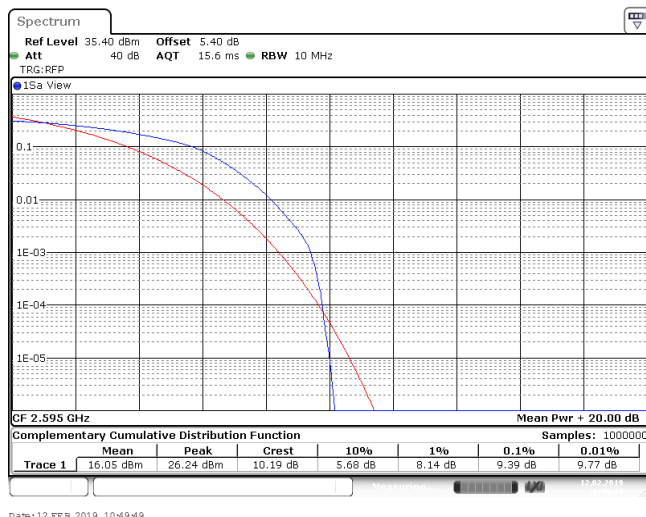
Band38_20MHz_16QAM_38150_100RB#0
