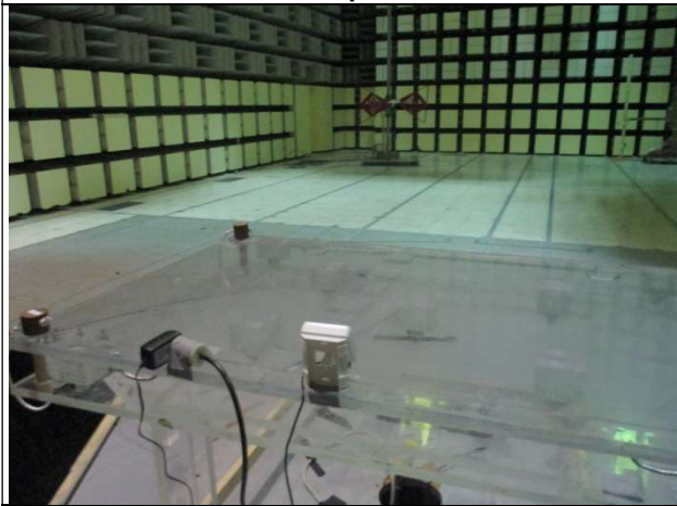
RE Test Setup – 30MHz – 1GHz
