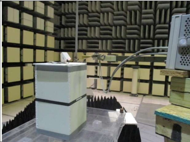
RE Test Setup – 40GHz – 50GHz
