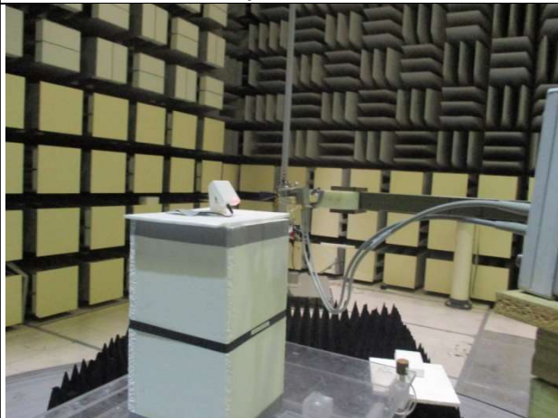
RE Test Setup – 50GHz – 75GHz
