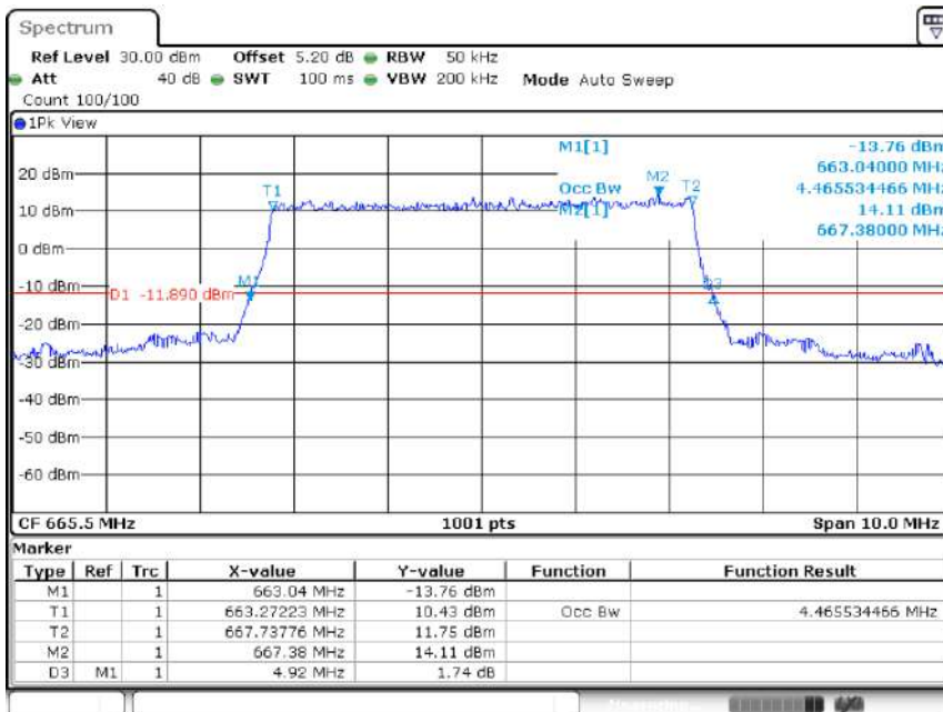
Band71-5MHz-QPSK-133147-25RB#0-4.466
