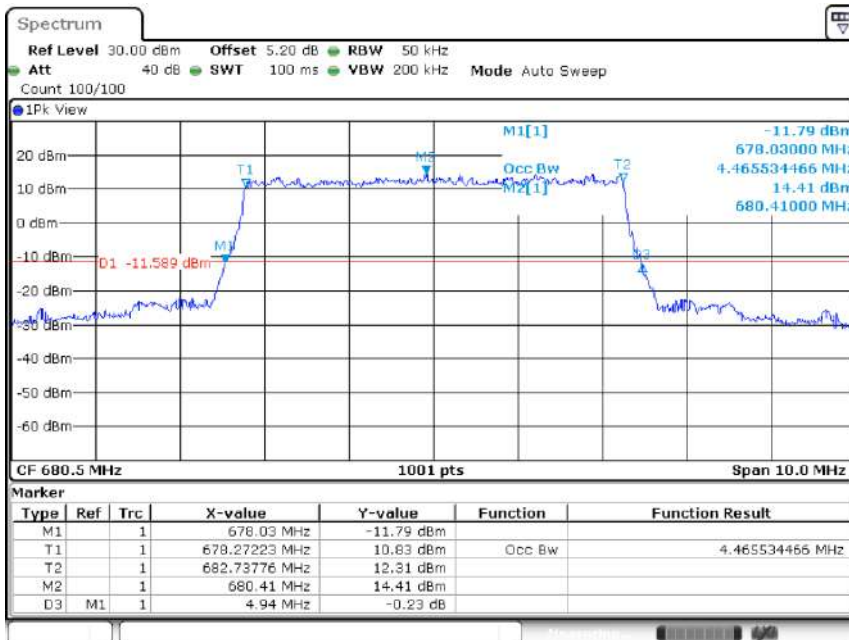
Band71-5MHz-QPSK-133297-25RB#0-4.466
