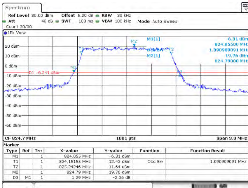
Band26-1.4MHz-QPSK-26797-6RB#0-1.091
