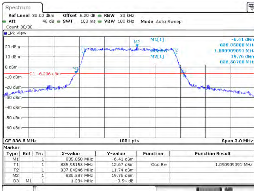
Band26-1.4MHz-QPSK-26915-6RB#0-1.091
