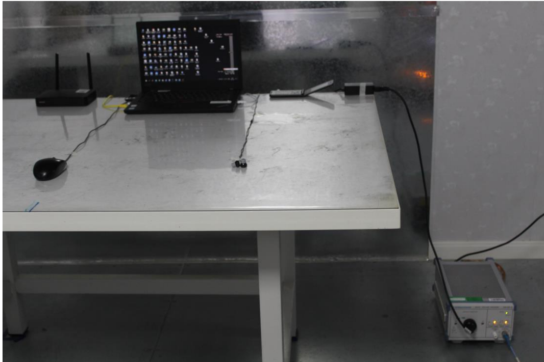
Radiated Emissions Test Setup
