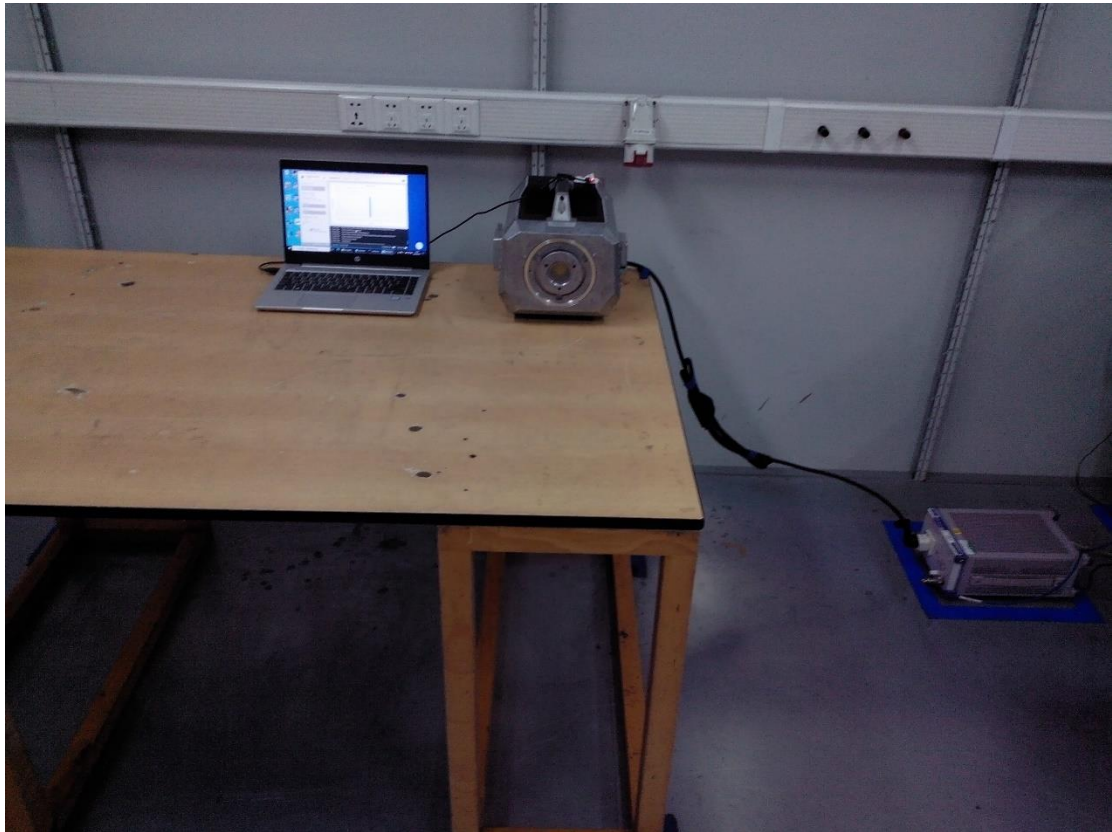
AC Conducted Emission Test Setup -Front
