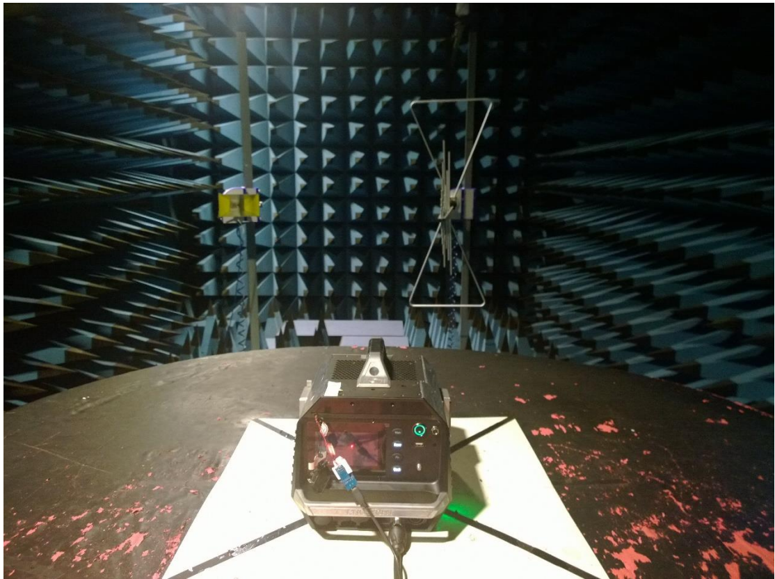
FCC Part15C Radiated Emission above 1-18GHz
