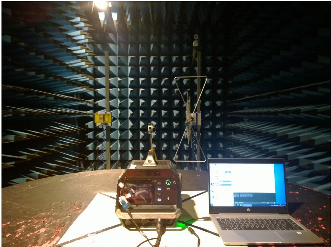
FCC Part15C Radiated Emission above 18-25GHz
