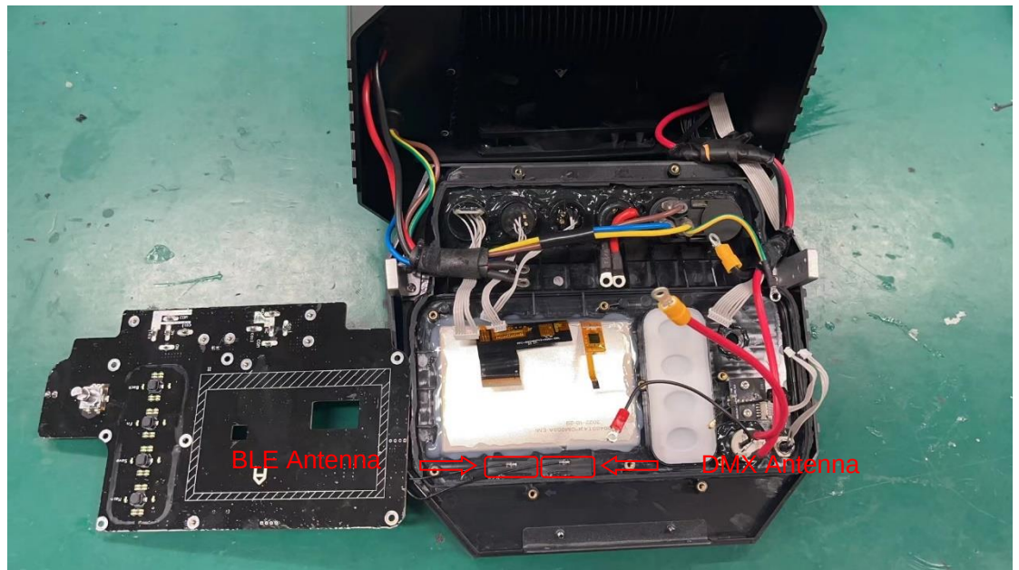
Photo 5 Inside of EUT
