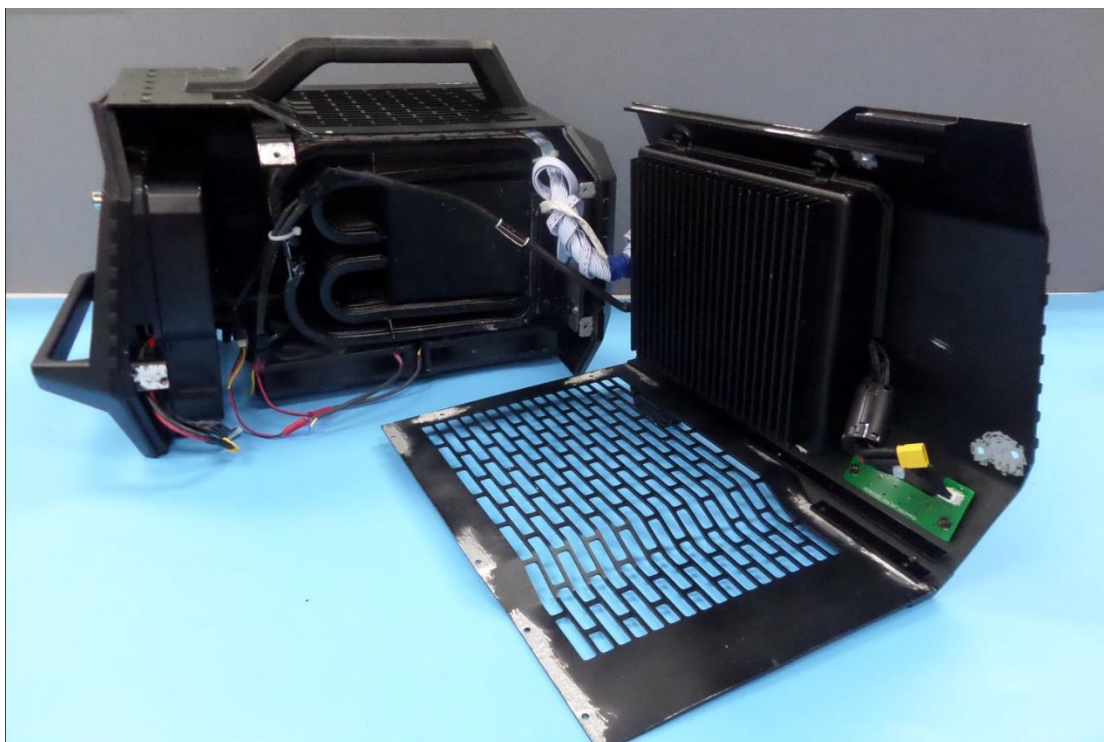
Photo 2 Inside of EUT
