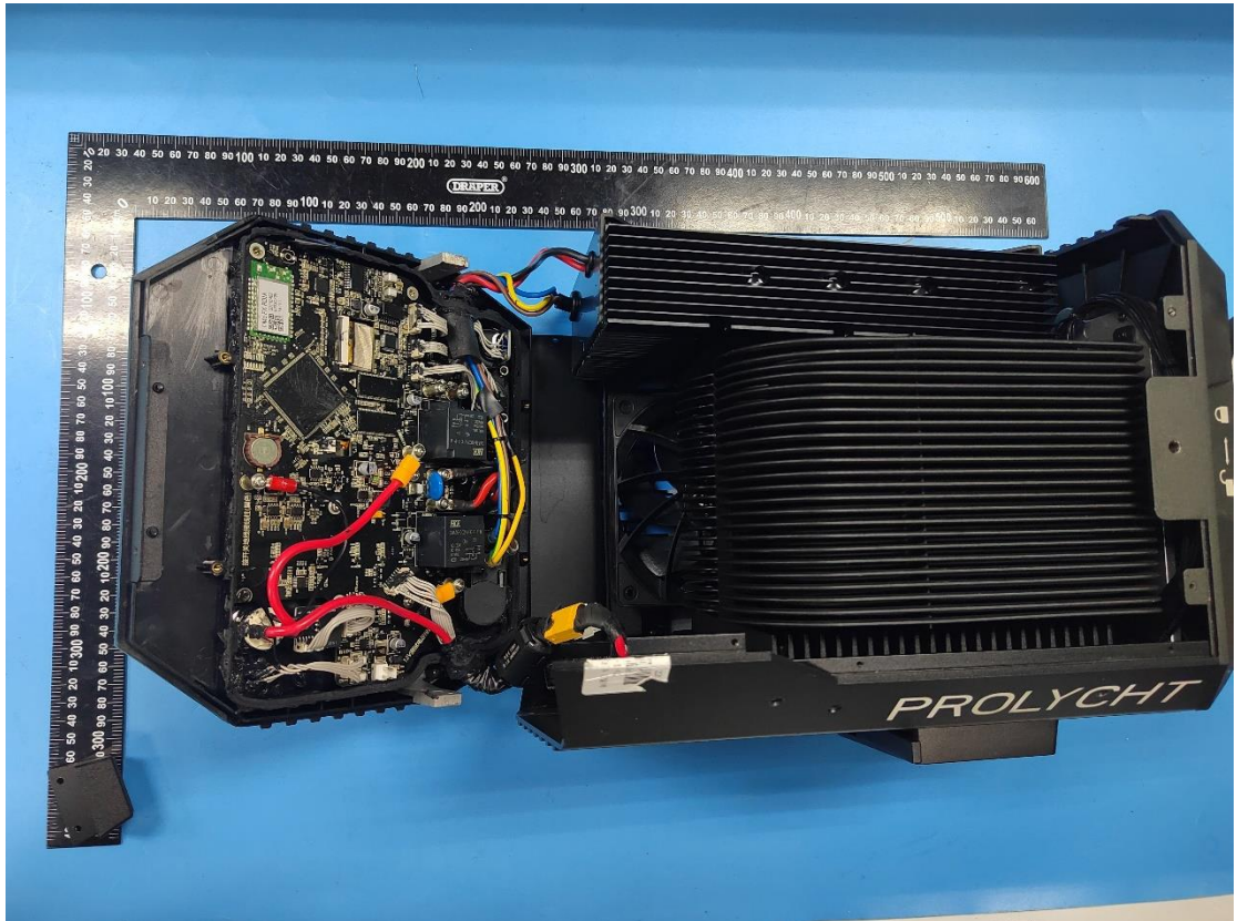
Photo 4 Inside of EUT
