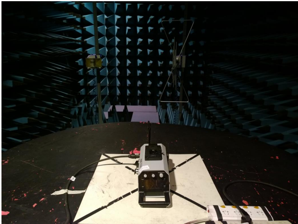
FCC Part15C Radiated Emission above 1-18GHz -Front
