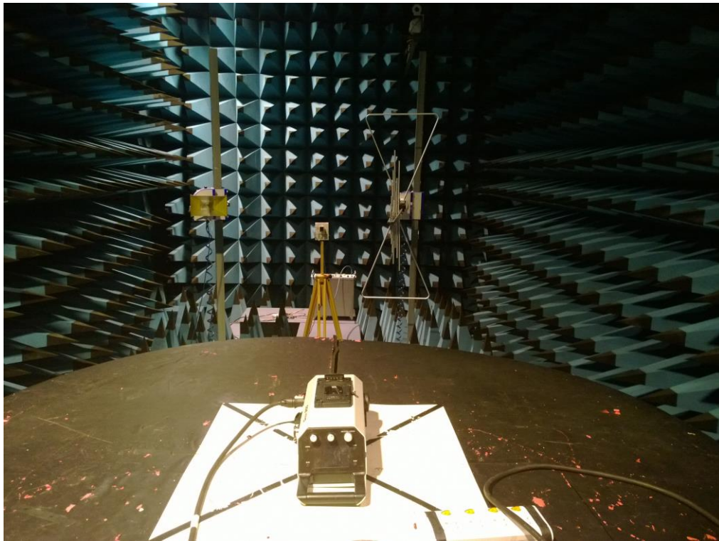
FCC Part15C Radiated Emission above 18-25GHz -Front
