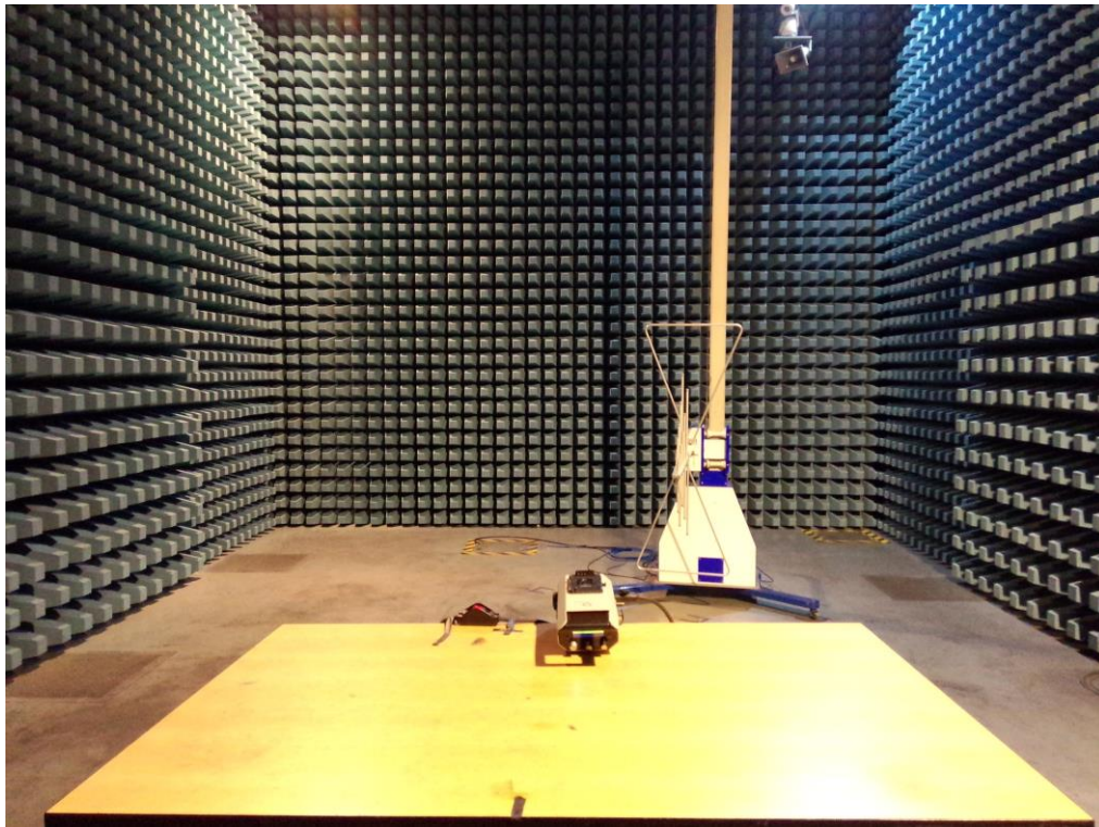
FCC Part15C Radiated Emission below 1GHz -Front
