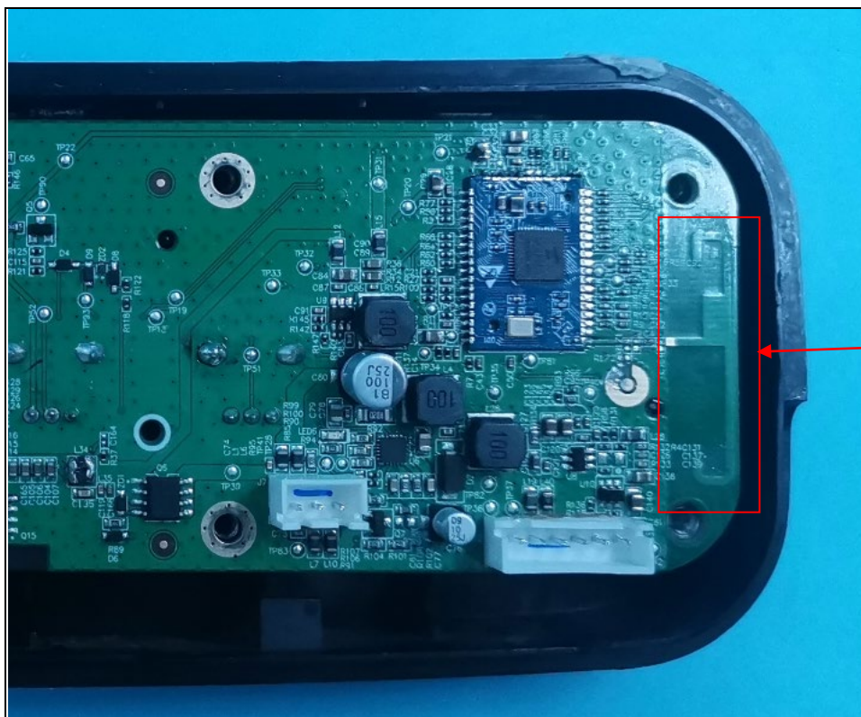
BT Antenna
