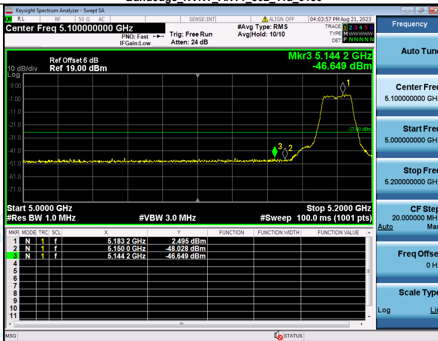
Bandedge_NVNT_ANT1_802_11a_5180
