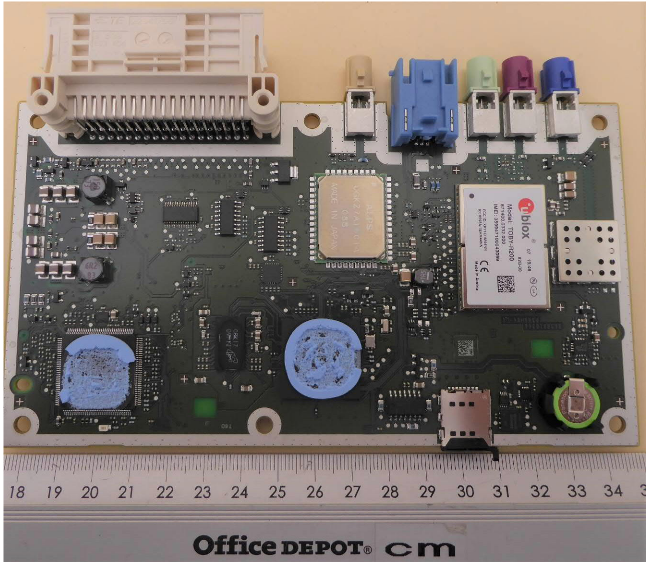
Main PCB – top view
