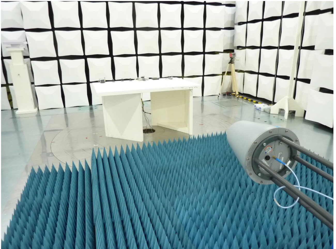
Test setup semi anechoic chamber 1 GHz – 13 GHz
