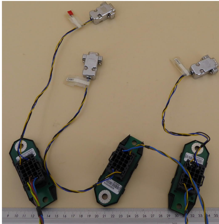
Sensors for CAN simulation
