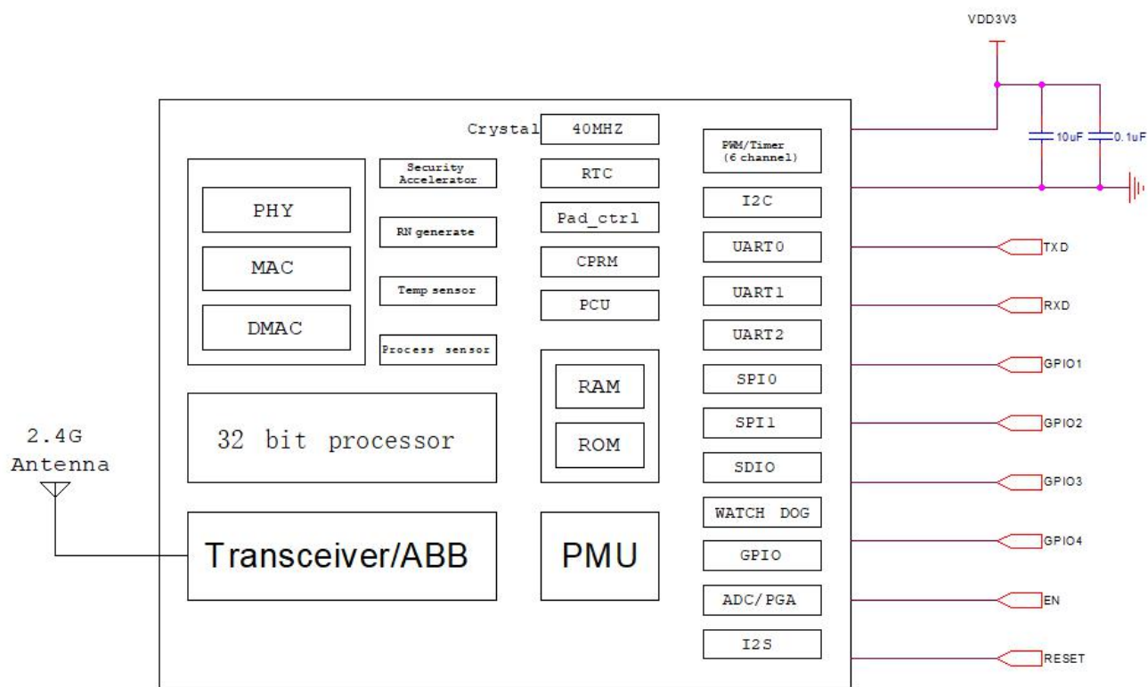
LA-WE2S Wi-Fi Module functional block diagram
