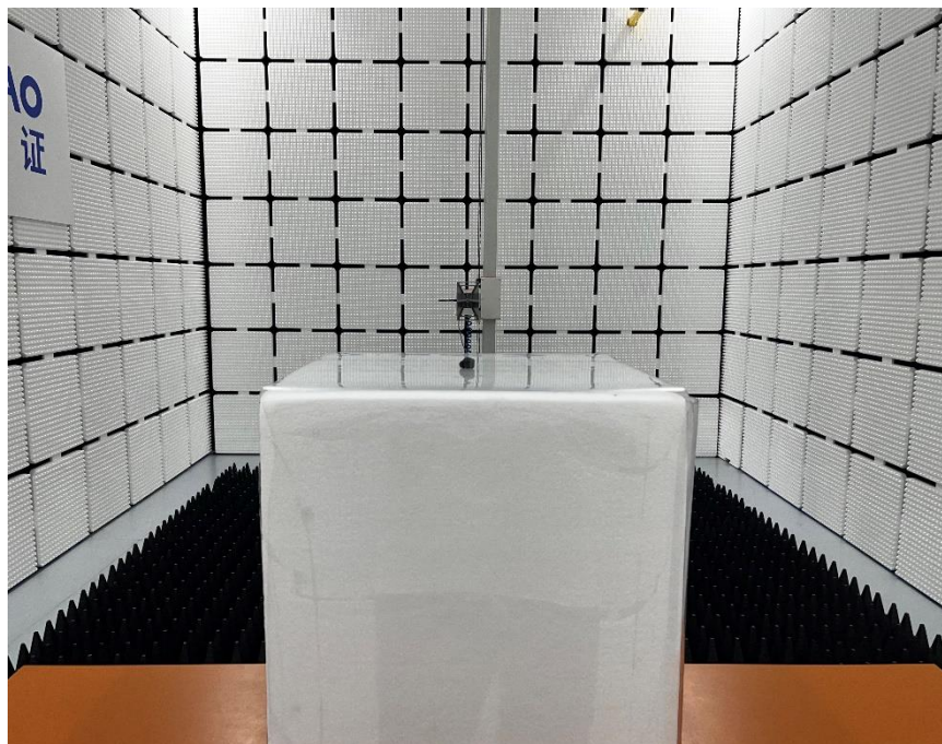
Radiated Emission Above 1GHz (Right ear)
