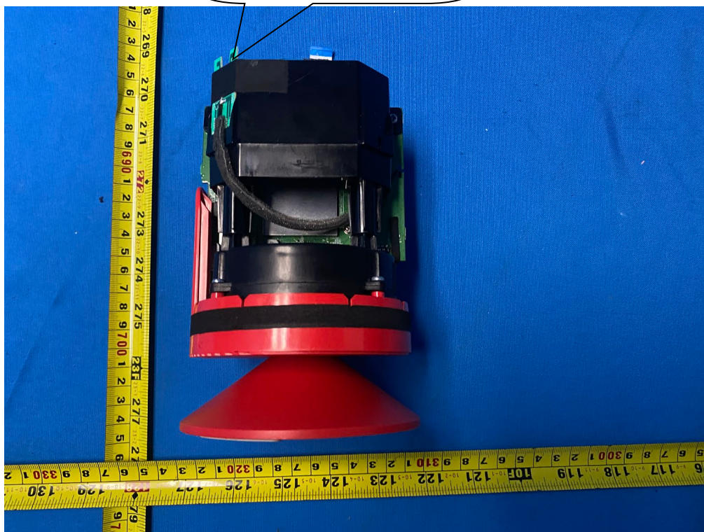
2.4G & 5G Antenna 2
