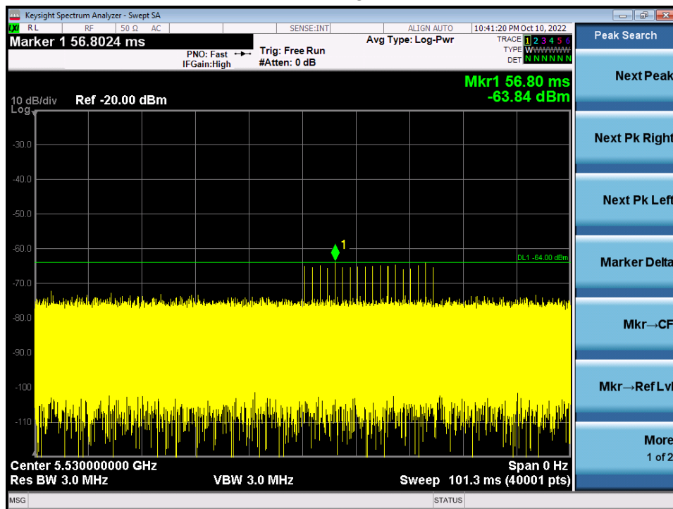
Radar Signal 0
