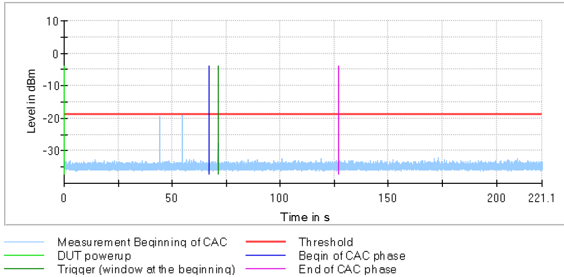
Beginning of CAC; Radar Pulses
