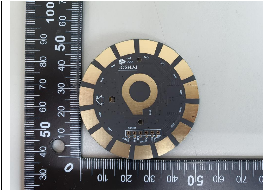
Touch Board Front
