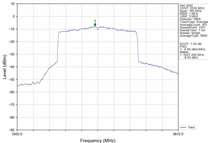
802.11ax(HEW80)_LCH_5530MHz_SU_ / _Ant2_NTNV
