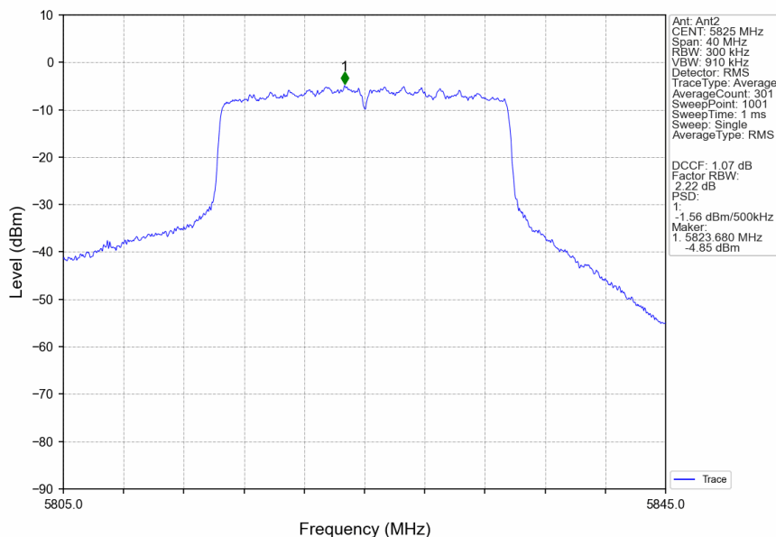
802.11ax(HEW20)_HCH_5825MHz_SU_ / _Ant2_NTNV
