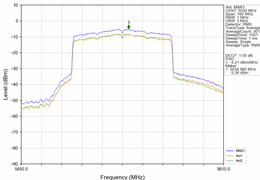
802.11ax(HEW80)_LCH_5530MHz_SU_/_MIMO_NTNV
