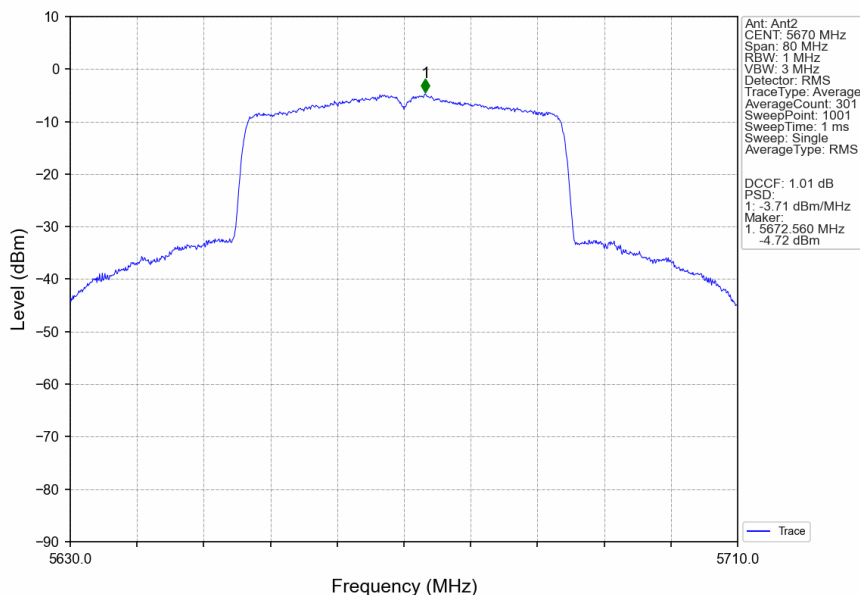
802.11ax(HEW40)_HCH_5670MHz_SU_/_Ant2_NTNV
