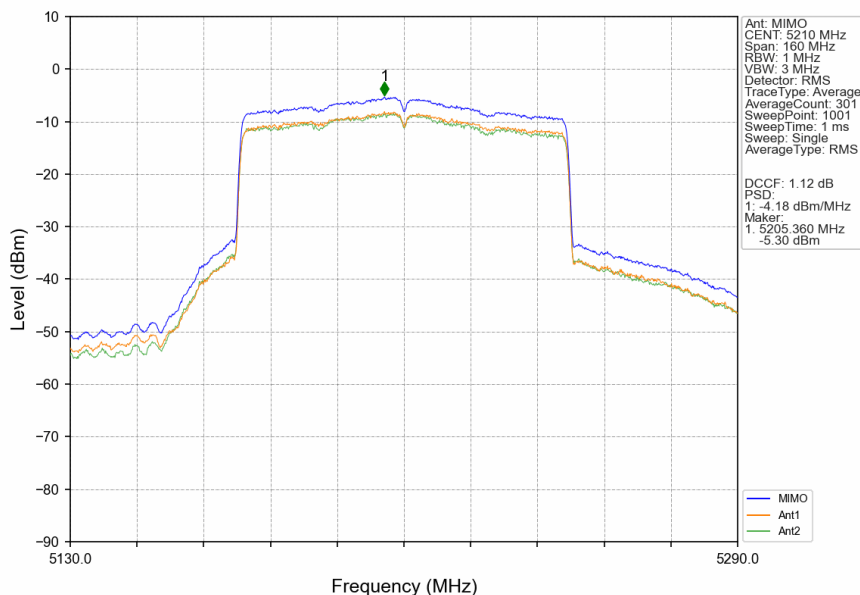
802.11ax(HEW80)_MCH_5210MHz_SU_/_MIMO_NTNV
