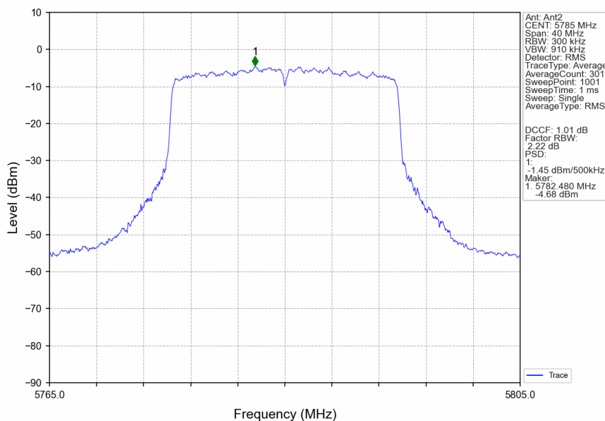
802.11ax(HEW20)_MCH_5785MHz_SU_ / _Ant2_NTNV
