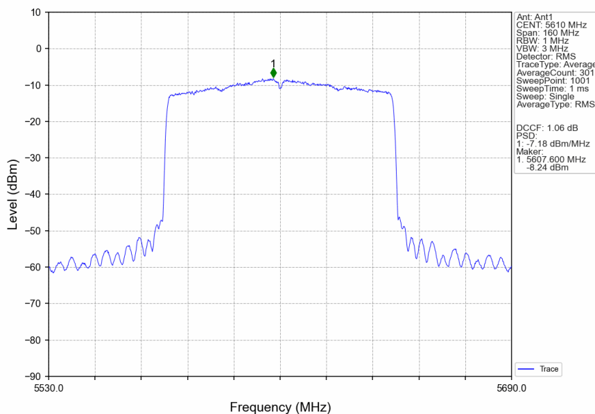
802.11ax(HEW80)_HCH_5610MHz_SU_/_Ant1_NTNV
