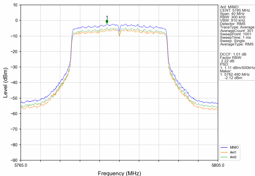
802.11ax(HEW20)_MCH_5785MHz_SU_/_MIMO_NTNV
