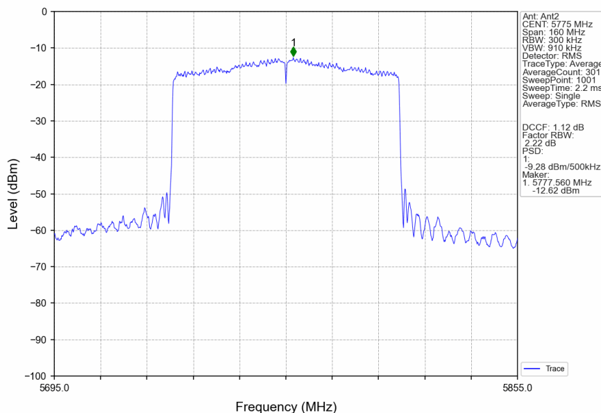
802.11ax(HEW80)_MCH_5775MHz_SU_ / _Ant2_NTNV
