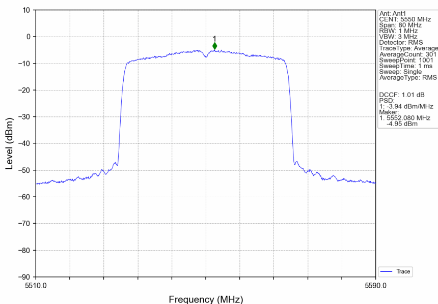
802.11ax(HEW40)_MCH_5550MHz_SU_ / _Ant1_NTNV
