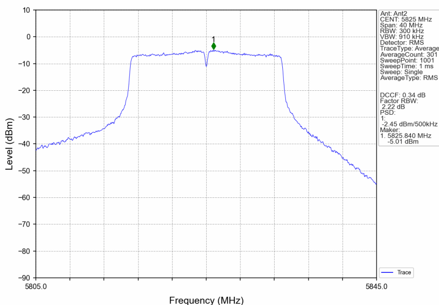
802.11ac(VHT20)_HCH_5825MHz_Ant2_NTNV
