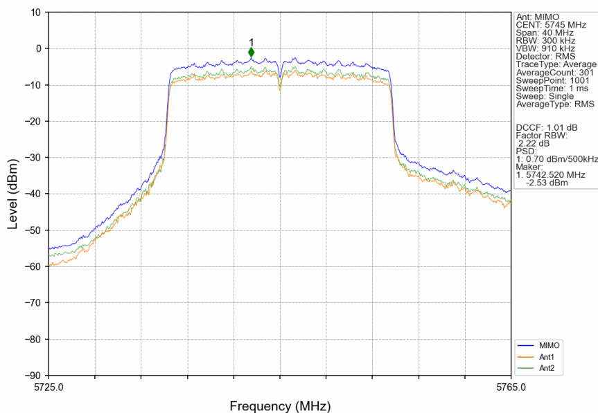
802.11ax(HEW20)_LCH_5745MHz_SU_ / _MIMO_NTNV
