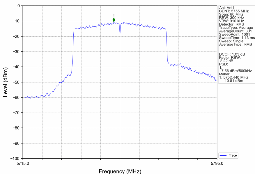
802.11ax(HEW40)_LCH_5755MHz_SU_ / _Ant1_NTNV
