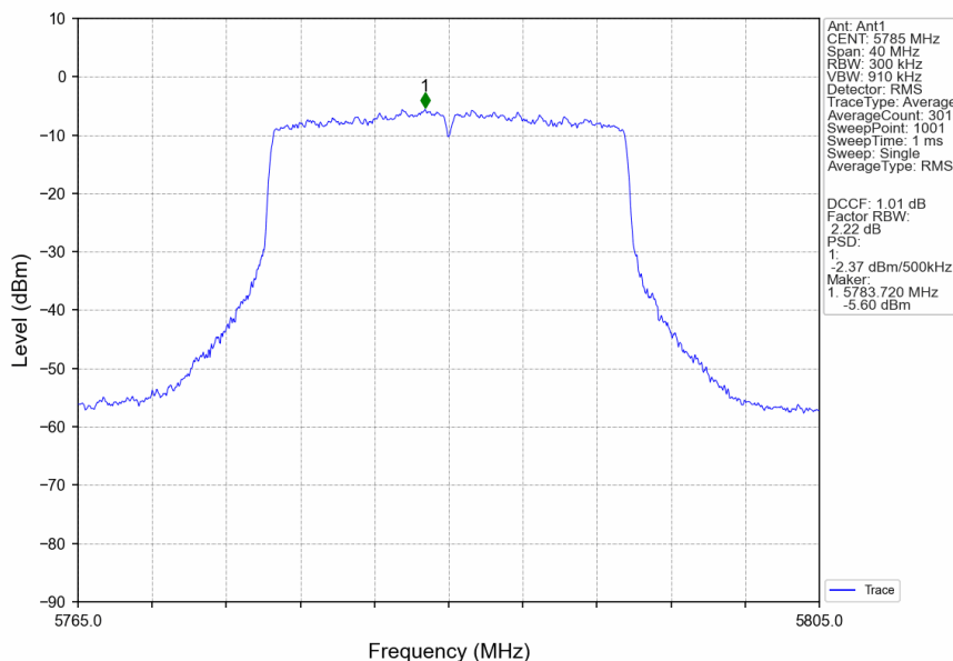
802.11ax(HEW20)_MCH_5785MHz_SU_ / _Ant1_NTNV
