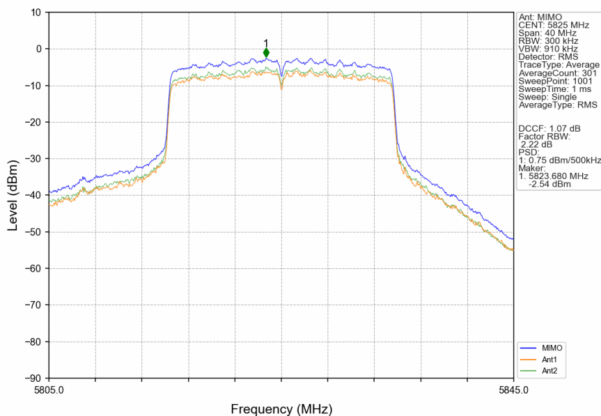
802.11ax(HEW20)_HCH_5825MHz_SU_ / _MIMO_NTNV
