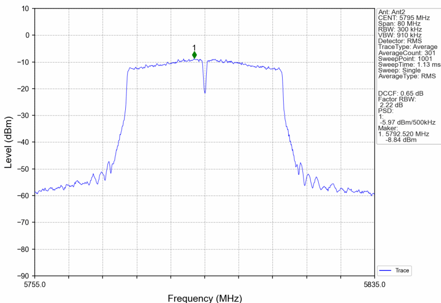
802.11ac(VHT40)_HCH_5795MHz_Ant2_NTNV
