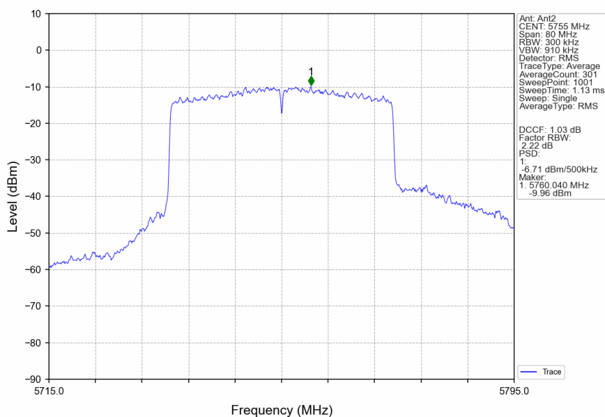
802.11ax(HEW40)_LCH_5755MHz_SU_ / _Ant2_NTNV
