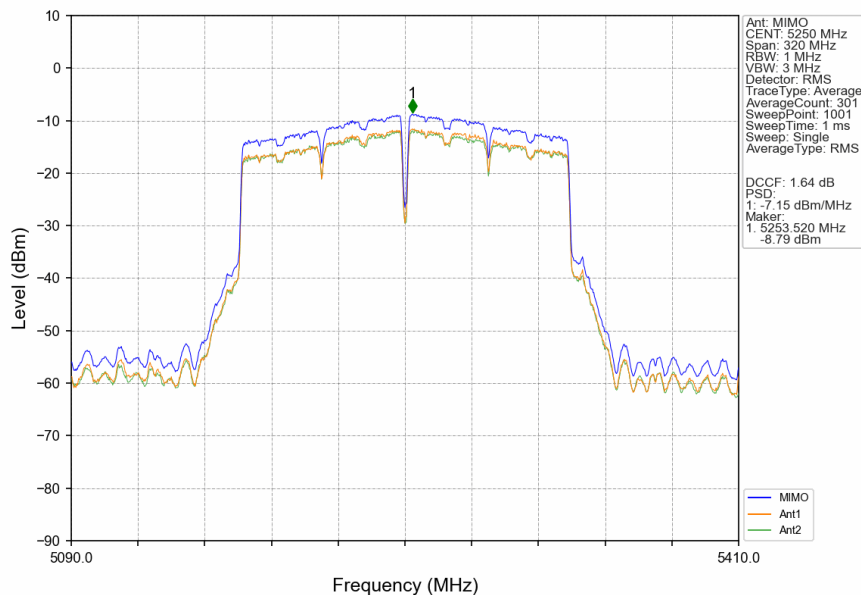
802.11ac(VHT160)_MCH_5250MHz_MIMO_NTNV
