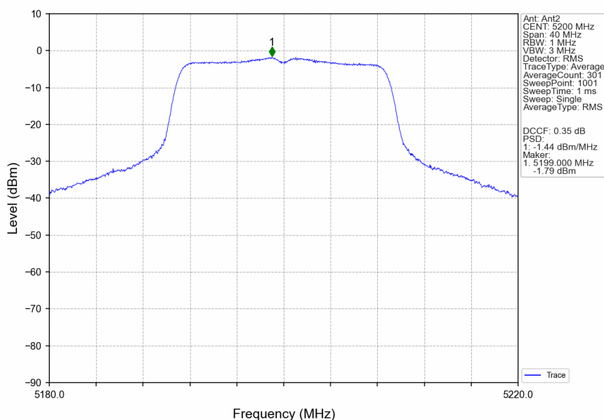
802.11ac(VHT20)_MCH_5200MHz_Ant2_NTNV
