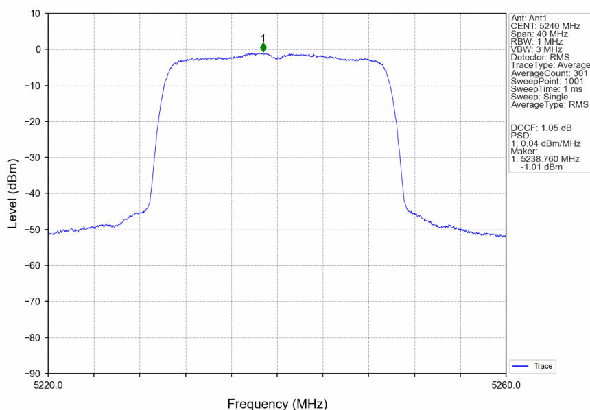
802.11ax(HEW20)_HCH_5240MHz_SU_ / _Ant1_NTNV
