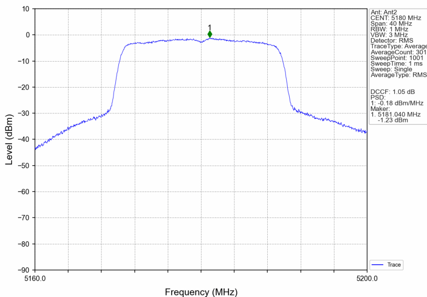
802.11ax(HEW20)_LCH_5180MHz_SU_ / _Ant2_NTNV
