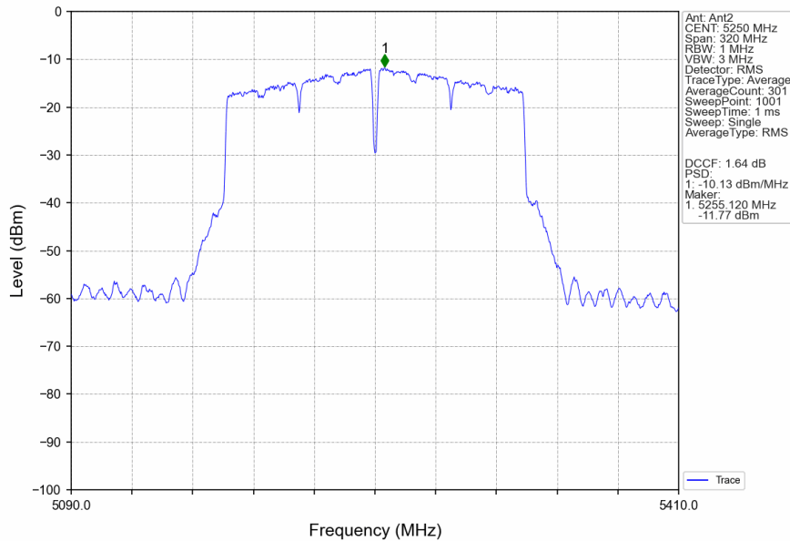
802.11ac(VHT160)_MCH_5250MHz_Ant2_NTNV
