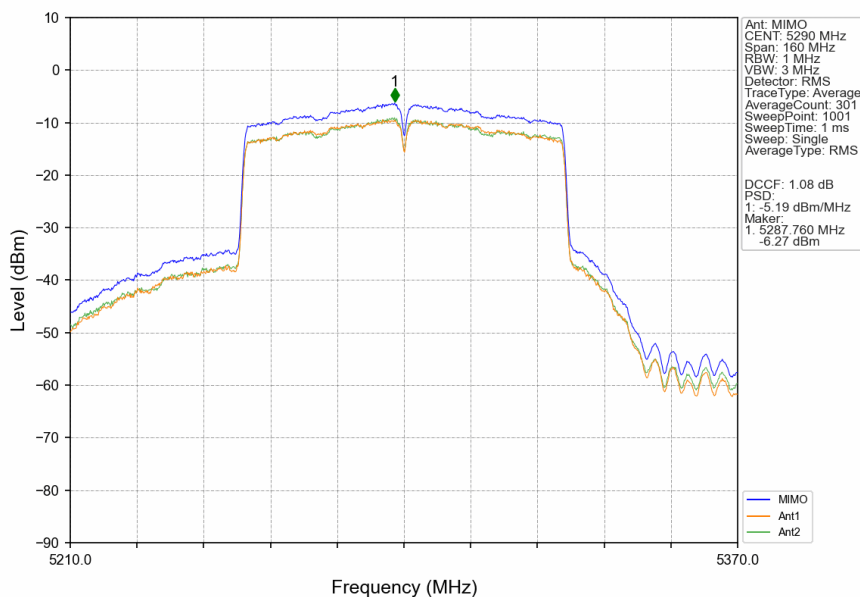
802.11ac(VHT80)_MCH_5290MHz_MIMO_NTNV
