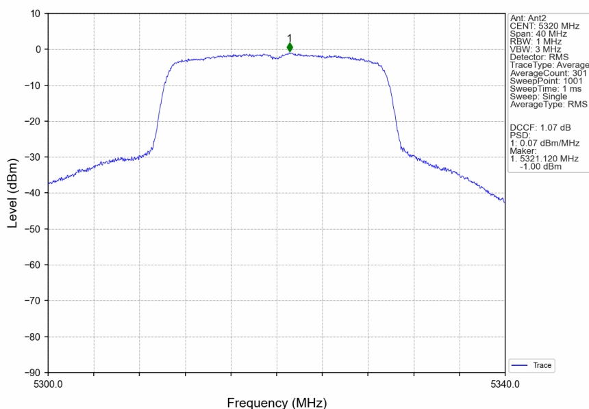
802.11ax(HEW20)_HCH_5320MHz_SU_/_Ant2_NTNV
