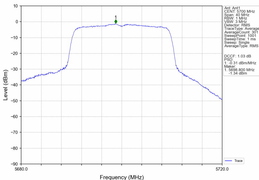
802.11ax(HEW20)_HCH_5700MHz_SU_/_Ant1_NTNV
