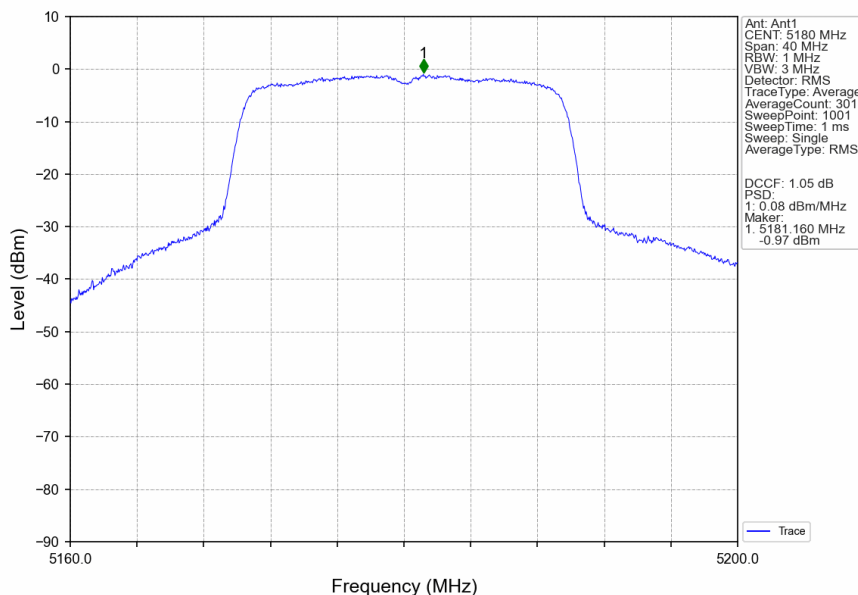
802.11ax(HEW20)_LCH_5180MHz_SU_ / _Ant1_NTNV
