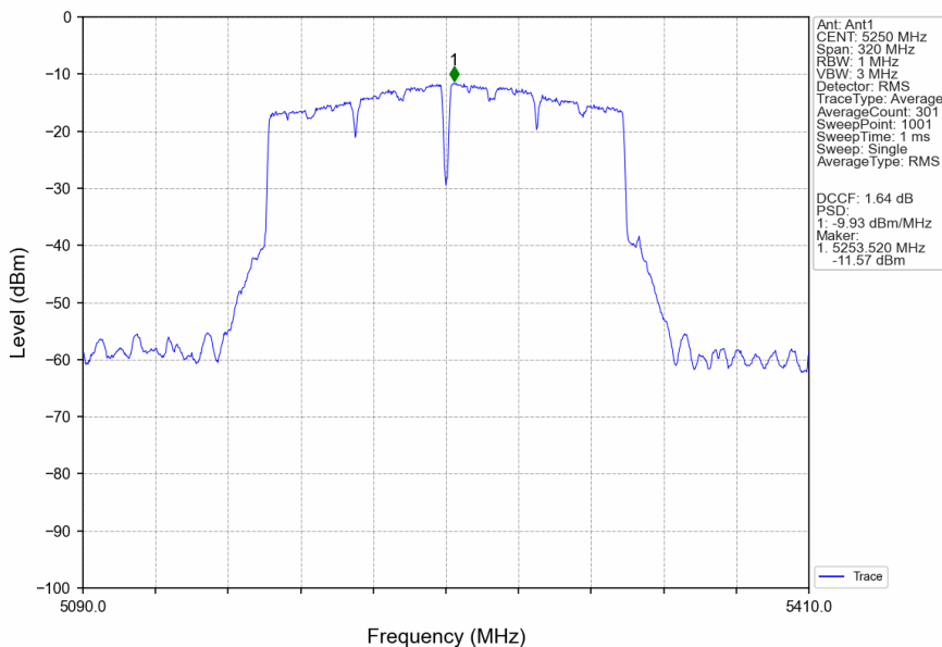
802.11ac(VHT160)_MCH_5250MHz_Ant1_NTNV
