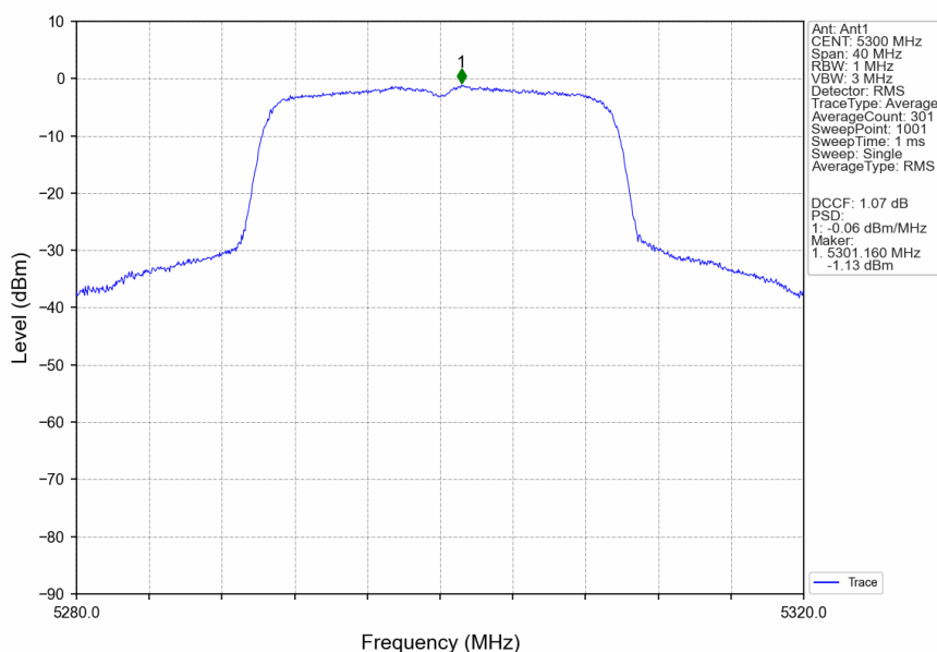
802.11ax(HEW20)_MCH_5300MHz_SU_ / _Ant1_NTNV
