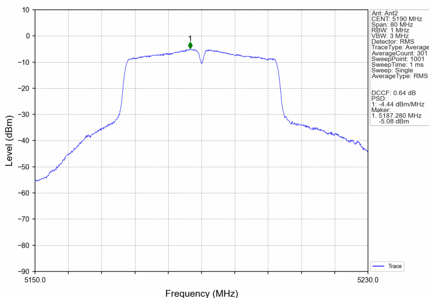
802.11ac(VHT40)_LCH_5190MHz_Ant2_NTNV
