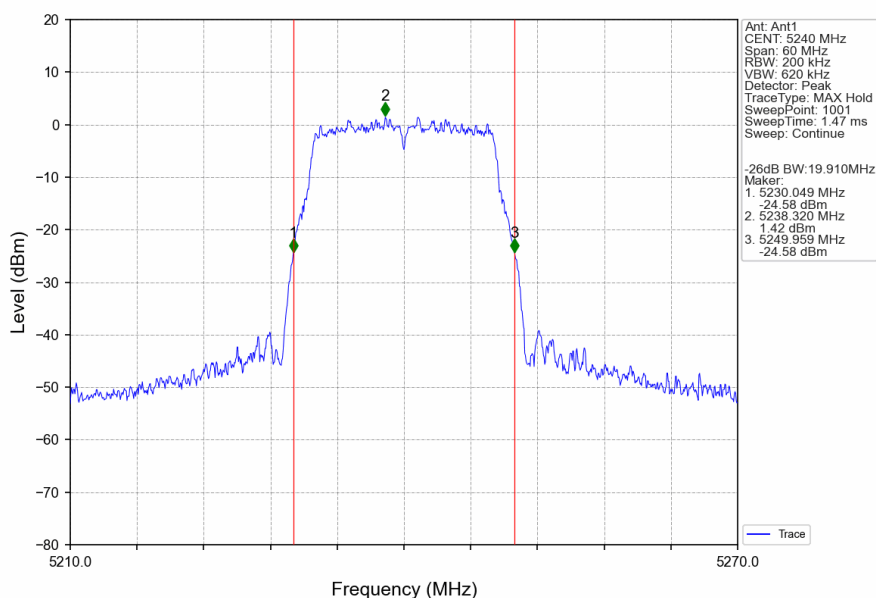
802.11a_HCH_5240MHz_Ant1_NTNV
