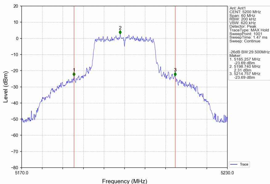
802.11n(HT20)_MCH_5200MHz_Ant1_NTNV
