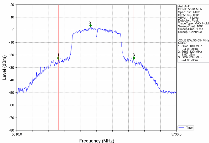
802.11n(HT40)_HCH_5670MHz_Ant1_NTNV
