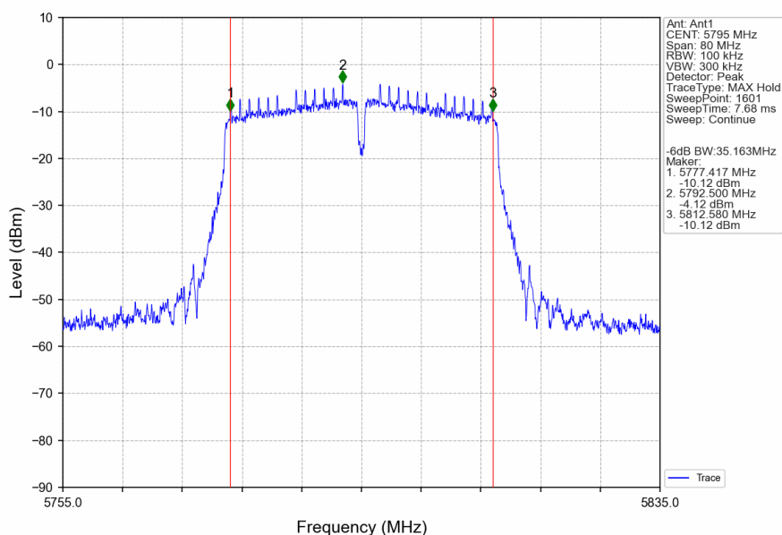
802.11ac(VHT40)_HCH_5795MHz_Ant1_NTNV
