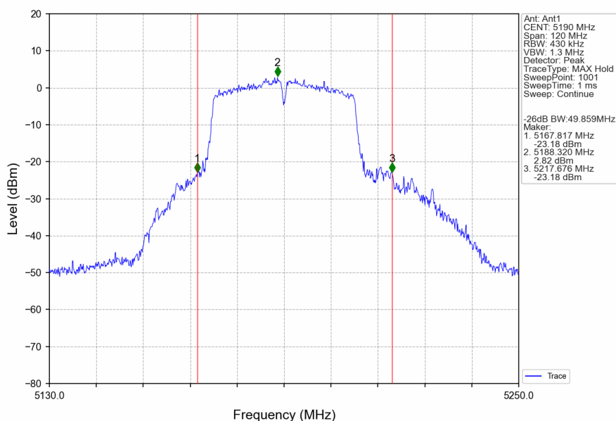
802.11ac(VHT40)_LCH_5190MHz_Ant1_NTNV
