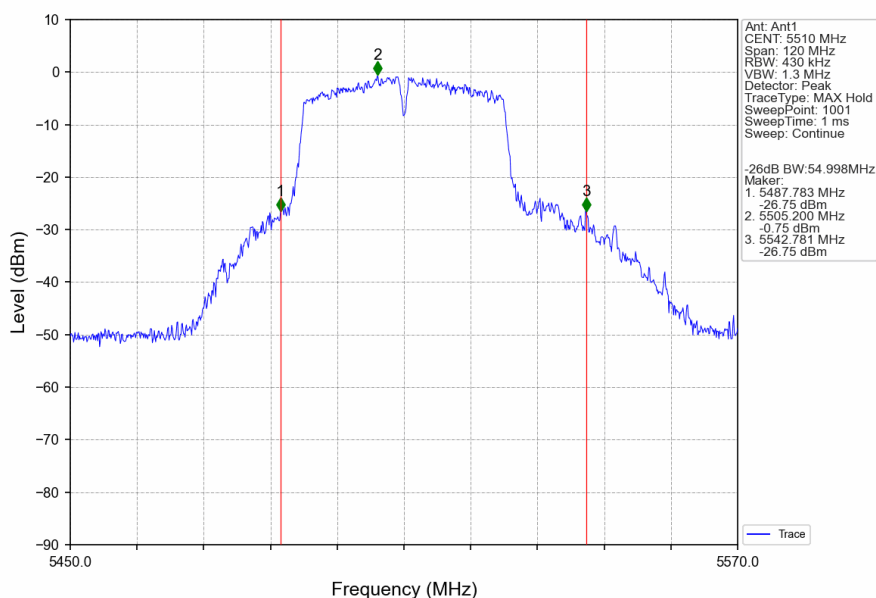
802.11ac(VHT40)_LCH_5510MHz_Ant1_NTNV
