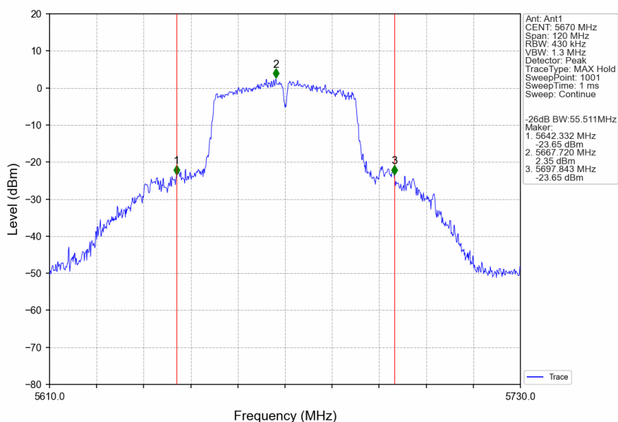
802.11ac(VHT40)_HCH_5670MHz_Ant1_NTNV
