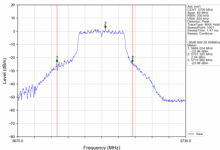
802.11a_HCH_5700MHz_Ant1_NTNV
