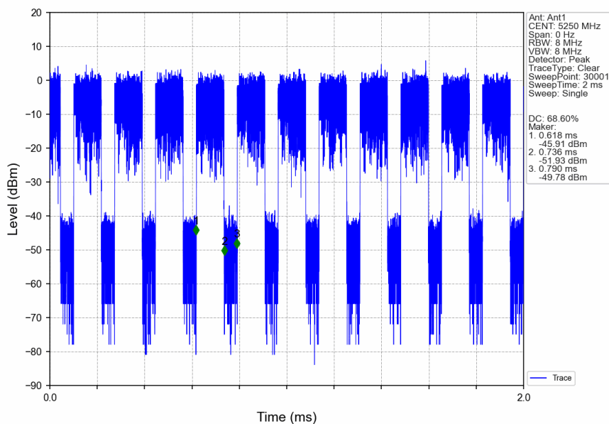
802.11ac(VHT160)_MCH_5250MHz_Ant1_NTNV
