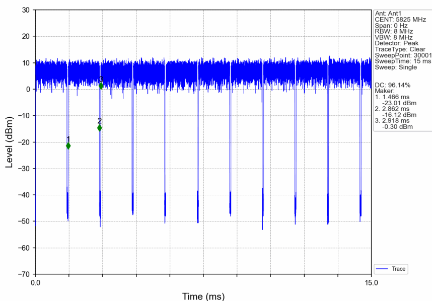
802.11a_HCH_5825MHz_Ant1_NTNV
