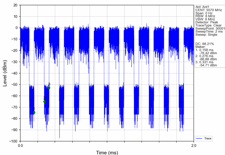
802.11ac(VHT160)_MCH_5570MHz_Ant1_NTNV
