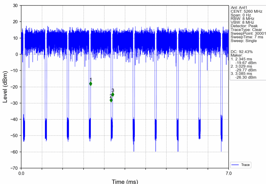
802.11ac(VHT20)_LCH_5260MHz_Ant1_NTNV
