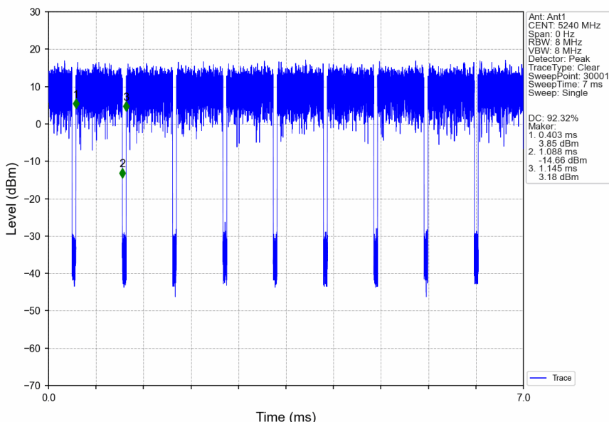
802.11ac(VHT20)_HCH_5240MHz_Ant1_NTNV
