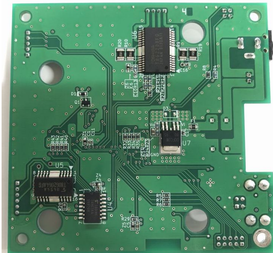
PCB (Bottom)
