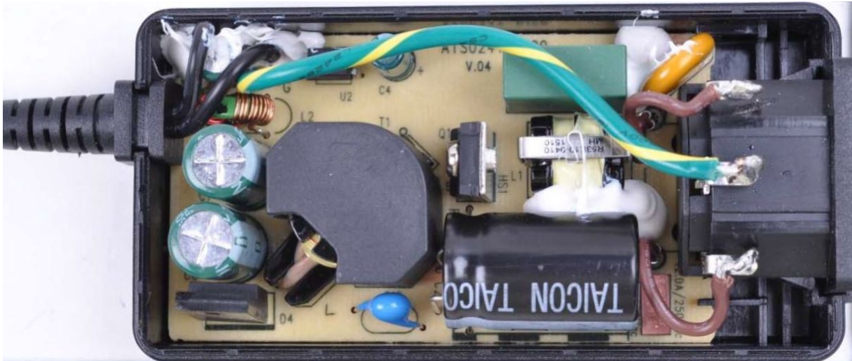
PCB inside the AC adaptor (Top)
