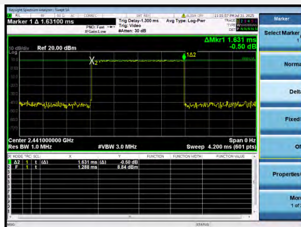
8-DPSK 3DH3
