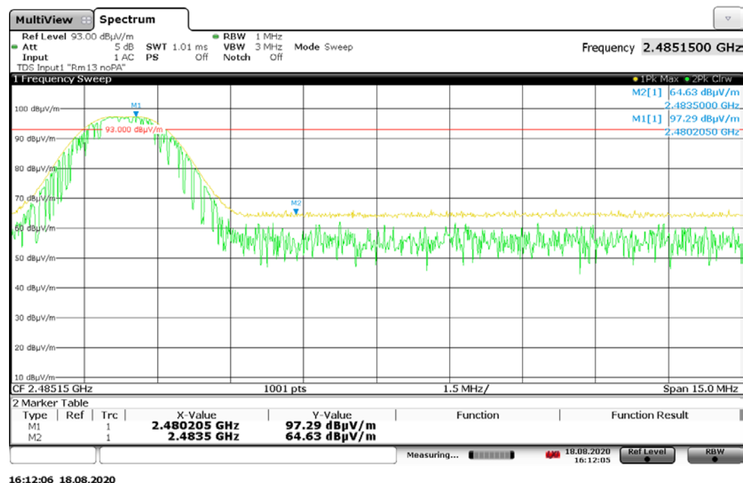
Graph 6-27: Upper Band edge (Restricted-band), 2480 MHz, Peak
