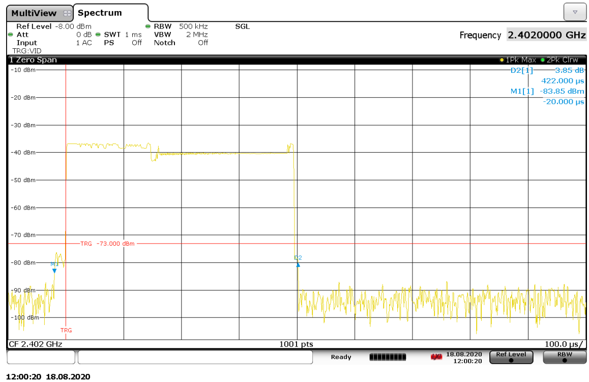
Graph 6-9: Duration of one pulse, 8-DPSK
