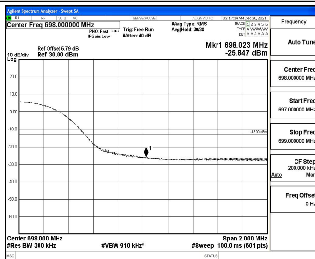
Band71-15MHz-16QAM-133197-75RB#0
