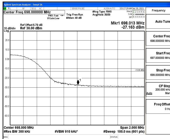
Band71-20MHz-QPSK-133222-100RB#0
