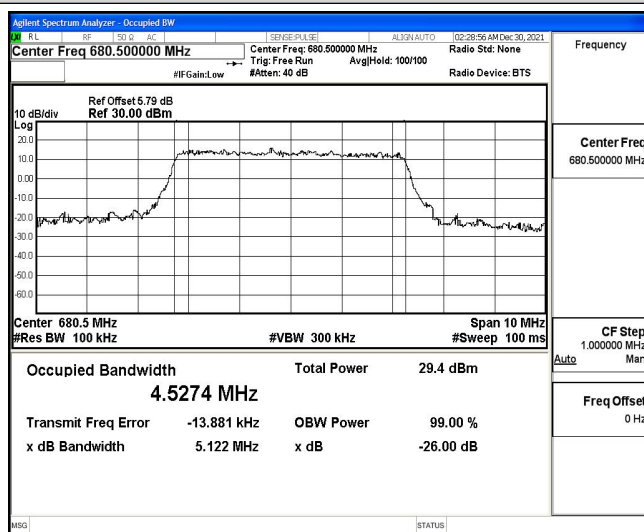
Band71-5MHz-16QAM-133447-25RB#0
