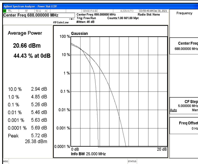
Band71-20MHz-16QAM-133372-100RB#0
