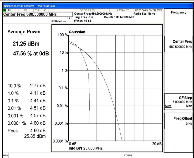
Band71-15MHz-16QAM-133297-75RB#0
