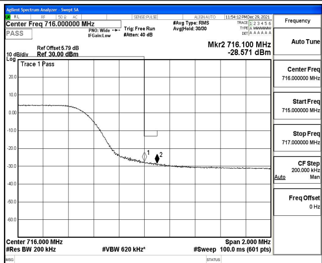
Band17-10MHz-16QAM-23780-50RB#0
