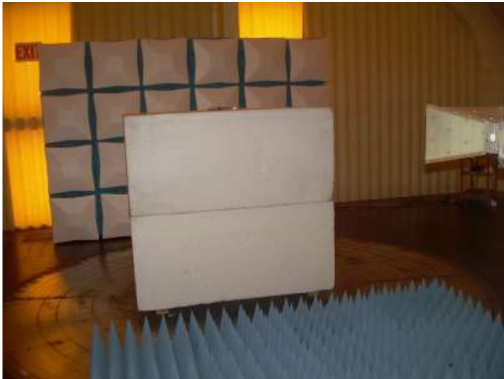
Photograph 3: Front View Radiated Emissions Battery Powered Flat– Above 1000 MHz Configuration
